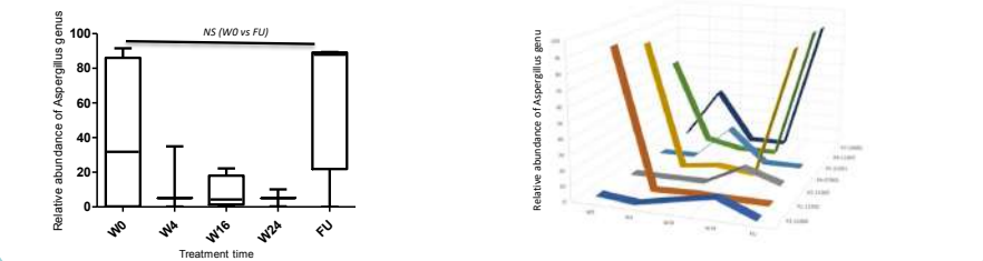
Figure 4. Evolution of the relative abundance of Aspergillus genus during treatment for each patient. (statistics : Wilcoxon test).
