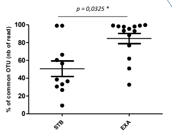
Figure 4: Proportion (%) of common fungal OTU (calculated in number of reads) between sputa and EDC in « stable sputa (STB) » (n=11) and « exacerbated sputa (EXA) » (n=14)
