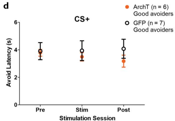
Figure 29. Optogenetic inhibition of the dmPFC-dl/IPAG pathway does not impair avoidance expression
