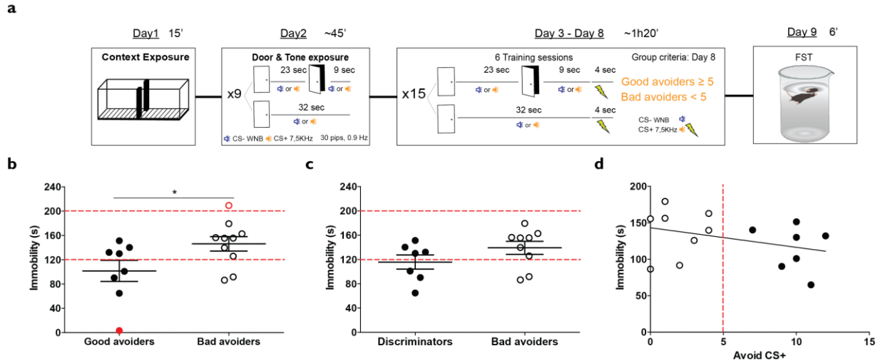
Figure 17. Bad and Good avoiders do not differ in the forced swim test
