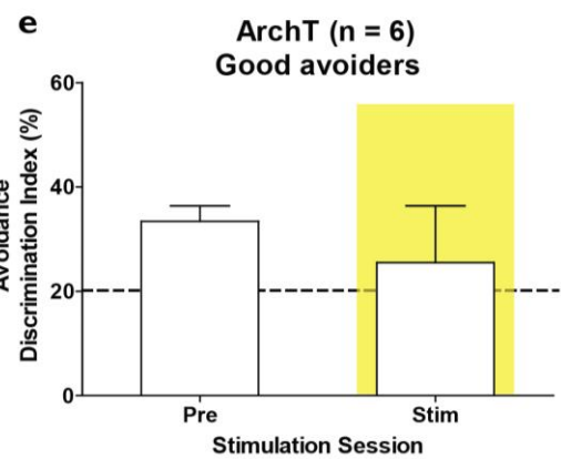
Figure 29. Optogenetic inhibition of the dmPFC-dl/IPAG pathway does not impair avoidance expression
