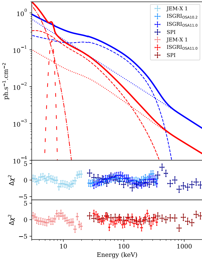
Fig. 5. Results of our (semi-)phenomenological fitting for LHS (blue) and HSS (red) with a Comptonisation model. The different model component are shown with different line styles: Comptonized continuum (dense-dashed), additional powerlaw (dotted), disk emission (dotted-dashed) and the iron line (loosely dashed). Bottom panels shows the residuals for both states.
