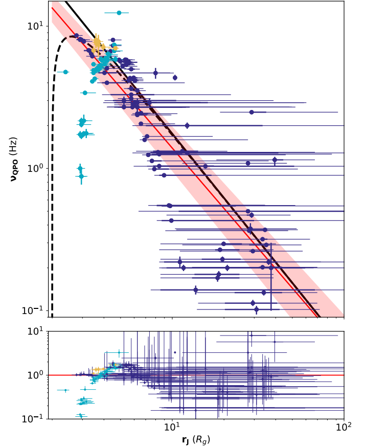
Fig. 7: Correlation between observed frequency \nu_{QPO} and the transition radius r_J (top) and the residuals defined as the ratio of the best weighted fit (red) to the data (bottom). Type A QPOs are shown in light yellow, Type B are indicated in cyan, Type C are shown in dark blue. The weighted linear fit considering only Type C LFQPOs, \nu_{QPO} = (36 \pm 6) \cdot r_J^{-1.41 \pm 0.08} , is indicated as a red line, the solid black line represents \nu_{QPO} = \nu_K(r_J)/100 , and the dashed black line represents \nu_{QPO} = \nu_{ep}(r_J)/100 .
