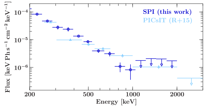
Fig. 3. Comparison of our extracted hard state INTEGRAL /SPI spectrum with INTEGRAL /IBIS/PICsIT spectra (a) extracted for the same time period as SPI and (b) for data before 2012 as published by Rodriguez et al. (2015).
