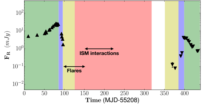
Fig. 2. Radio observations at 9 GHz during the 2010–2011 outburst of GX 339-4 (Corbel et al. 2013a,b). Steady jet emission is shown with triangle markers, upper for the rising phase and lower for the decaying phase, all corresponding to proper detections. Double arrows are drawn when radio emission was also observed but has been interpreted as radio flares or interactions with the interstellar medium (Corbel et al., in prep.). The vertical position of the arrows is arbitrary. The background color shades correspond to the X-ray spectral states (see Sect. 2.2). The epoch in white corresponds to a gap in the X-ray coverage due to solar constraints.
