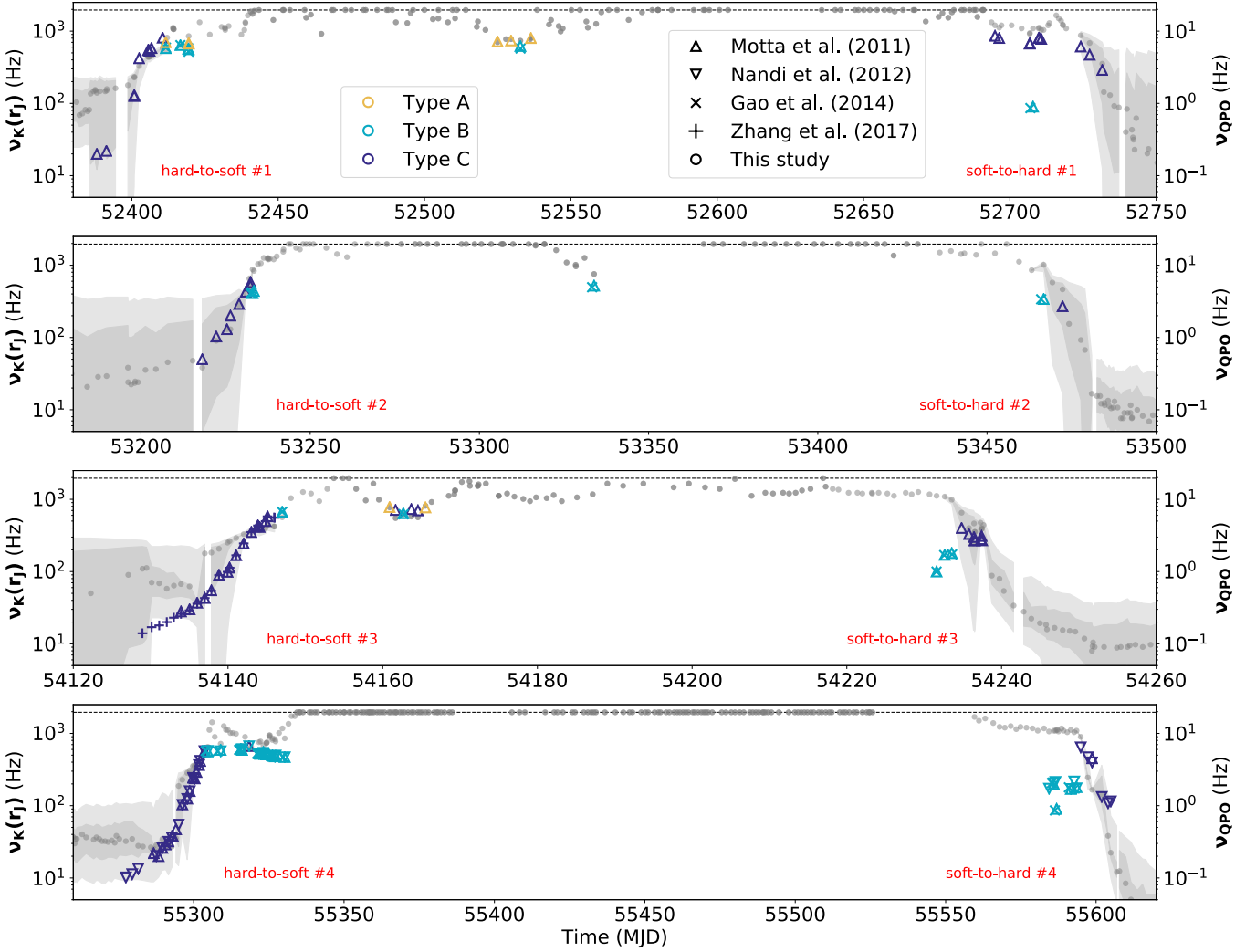
Fig. 5: Co-evolution of the observed QPO frequency \nu_{QPO} and the Kepler rotation frequency \nu_K(r_J) for the 4 different outbursts, showing both hard-to-soft and soft-to-hard transitions (see red annotations). The left y-axis shows the Kepler frequency at the transition radius, \nu_K(r_J) , and the 5% and 10% confidence intervals. The right Y-axis shows the observed QPO frequency, \nu_{QPO} . Different markers are used to distinguish the different works: Motta et al. (2011) is indicated in upward triangles, Nandi et al. (2012) is indicated in downward triangles, Gao et al. (2014) is indicated in crosses, Zhang et al. (2017) is shown in plus signs, and new detections are shown in circles (see text). Different colors indicate the different types of QPOs (see legend).
