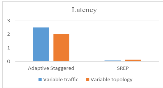
Figure 51: Latency comparison
