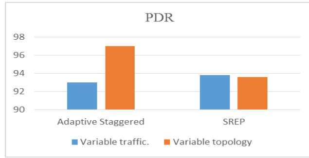
Figure 50: PDR comparison
