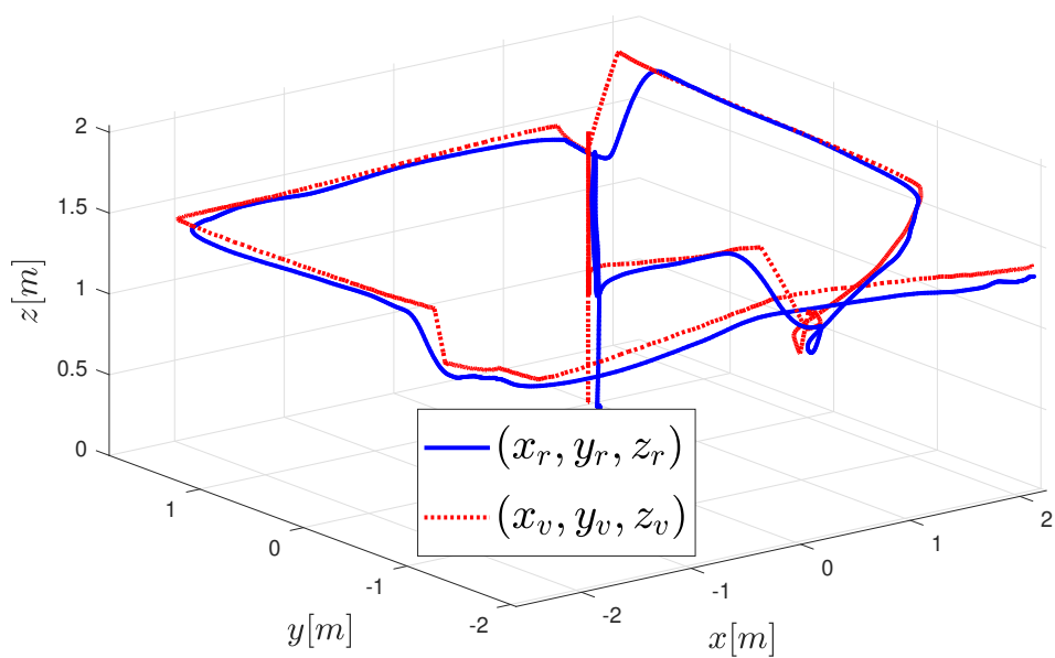
Figure 3.13 – 3D-position performance trajectory given by the user and imitated by the real drone.
