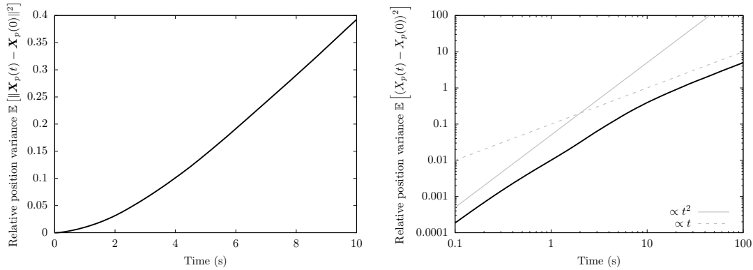
Figure 9.6. Time evolution of the sample variance of particle relative positions under the EMEF, with linear (left) or log (right) scales. Relative variance of one physical particle position on 240 sub-grids, averaged over 240 large eddies. The sub-grid amounts for 20% of the total fluid energy. Particle relaxation time scale of 1s. Initial particle velocity set to fluid velocity.
