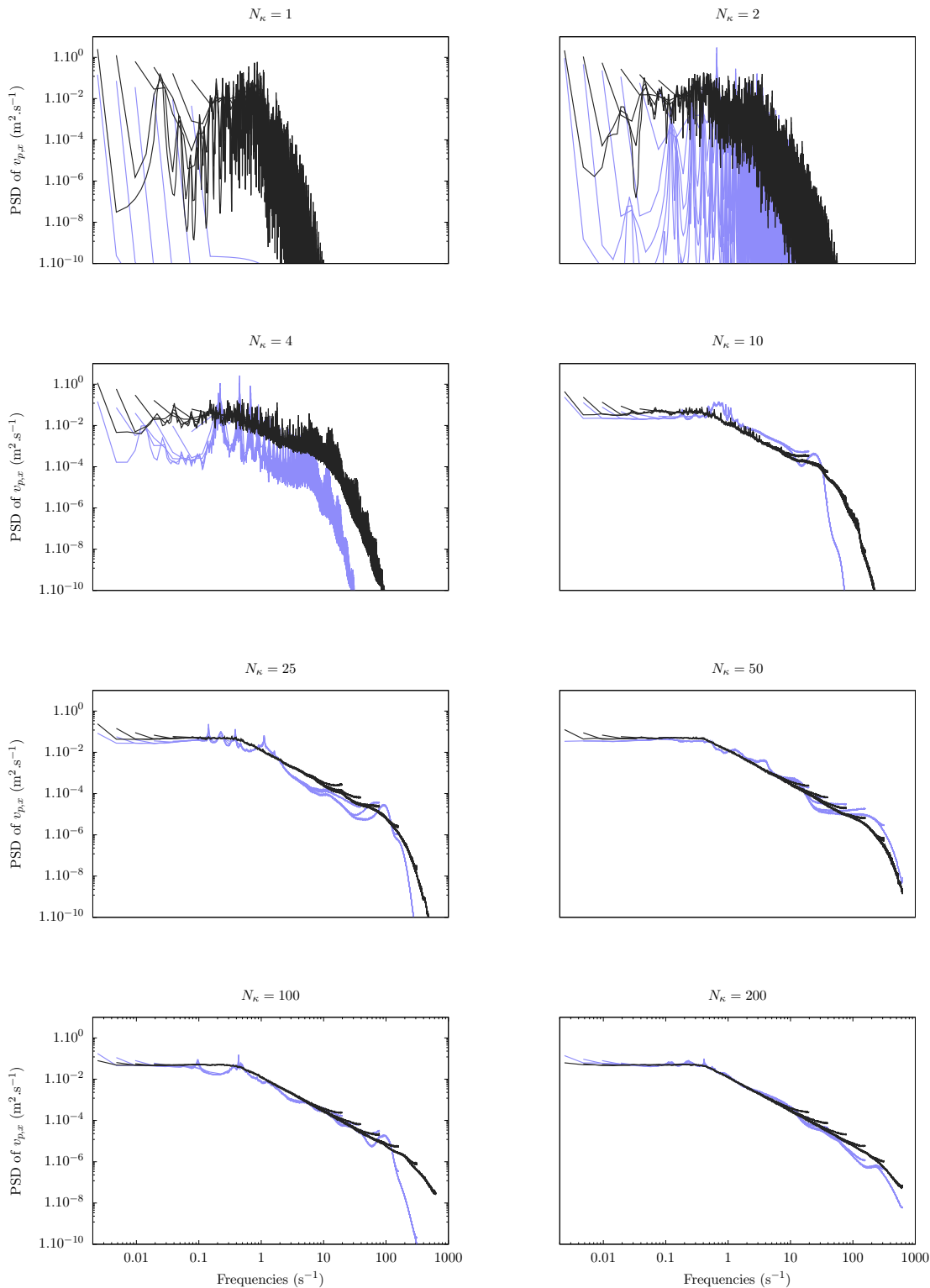
Figure 7.4. Influence of the number of fluid modes (indicated above each graph \{1,4,10,25,50,100,200\} ) on the power spectral density of the velocity of a fluid parcels along its trajectory on a fluid of energy 1\text{m}^2.\text{s}^{-2} wave-number range between 1\text{m}^{-1} and 10^4\text{m}^{-1} averaged 10 times. In black lines, a particle on 240 different fluids. In blue lines, PSD of 240 particles on one fluid realization. Graph shows the superposition of 6 PSD of 2^{14} points with Hann windowing of different resolutions in order to get a visualisation of a wide spectrum range. Trajectories computed with RK4 integration and a time step of 8.10^{-4}\text{s} .
