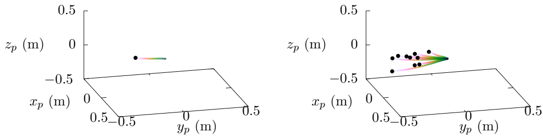
Figure 5.2. The beginning of the trajectory of one inertial particle ( \tau_p = 1\text{s} ) on one fluid on the left and on ten different fluids conditioned by 80% of their energy (synthetic fluids, presented in Sec. 6.1, of 200 modes, meaning that the 160 lowest wave-numbers modes are constants across fluids) on the right. The initial particle velocity is taken as the fluid velocity at the particle position.
