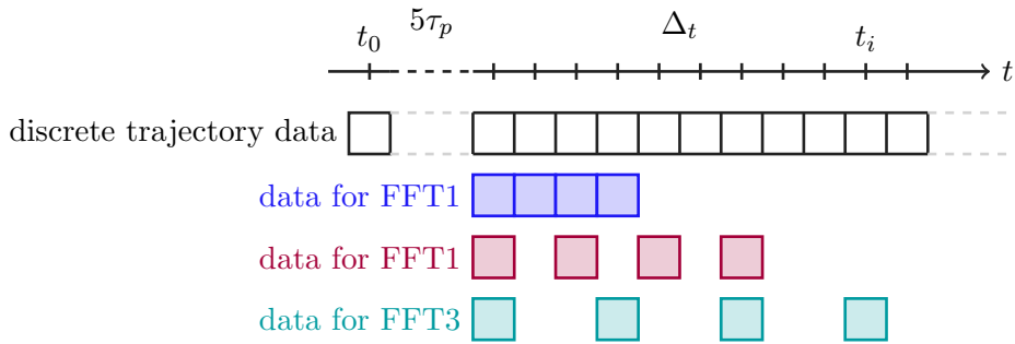
Figure 6.5. Chosen strategy for computing the discrete Fourier transform of a signal over a wide range of scales at a reasonable cost.
