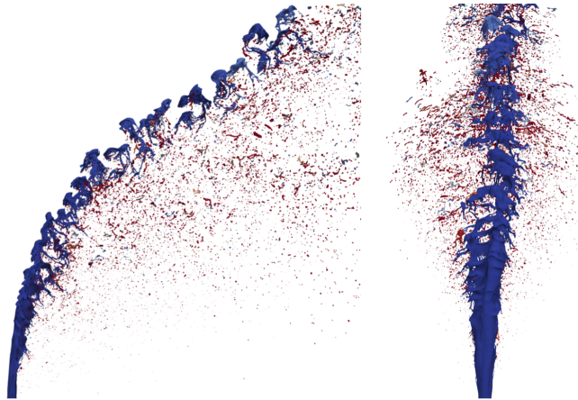
Figure 6. Simulation of a liquid jet in a crossflow simulated with the YALES2 solver (Leparoux, Mercier, Moureau, and Musaefendic (2018)).
