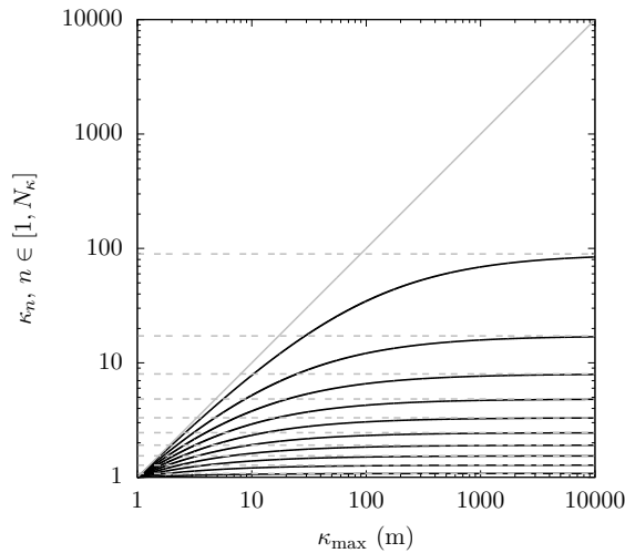
Figure 7.1. Influence of the range of fluid wave-numbers on the modes (here for 10 modes). Asymptotes are represented in dotted lines, and the first bisector with a lighter shade.
