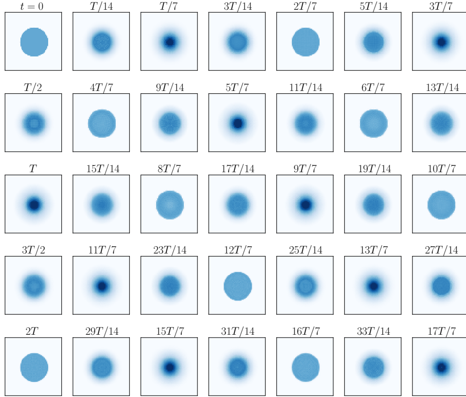
Figure 9.9: Numerical simulation with an initially uniform disk-shaped cloud, for the parameters N_s = 512 and \alpha = 4 . The initial wave function is the ground state of a disk-shaped box-potential. The images show the density distribution of this wave function during an evolution according to the full Gross-Pitaevskii equation. The same density distribution seems to appear every 2T/7 .
