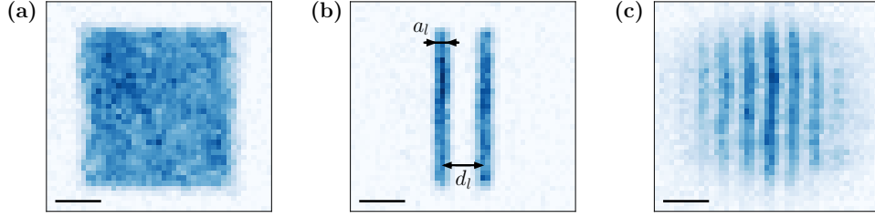
Figure 6.1: Experimental procedure. (a) The gas is prepared in a square of side 40\text{ }\mu\text{m} and its ratio T/T_c is controlled and can be measured independently. (b): All the atoms are transferred to the state F = 2, m_F = 0 with a microwave pulse. A controlled fraction of the atoms contained in the region of two lines is transferred back to the state F = 1, m_F = 0 with the Raman beams. We send a beam resonant with the transition F = 2 \rightarrow F' = 3 on the sample, and the atoms that have stayed in the state F = 2 are expelled from the trap. The picture shows the two lines that we isolate with this method. Their expected full-width is a_l and the distance between their centre is d_l . (c): The two lines expand and interfere. On all the images, the solid black line corresponds to 10\text{ }\mu\text{m} .
