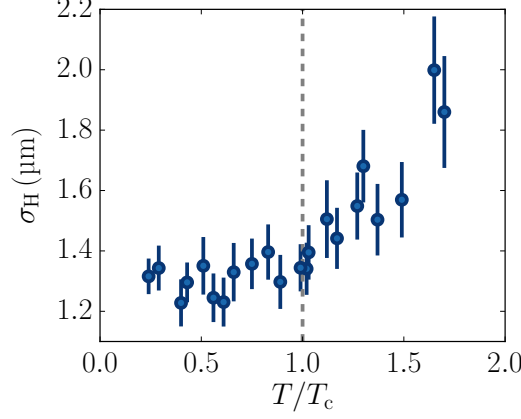
Figure 5.6: Half width at half-maximum \sigma_H of the momentum distribution of the cloud as a function of the ratio T/T_c . This width stays around 1.3\,\mu\text{m} when T < T_c . When the temperature is increased above T_c , the momentum distribution gets wider, with a HWHM as high as 2\,\mu\text{m} .
