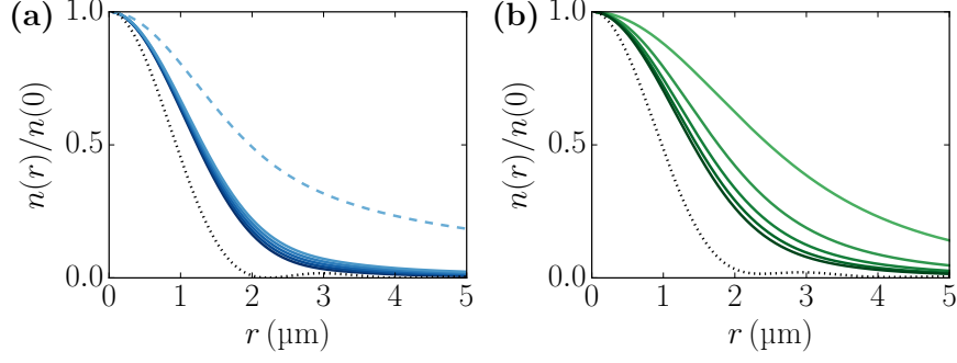
Figure 5.7: Numerical computations of the momentum distribution measurement using our experimental method from equation 5.19 and for a disk of radius 20\text{ }\mu\text{m} . (a): The correlation function is a power law r^{-\eta} for \eta = 0.05, 0.1, 0.15, 0.2 and 0.25 from dark blue to light blue, solid lines. The five curves are very close to one another. The dashed line is the result we obtain with \eta = 1 , which is not in the range theoretically allowed. The dotted black line is the momentum distribution we would measure when \eta = 0 and a perfect optical resolution. (b): The correlation function is an exponential decay \exp(-r/\ell) with \ell = 5, 10, 15, 20, 25\text{ }\mu\text{m} from light green to dark green. A correlation function with a short range gives a broad momentum distribution. The dotted black line is the momentum distribution we would measure when \ell = 100 and a perfect optical resolution.
