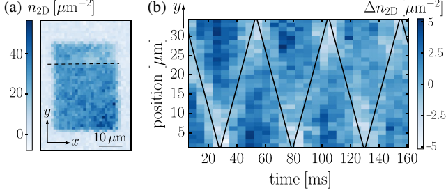
FIG. 1. Experimental protocol and observation of propagating waves. (a) Absorption image of the cloud perturbed by a local additional potential. The excitation is delimited by the horizontal dashed line and depletes the atomic density by a factor around 1/3 . (b) Example of time evolution of the variation of the density profile n_{2D} with respect to its spatial mean value (integrated along x ) obtained after abruptly removing the additional potential. For this example T/T_c = 0.37(12) and n_{2D} = 29(3) \mu\text{m}^{-2} . The position of the dip is fitted by a triangle function (black solid line) which gives, c = 1.49(3) \text{ mm/s} .
