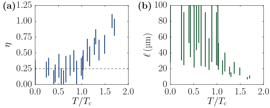
Figure 5.9: Comparison between the experimental data presented on Fig. 5.6 and the computations summarized on Figs. 5.7 and 5.8. (a): For each experimental point, assuming that the correlation function is a power law, the range of exponents \eta that are compatible with the measurement is indicated as a vertical bar. (b): For each experimental point, assuming that the correlation function is an exponential, the range of characteristic lengths \ell that are compatible with the measurement is indicated as a vertical bar.
