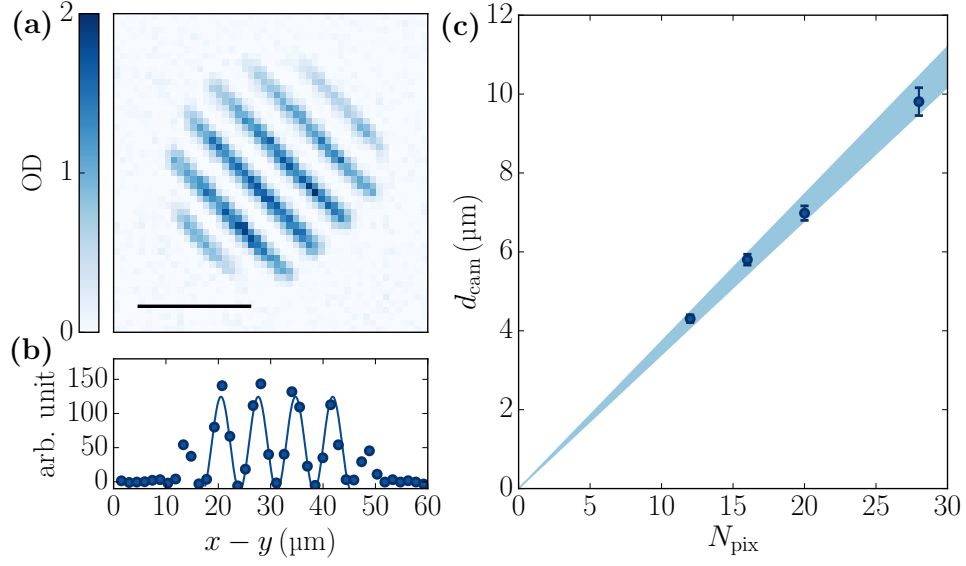
Figure 3.6: Calibration of the effective size of the DMD . (a): A striped pattern with an integer number of DMD pixels is shone on the atoms. We measure the density distribution of transferred atoms by averaging five experimental realisations. On the image shown here, the periodicity of the pattern is N_{\text{pix}} = 20 . The horizontal black line represents 20 \mu\text{m} . (b): This distribution is summed along the axis of the stripes, and the obtained signal is fitted with a sine function. The fitted periodicity is here d_{\text{cam}} = 7.0(2) \mu\text{m} . (c): The periodicity d_{\text{cam}} as a function of N_{\text{pix}} is plotted and fitted with a linear function. The slope is 0.36(1) \mu\text{m} .
