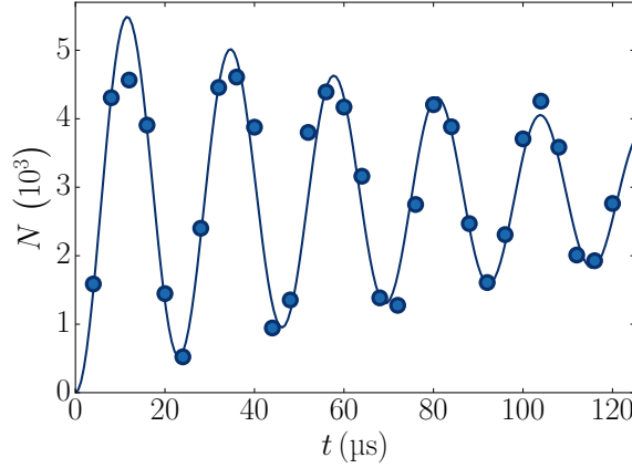
Figure 3.4: A Rabi oscillation with the Raman beams. A small cloud of radius 5\text{ }\mu\text{m} in the F = 1, m_F = 0 state is illuminated during a time t with the Raman beams. The number of atoms transferred in F = 2, m_F = 0 is measured. The results are fitted with an exponentially attenuated squared sine function. The fitted Rabi frequency is \Omega_R = 2\pi \cdot 21.7(2)\text{ kHz} , and the decay time of the amplitude is \gamma^{-1} = 110(10)\text{ }\mu\text{s} .
