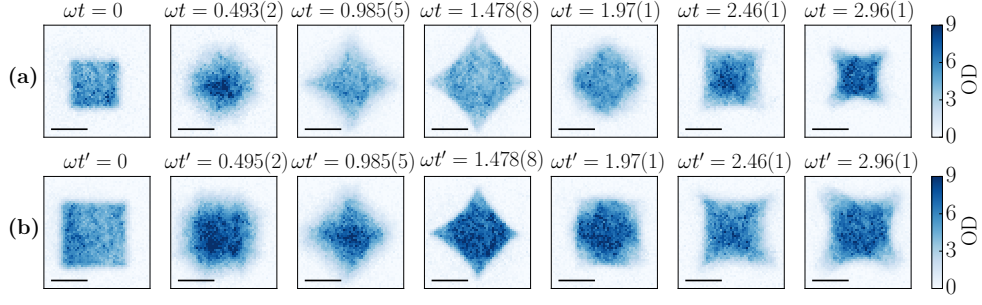
Figure 8.9: Evolution of two initially uniform square-shaped clouds with a different initial size and a different atom number. (a): Evolution in a harmonic potential during the first half period of a cloud of N_1 = 3.7(3) \cdot 10^4 atoms initially in a square-shaped box potential of side L_1 = 27.0(5) \mu\text{m} . (b): Evolution in the same harmonic potential during the first half period of a cloud of N_2 = 5.4(3) \cdot 10^4 atoms initially in a square-shaped box potential of side L_1 = 36.8(5) \mu\text{m} .
