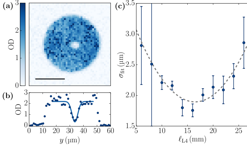
Figure 3.5: Focusing the DMD of the Raman beams on the atoms. (a): We transfer the atoms with the Raman beams to the F = 2, m_F = 0 state uniformly, except on a small region selected with the DMD . The image is the average of two experimental realisations. The horizontal black line represents 20 \mu\text{m} . (b): The density profile of this region is fitted with a 1D inverted Gaussian shape and the size along the y -direction \sigma_{\text{fit}} is extracted. On this example, \sigma_{\text{fit}} = 1.8(1) \mu\text{m} . (c): We plot \sigma_{\text{fit}} as a function of the position \ell_{L4} of lens L4. The position where a minimum is reached is where the DMD is on focus. With a parabolic fit of the data points we determine that this focus is at \ell_{L4} = 16.5(5) \text{ mm} . The origin of this axis is arbitrary, and the important quantity to extract from the fit is the ratio between the error bar of this minimum and the focal length of the lens, here 400 \text{ mm} .
