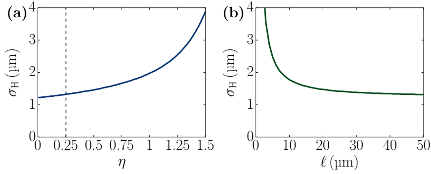
Figure 5.8: Half width at half-maximum \sigma_H of the computed momentum distributions for a disk of radius 20\mu\text{m} . (a): The function g_1^\infty is modelled by a power law of exponent \eta . The graph shows the width of the obtained momentum distribution as a function of \eta . The interesting region for the BKT transition is for 0 \leq \eta \leq 0.25 , delimited by the dashed grey line. (b): The function g_1^\infty is modelled by an exponential with characteristic length \ell . The graph shows the width of the obtained momentum distribution as a function of \ell .
