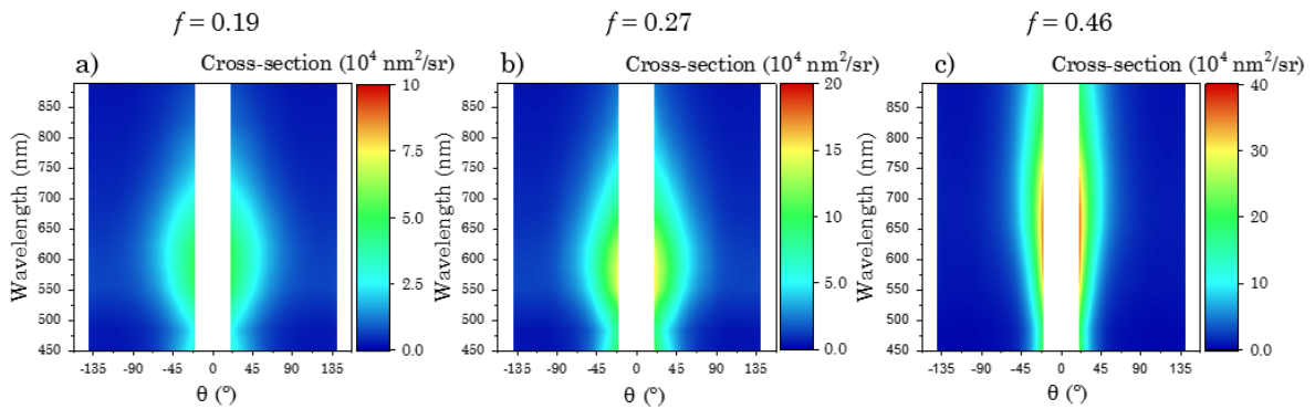
Figure 4.9: Experimental scattering patterns: values of the differential scattering cross-sections ( \sigma_{\text{cluster}} ) as a function of the wavelength \lambda and the scattering angle \theta , for cluster samples a) PEG-6000-2 (gold volume fraction estimated at f \approx 0.19 ), b) PEG-2000-2 ( f \approx 0.27 ) and c) PEG-800-4 ( f \approx 0.46 ). We measured only for \theta > 0 , but assumed that \sigma_V(\lambda, -\theta) + \sigma_H(\lambda, -\theta) = \sigma_V(\lambda, \theta) + \sigma_H(\lambda, \theta) . Note that the \text{nm}^2/\text{steradian} color scale is enhanced by a factor 2 going from (a) to (b) and by 2 again from (b) to (c).
