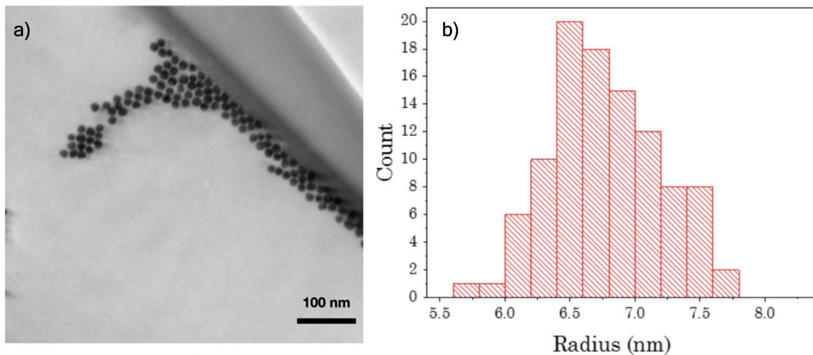
Figure 2.14: a) TEM image of the synthesized gold NPs. b) Size distribution of gold NPs estimated from TEM images.
