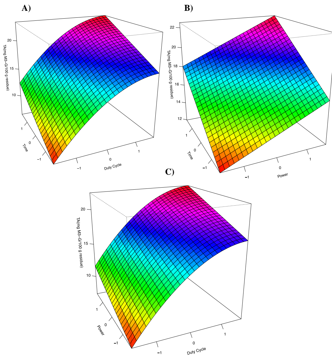
Figure V-2. Response surface plots of the predicted model of time – duty cycle (A), time – power (B) and power - duty cycle (C) for total anthocyanin extraction from grape pomace by UAE. The third independent factor was set at 0 (coded value) to plot the response surfaces
