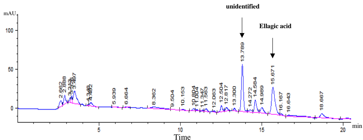
Figure IV-5. High performance liquid chromatogram of a polyphenol-rich extract obtained from defatted walnut cake by UAE
