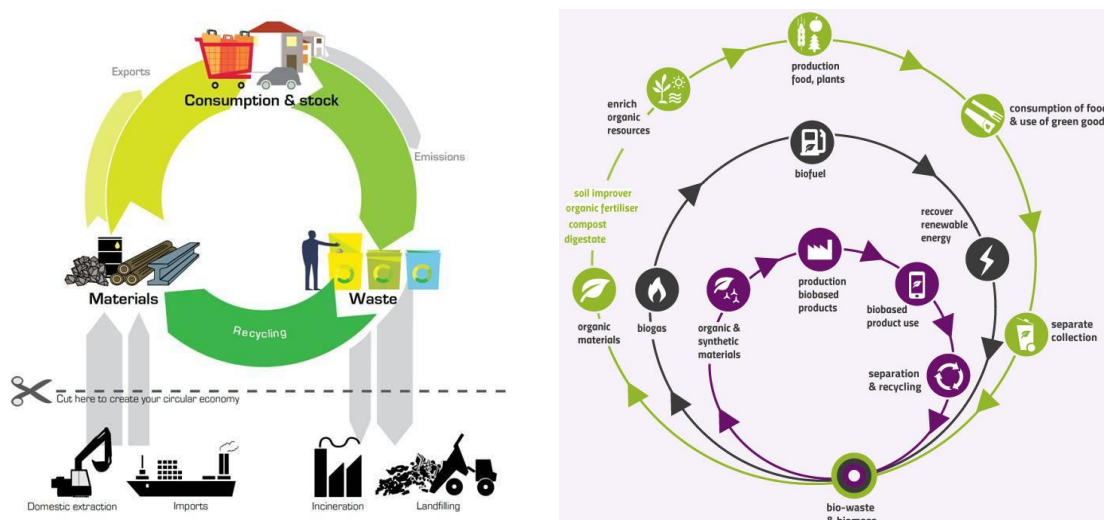
Figure I-4. Schematic representation of the circular economy approach (adapted from European Compost Network)
