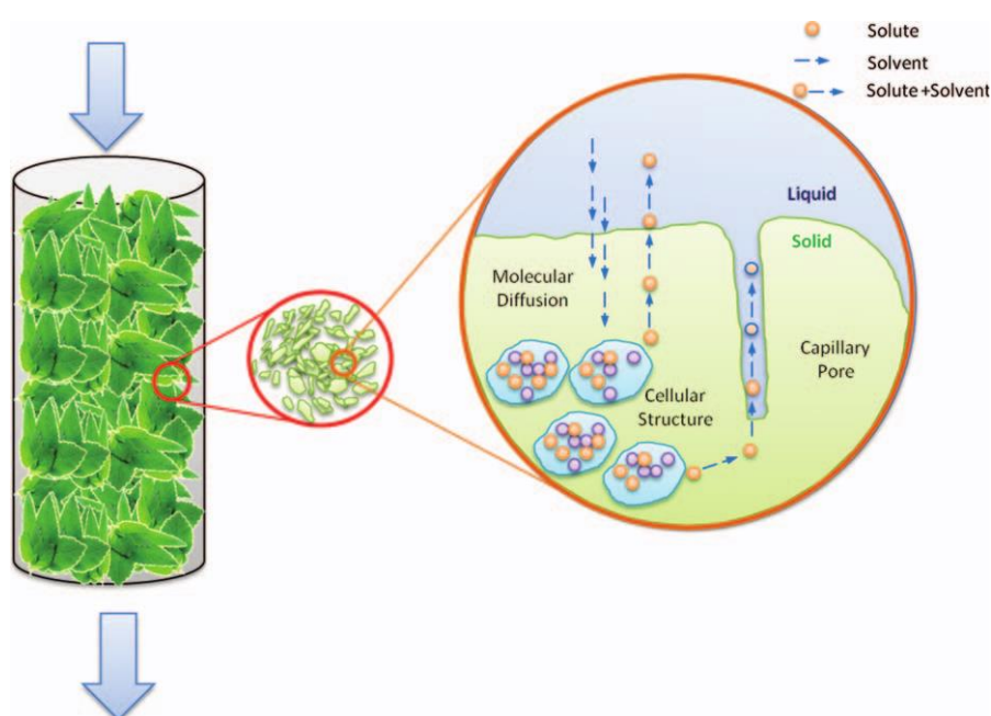
Figure I-11. Schematic representation of the extraction mechanism from plant matrices (Source Palma et al., 2013)
