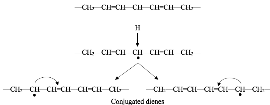
Figure I-10. Formation of conjugated dienes as primary products of lipid oxidation (Source: Dridi, 2016)
