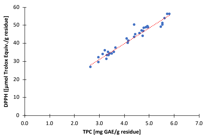
Figure V-A1. Correlation between TPC and antiradical activity of grape pomace extracts obtained by UAE
