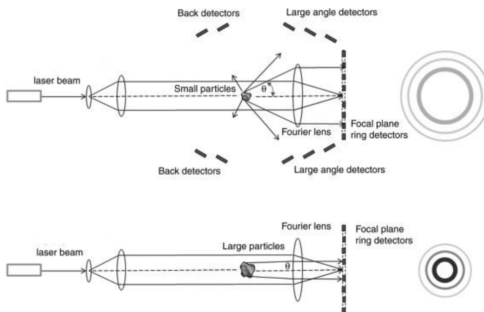
Figure II-11. Light scattering angles of small and large particles
