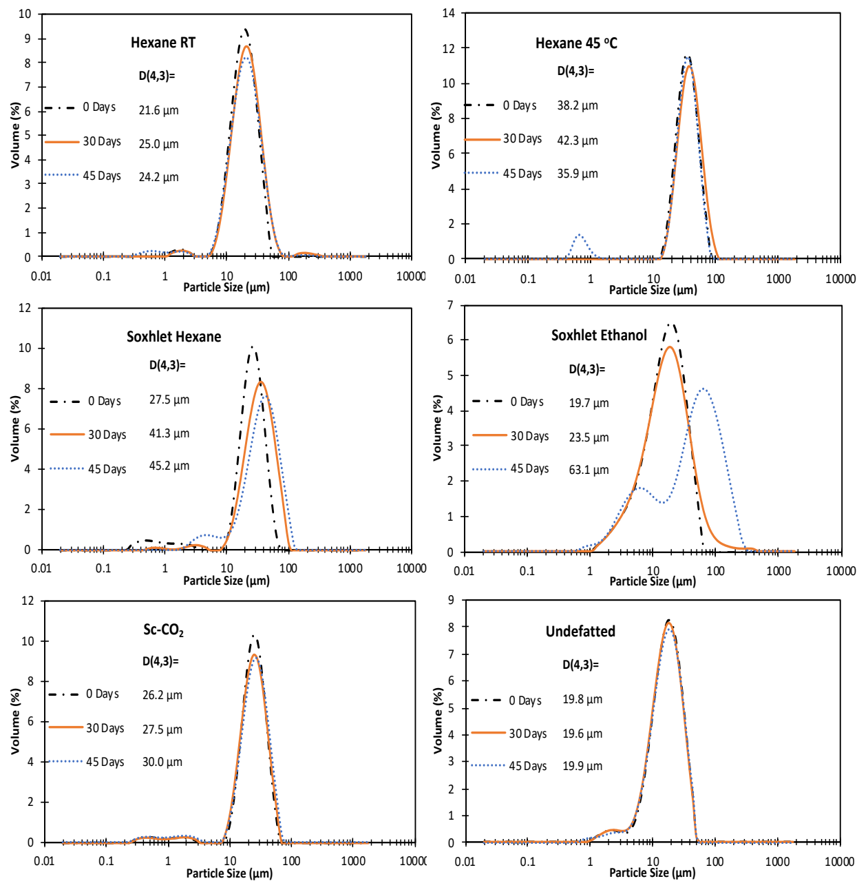
Figure III-10. Droplet size distributions of emulsions prepared with different corn germ protein extracts, after different storage durations at 4 °C
