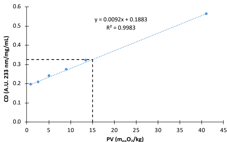
Figure IV-13. Correlation between peroxide value and the formation of CD during oxidation of virgin linseed oil at 60 °C
