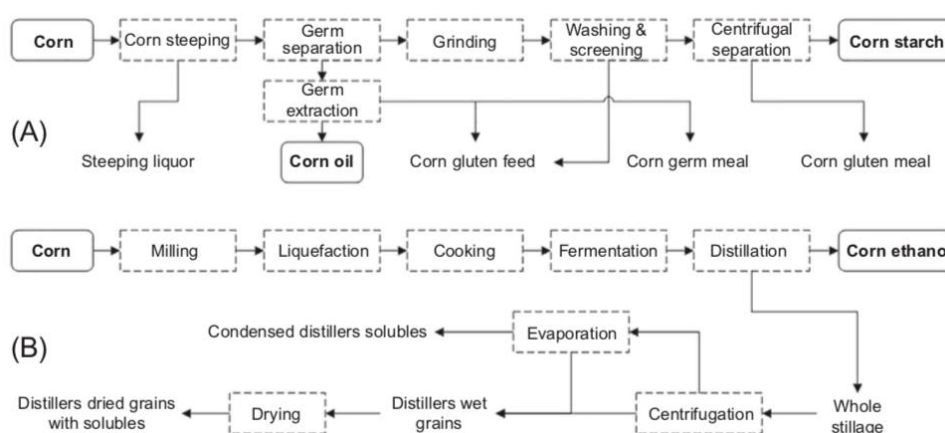
Figure III-3. Processing of corn by wet milling (A) and dry milling (B)
