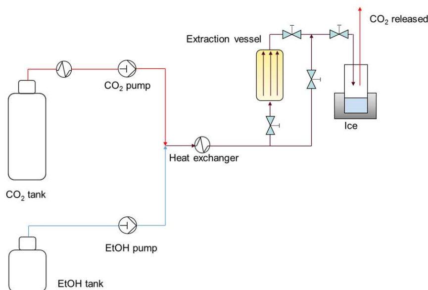
Figure II-6. SFE set -up (Adapted from: Bardeau et al., 2015)
