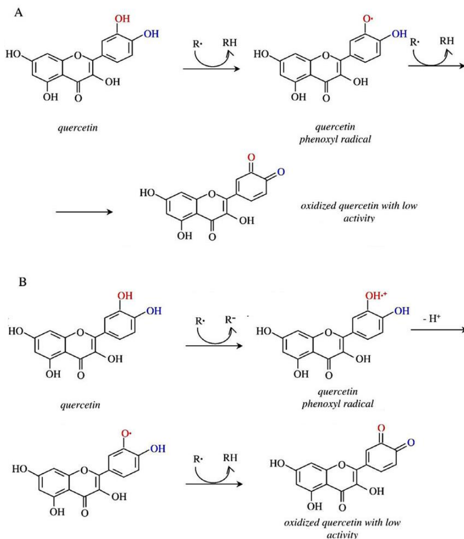
Figure I-6. Mechanisms for free radical scavenging activity of polyphenols (quercetin) by (A) hydrogen atom donation or (B) electron transfer—proton transfer (Source: Papuc et al., 2017)
