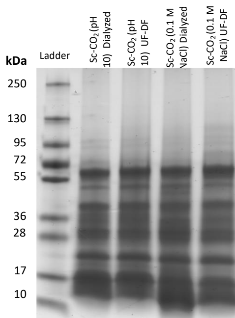
Figure III-14. SDS-PAGE profiles of proteins extracted from Sc-CO 2 defatted meal by means of various protein extraction methods (saline or alkaline) and purification methods (dialyzing or UF-DF)
