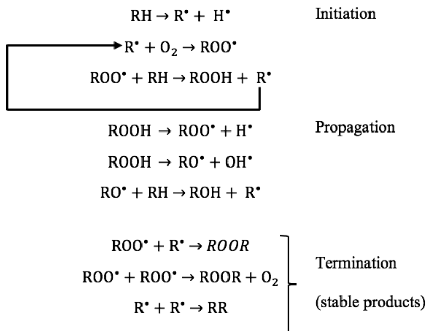
Figure I-9. Schematic representation of peroxidation of lipids
