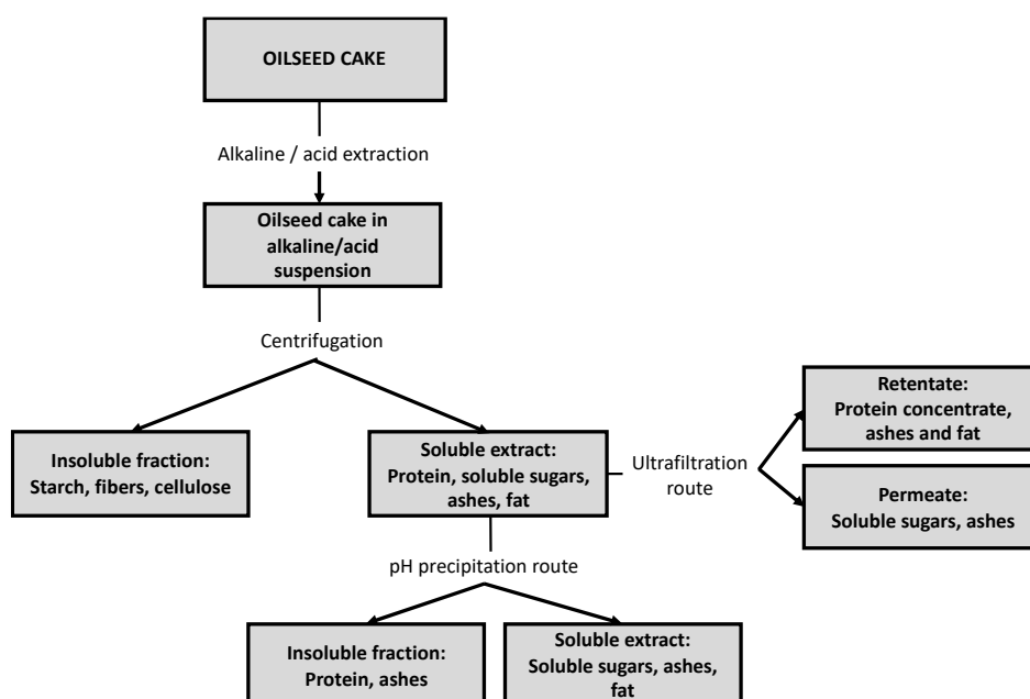
Figure I-12. Industrial scale extraction and isolation of vegetable protein by solid-liquid method (Adapted from Chéreau et al., 2016)
