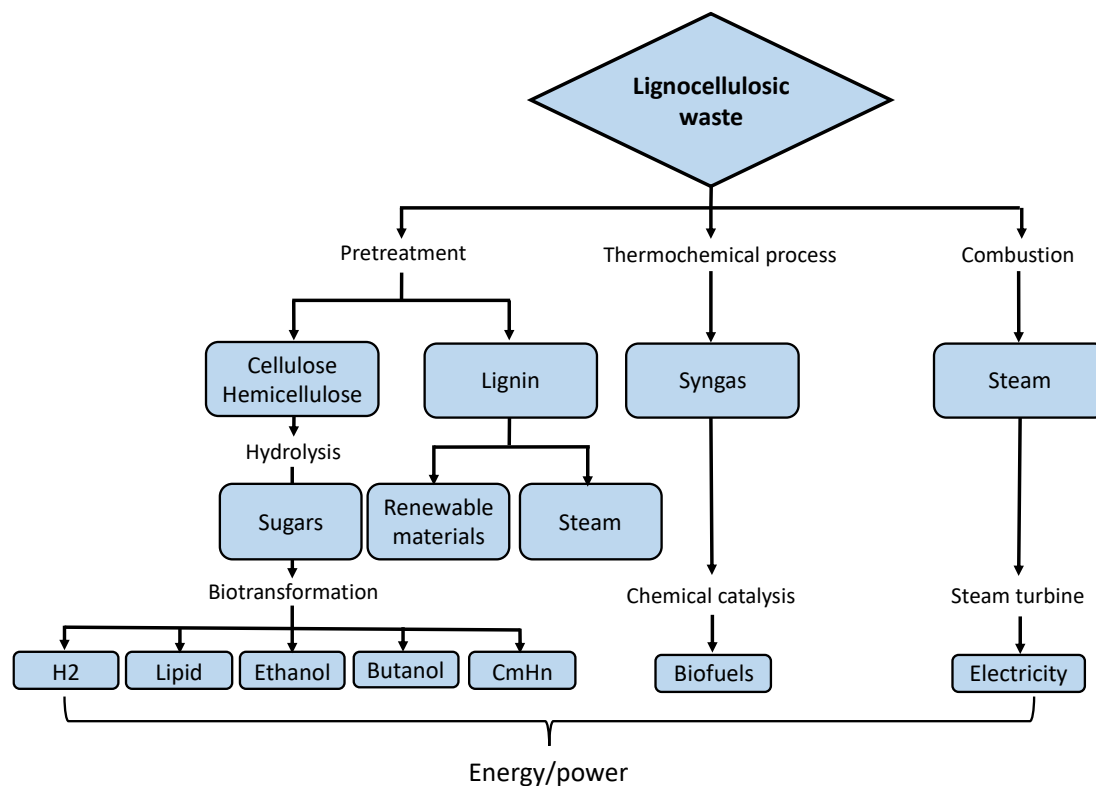
Figure I-7. Scheme of combined processes for energy achievement from lignocellulosic sources (Adapted from Ankush et al., 2020; Huang & Zhang, 2011)
