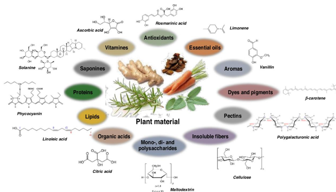
Figure I-1. Some valuable metabolites from plant materials (Source: Perino & Chemat, 2019)
