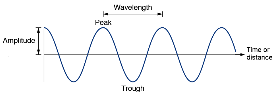
Figure I-14. Main physical parameters of an ultrasonic wave
