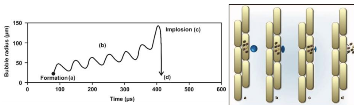
Figure I-13. Schematic representation of the effects of ultrasonic waves on plant matrices.
