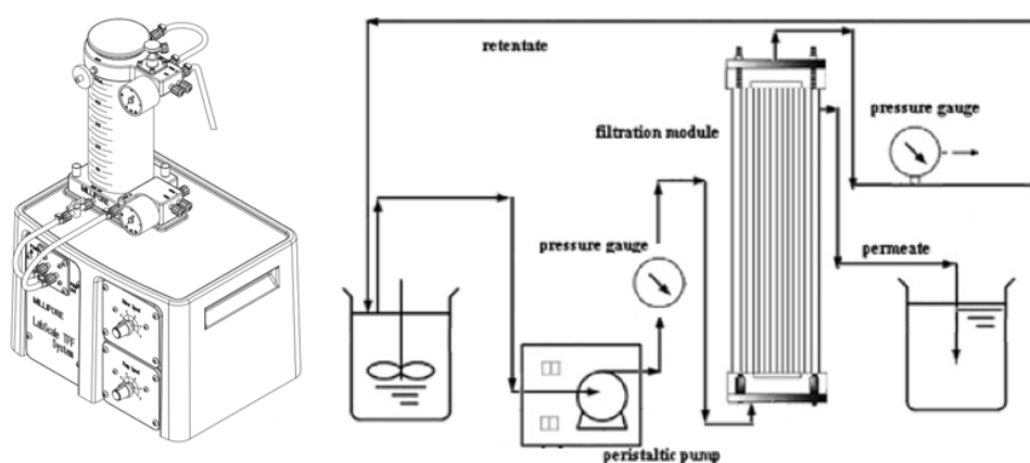
Figure II-10. Apparatus and flowchart of the tangential flow filtration system (adapted from Huang et al., 2012)
