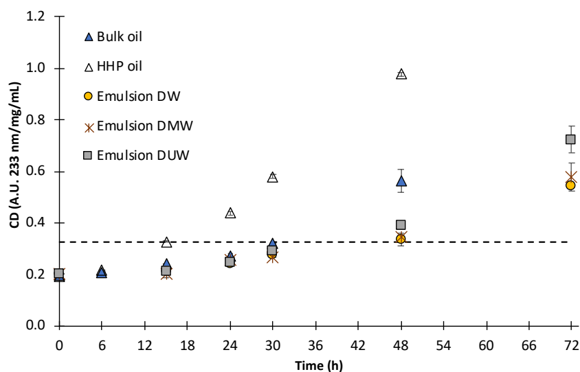
Figure IV-14. Monitoring of CD formation in either bulk linseed oil or dispersed in a 4:1 water:oil emulsion stabilized by walnut particles and submitted to accelerated oxidation at 60 °C. The dotted line indicates the limit of oil edibility.
