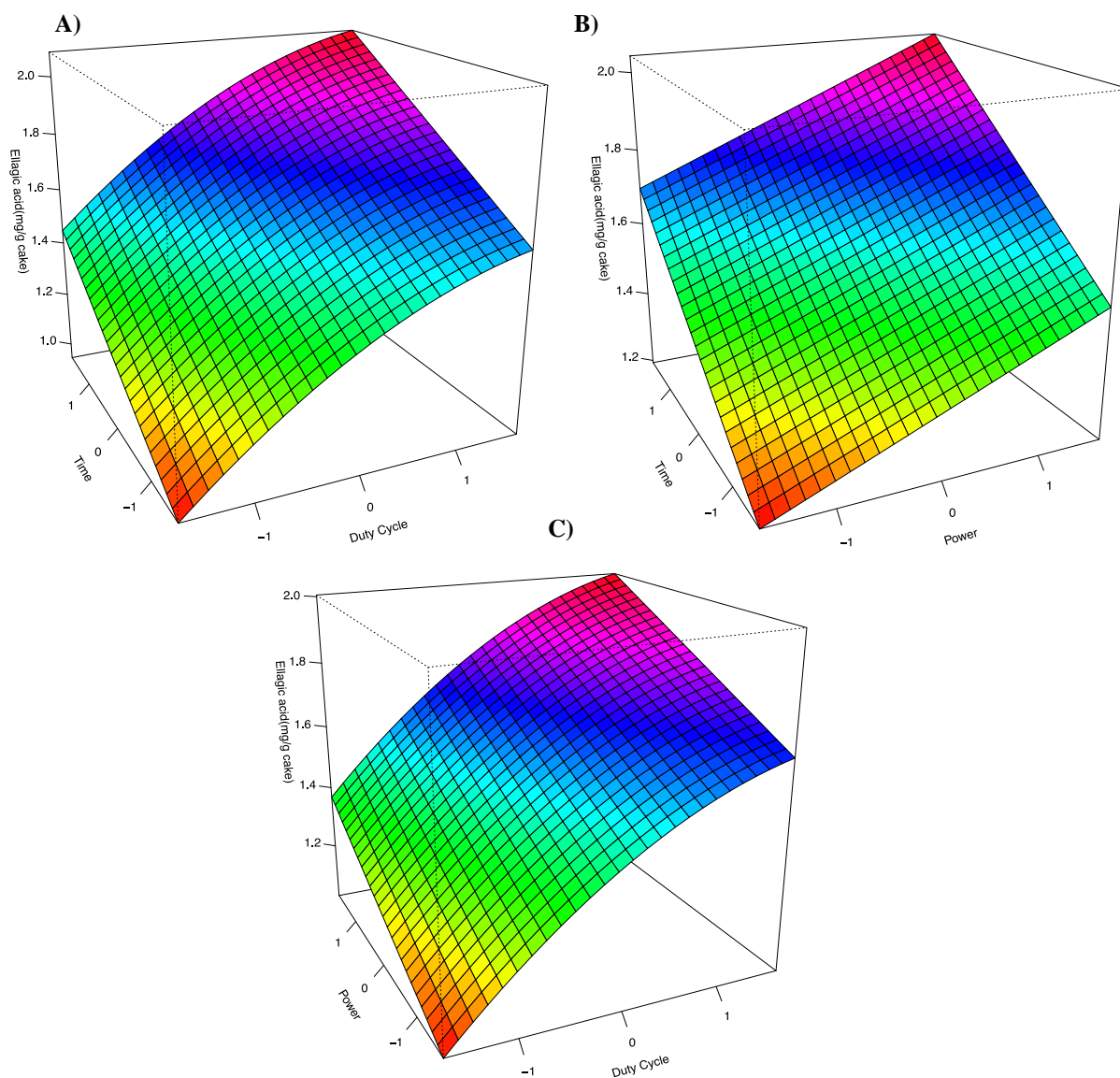
Figure IV-6. Response surface plots of the predicted model of time – duty cycle (A), time – power (B) and power - duty cycle (C) for ellagic acid extraction from defatted walnut cake by UAE. The third independent factor was set at 0 (coded value) to plot the response surfaces
