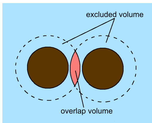
Figure IV-11. Overlap of excluded volumes of hard spheres
