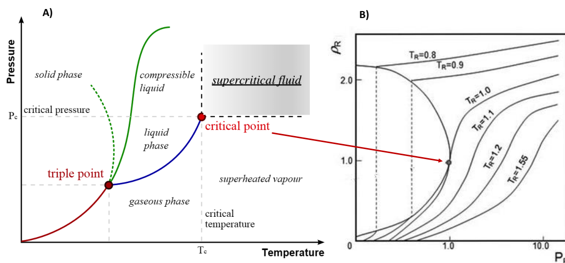
Figure I-15. Typical pressure–temperature phase diagram of pure substances (dotted green shows the anomalous behavior of water) (A) and CO 2 density–pressure phase diagram at different temperatures considering reduced variables ( T_R = T/T_C , P_R = P/P_C and \rho_R = \rho/\rho_C ) (B)
