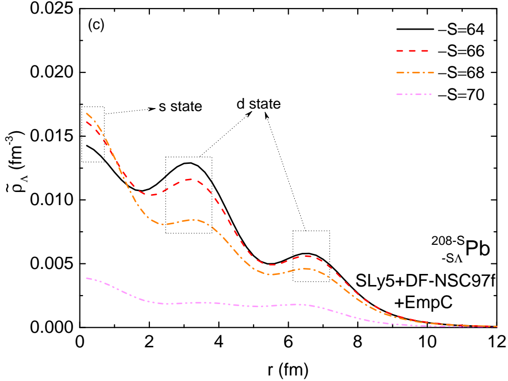
Fig. 2.7: \Lambda pairing densities for ^{40}_{-S\Lambda}\text{Ca} (a), ^{132}_{-S\Lambda}\text{Sn} (b), and ^{208}_{-S\Lambda}\text{Pb} (c) hypernuclei, calculated with the HFB approach.
