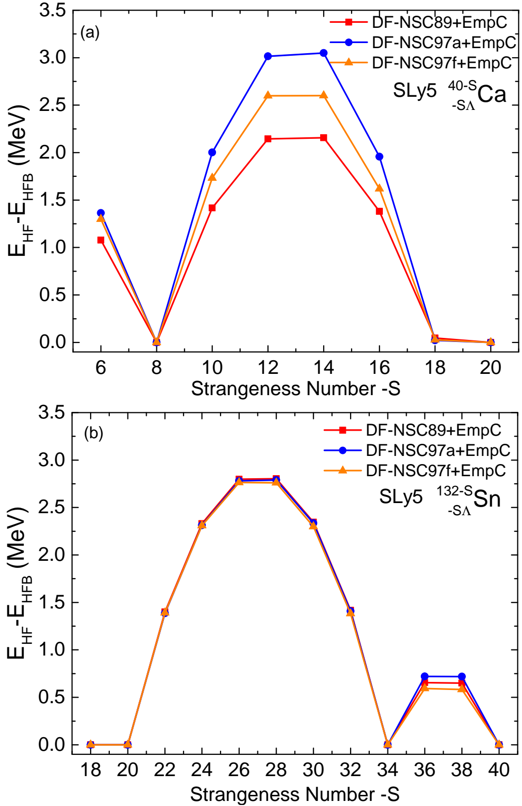
Fig. 2.5: Difference of binding energies between HF and HFB for {}^{40}_{-S\Lambda}\text{Ca} (a) and {}^{132}_{-S\Lambda}\text{Sn} (b) hypernuclei with DF-NSC89+EmpC, DF-NSC97a+EmpC and DF-NSC97f+EmpC force sets.
