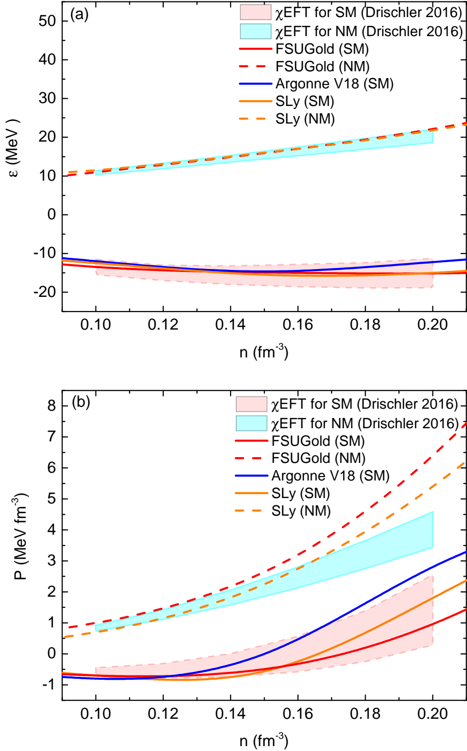
Fig. 3.3: Energy (a) and Pressure (b) distributions calculated by using \chi EFT from the Ref. [DHS16] for both symmetric matter (SM) and neutron matter (NM).
