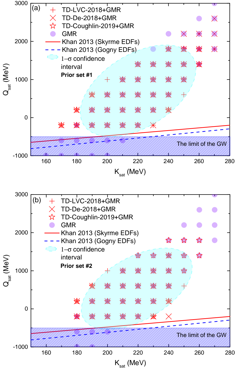
Fig. 4.9: The values of the K_{\text{sat}} and Q_{\text{sat}} inside of the 1-\sigma probability for the prior set #1 (a) and #2 (b) with a spurious correlation found for Skyrme and Gogny EDFs from Ref [KM13]. Note that the \chi EFT constraint is included for all joint posteriors.
