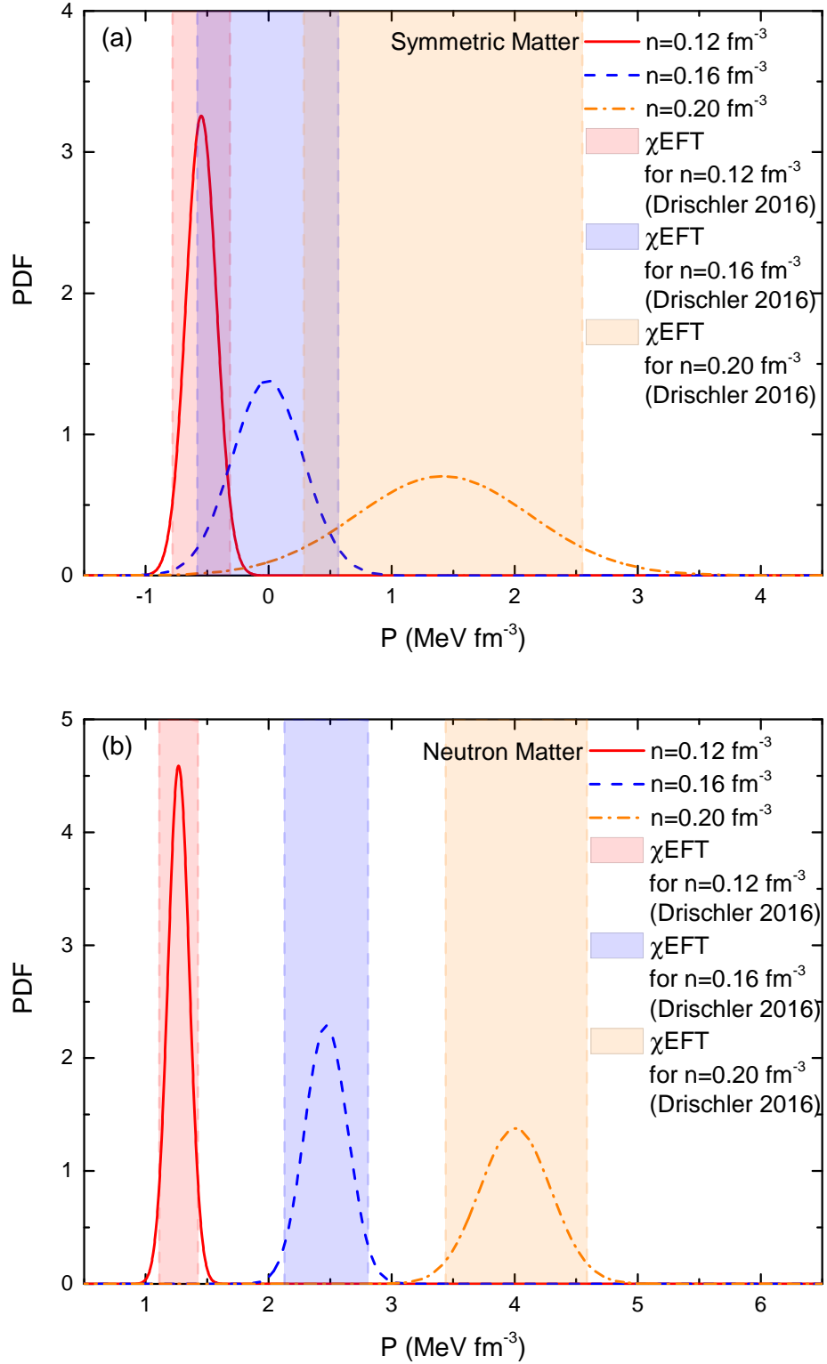
Fig. 3.4: Pressure posterior functions in neutron matter (NM) (a) and symmetric matter (SM) (b) obtained from the constraint C3 associated to the \chi EFT bands calculated in Ref. [DHS16].
