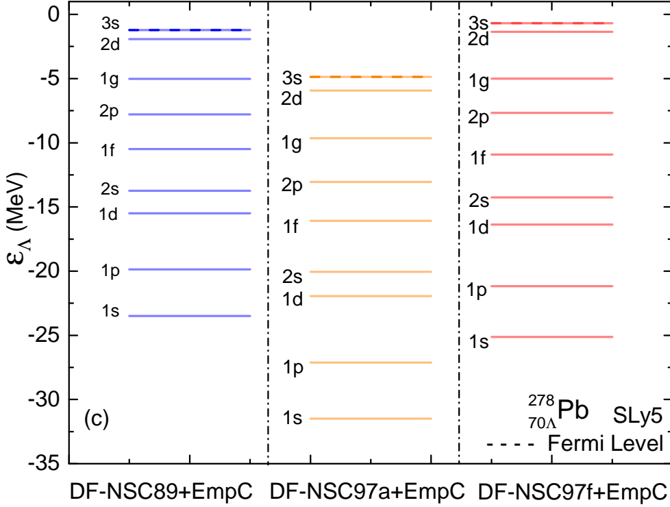
Fig. 2.1: The \Lambda single particle spectrum {}_{20\Lambda}^{60}\text{Ca} (a), {}_{40\Lambda}^{172}\text{Sn} (b) and {}_{70\Lambda}^{278}\text{Pb} (c) hypernuclei, calculated with the HF approach.
