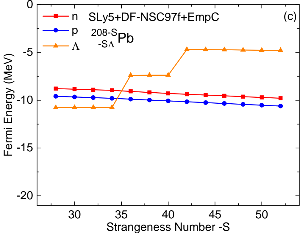
Fig. 2.2: Evolution of proton, neutron and \Lambda Fermi energies function of strangeness number -S for ^{40-S}_{-S\Lambda}\text{Ca} (a), ^{132-S}_{-S\Lambda}\text{Sn} (b), and ^{208-S}_{-S\Lambda}\text{Pb} (c) hypernuclei with the HF approach.
