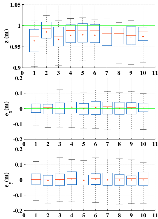
Figure 5.10 – Box and whisker plot for 10 trials of the STSMC method after four successive failures in square trajectory flight, showing the altitude z(m) , and position errors e_x(m) and e_y(m) between t=17s and t=45s .
