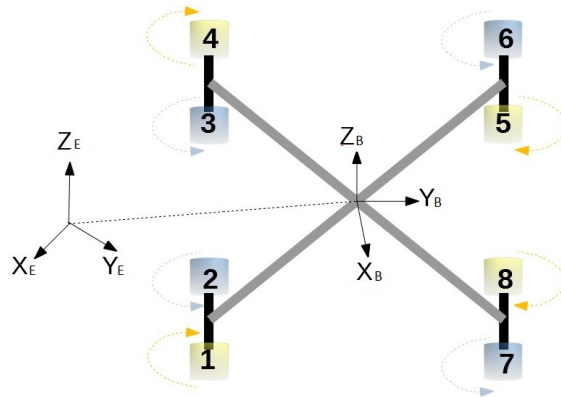
Figure 2.3 – Octorotor's configuration
