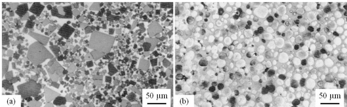
Figure I-28 Micrographs showing the microstructures of samples sintered at 1450°C for 1h in vacuum (13 Pa), (a) NbC-30wt%Fe, (b) NbC-30wt%Fe-3wt%B [46].
