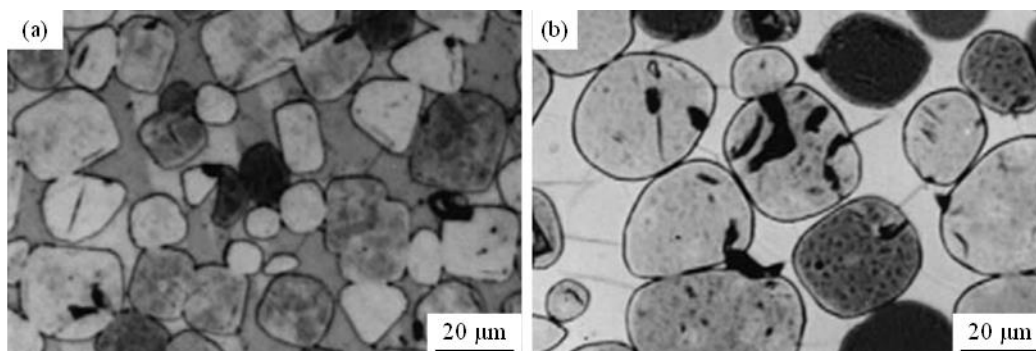
Figure I-26 Grain growth phenomenon in a NbC-30wt%Co-2.3wt%B material sintered for 2h in vacuum at (a) 1400°C, (b) 1550°C [55].
