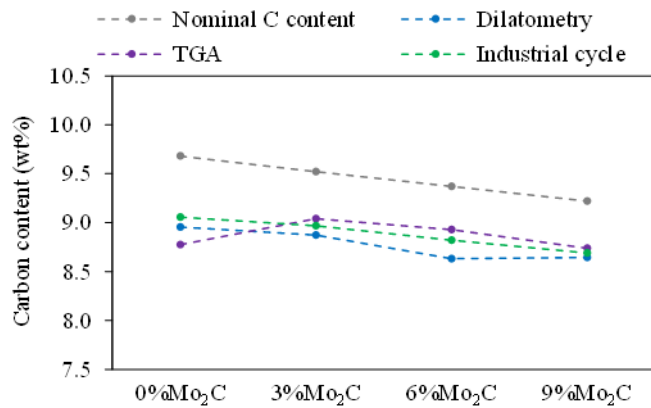
Figure V-2 Carbon content after sintering at 1450°C in vacuum compared to the recalculated nominal carbon content for NbC-12vol%Ni-0.5vol%WC samples with different amount of Mo 2 C.
