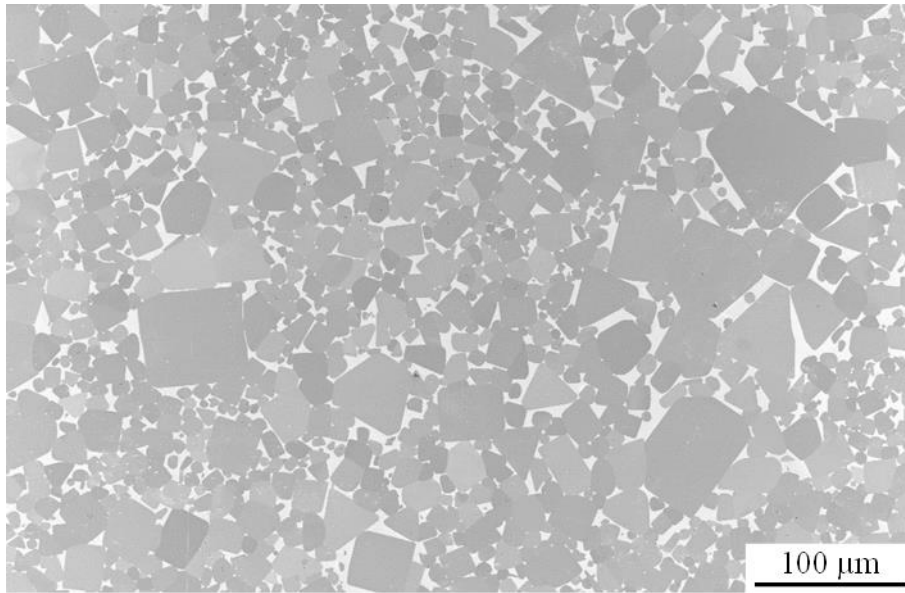
Figure VI-2 Microstructure of NbC-12vol%Ni sintered at 1360°C in vacuum with a dwelling time of 4h, abnormally big grains are visible.
