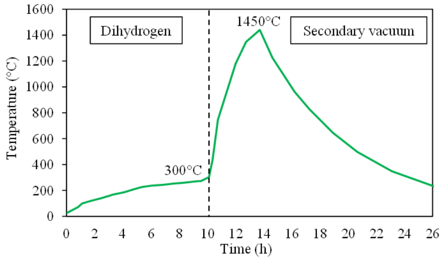
Figure II-15 Industrial debinding & sintering thermal cycle
