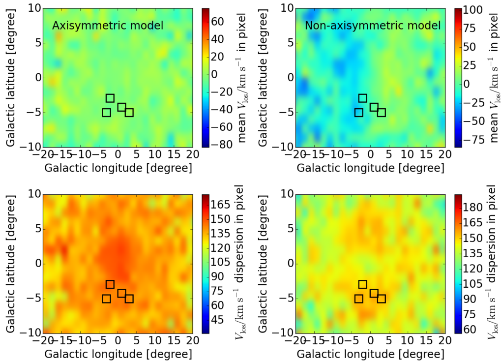
Figure 6.4: Kinematics maps toward the bulge regions as predicted for our halo particle simulations, before and after bar formation. Left for the axisymmetric model and right the non-axisymmetric model or after bar model is added. The black squares shows the Galactic localization of the BRAVA-RR stars studied by Kunder et al. (2016) .
