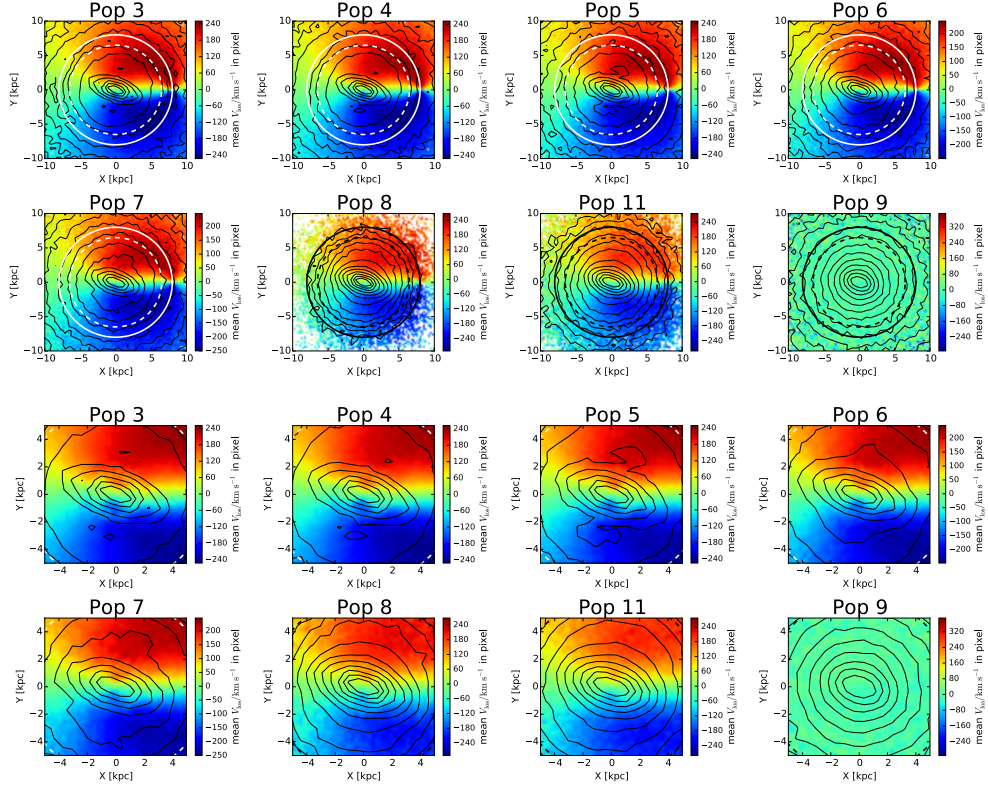
Figure 5.16: Predicted line-of-sight velocity maps of our best model (see text) in the region delimited by |X| < 10 kpc and |Y| < 10 kpc (first and second row), and a zoomed-in view of the same region delimited by |X| < 5 kpc and |Y| < 5 (third and fourth row). Corotation radius is shown in white and black dashed line, and the Solar radius is shown in white and black solid line. The thin black lines shows the logarithmic surface density contours of the disk and halo particles. Colors indicate \langle V_{los} \rangle in units of \text{km s}^{-1} .
