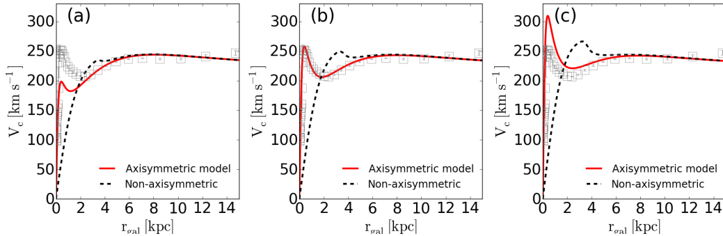
Figure 3.7: Rotation velocity profile for three models with different bar mass (Non-axisymmetric model) and different mass for the spherically symmetric component (Axisymmetric model): 0.63 \times 10^{10} M_{\odot} (panel a), 1.1 \times 10^{10} M_{\odot} (panel b), and 1.6 \times 10^{10} M_{\odot} (panel c). Grey symbols to guide the eye based on the observations of H_I and CO from Sofue (2015).
