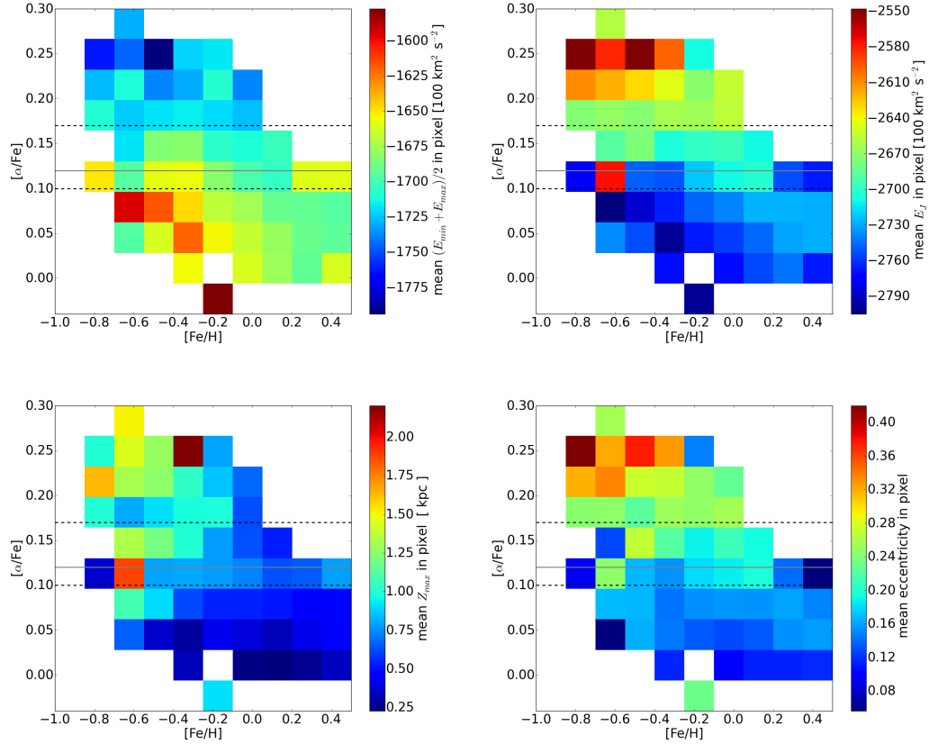
Figure 8.4: [\text{Fe}/\text{H}] vs. [\alpha/\text{Fe}] distribution showing the mean orbital elements per bin: the characteristic orbital energy ( \frac{E_{max}+E_{min}}{2} ) as defined in Moreno et al. (2015) , the orbital Jacobi energy E_J , maximum height above the plane Z_{max} , and the eccentricity e . The black dashed lines show the cuts employed by Allende Prieto et al. (2016) to split the sample into thin disk and thick disk component, while the grey line show our arbitrary cut to divide the sample into a \alpha -rich disk and a \alpha -poor disk.
