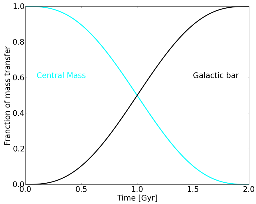
Figure 4.2: Adiabatic growth of the boxy bar (see text).
