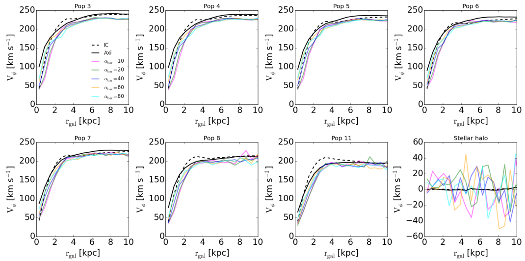
Figure 4.4: Radial distribution of the mean azimuthal velocity V_\phi as a function of Galactocentric distance ( r_{\text{gal}} at relatively smaller heights from the plane ( |Z| < 0.3 kpc). The black dashed line refers to the initial conditions ( t = 0 Gyr), the black line is the resulting V_\phi from the axisymmetric model after 5 Gyr forward integration, and the colored lines are the resulting V_\phi along different azimuthal angles labeled here as \alpha_{\text{bar}} , and after 5 Gyr forward integration in the non-axisymmetric potential which includes a boxy/peanut bar (see text).
