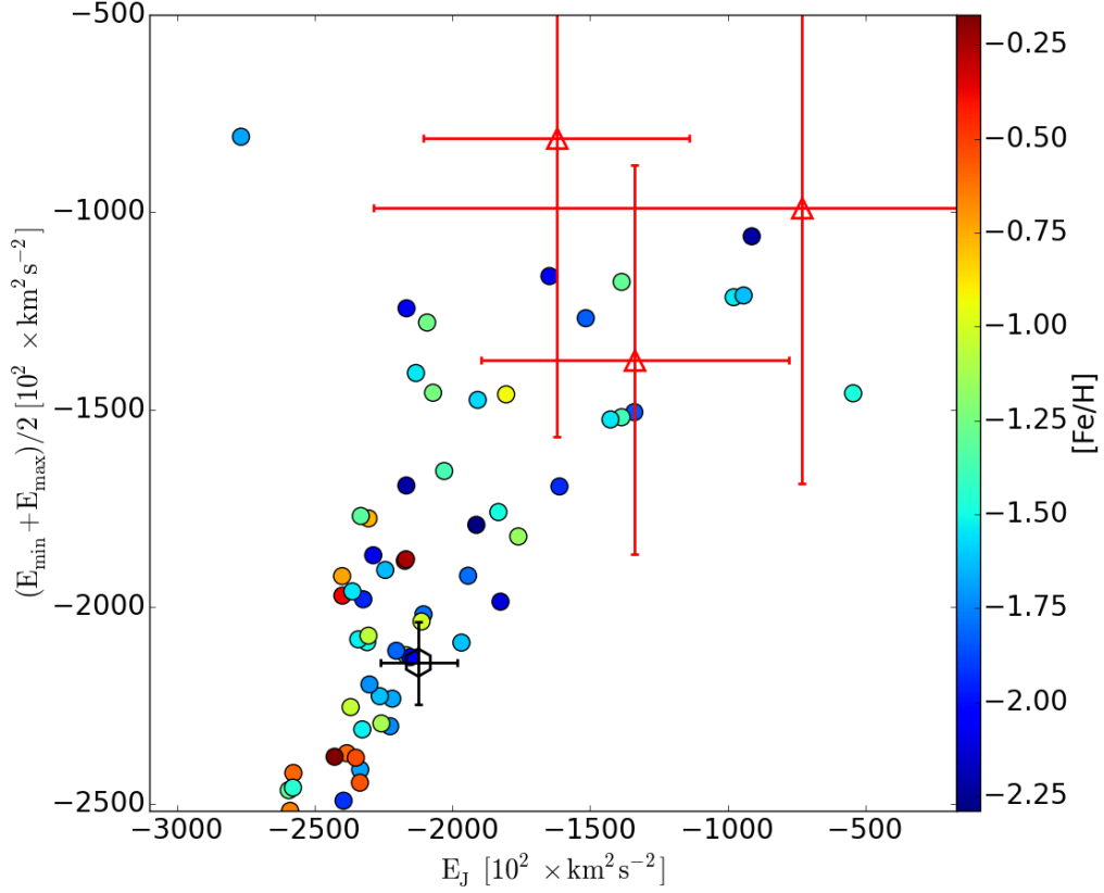
Figure 8.8: The characteristic orbital energy (E_{min} + E_{max})/2 versus the orbital Jacobi energy E_J as defined in Eq. B.19. This plot shows the energy distribution for 63 globular clusters listed in Table C.2, one giant star from Fernández-Trincado et al. (2016a), and three migrant stars (red triangle symbols) from Martell et al. (2016). Colours represent the metallicity of each globular cluster from Harris (2010).
