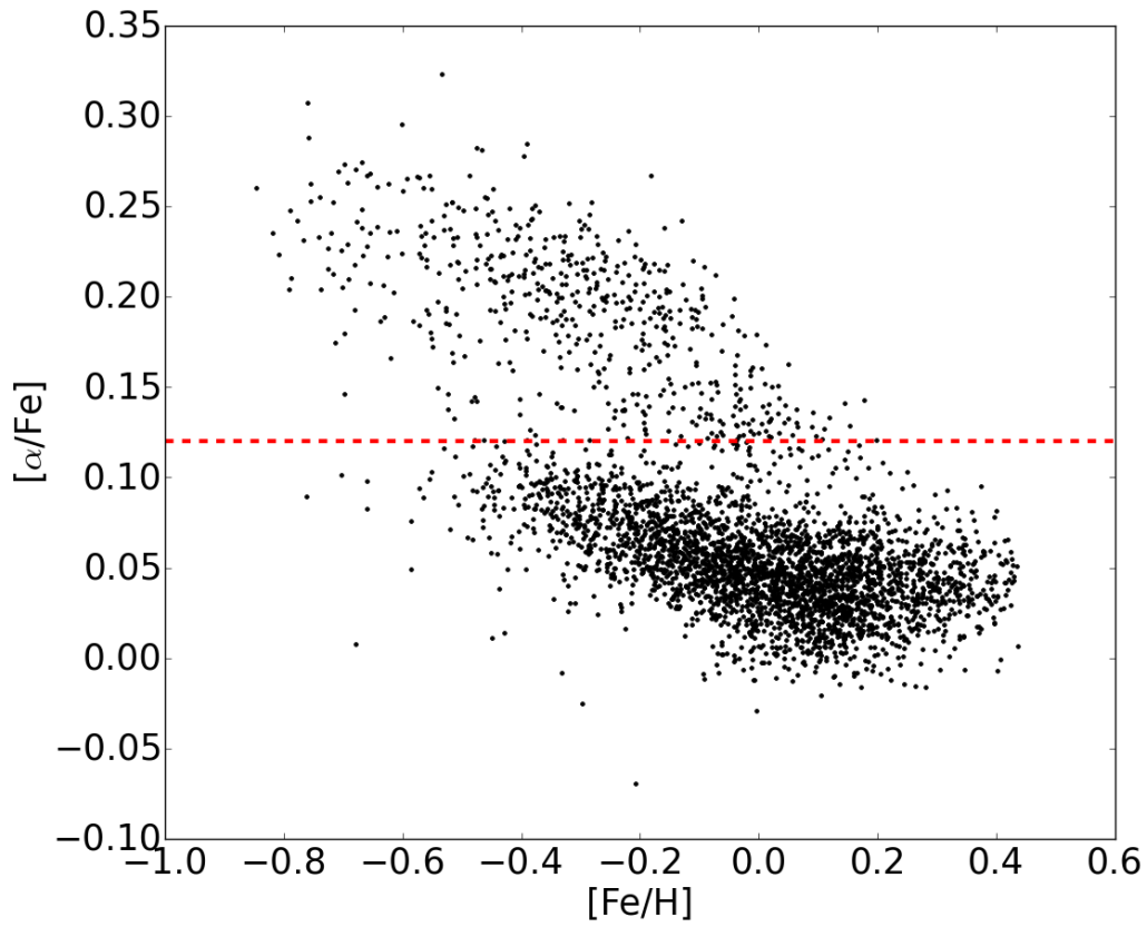
Figure 8.5: [Fe/H] vs. [\alpha/Fe] distribution taken from the compilation of the TGAS plus APOGEE datasets from Allende Prieto et al. (2016) . The red dashed line show our arbitrary cut to split the sample into a thin disk and thick disk component.
