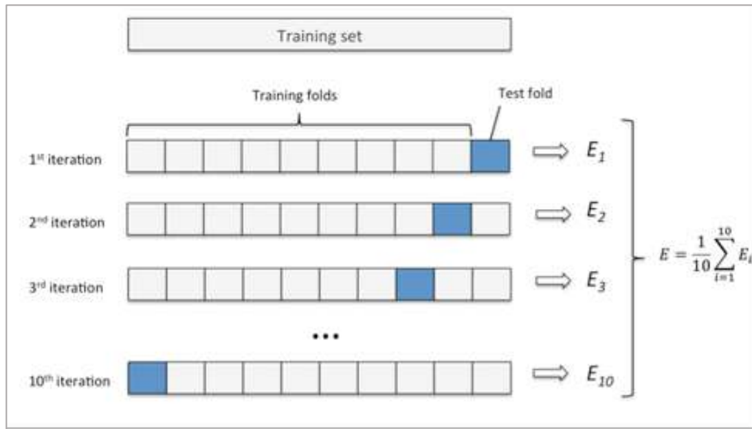
Figure 2.12: 10-fold cross validation. The designated training set is further divided up into K folds ( K=10 ), each of these will now function as a hold-out test set in K iterations. Finally, the scores obtained from the model on individual iterations are summed and averaged into the final score.
