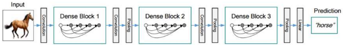
Figure 4.8: A deep DenseNet with three dense blocks. The layers between two adjacent blocks are referred to as transition layers and change feature-map sizes via convolution and pooling [62].
