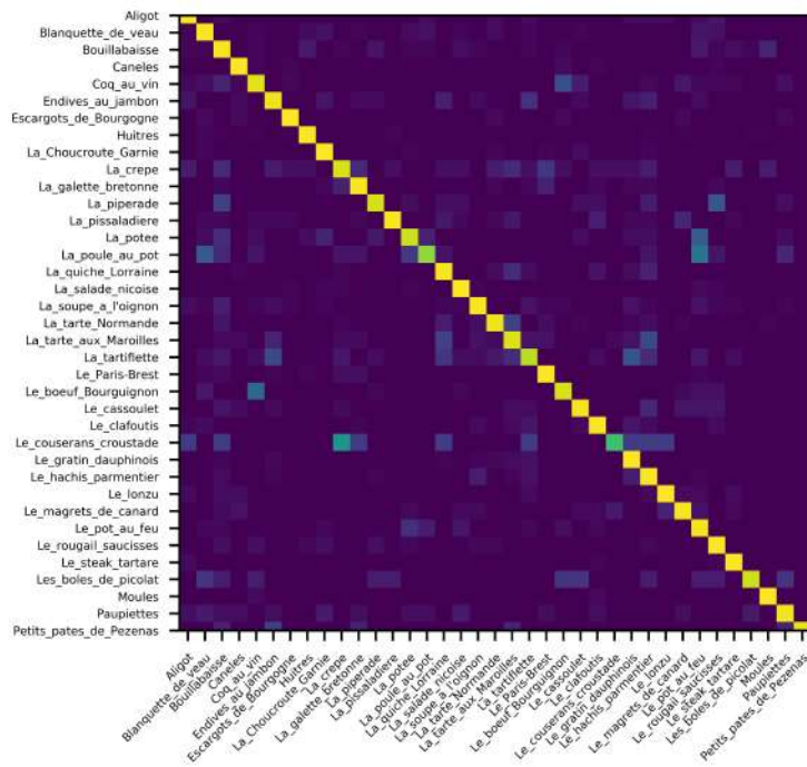
(c) ResNet18
