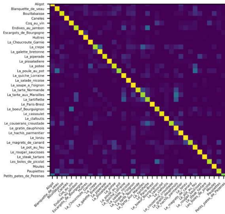
(b) Inception-v3
