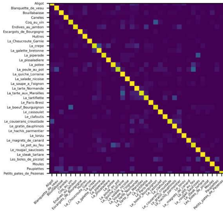
(a) DenseNet
