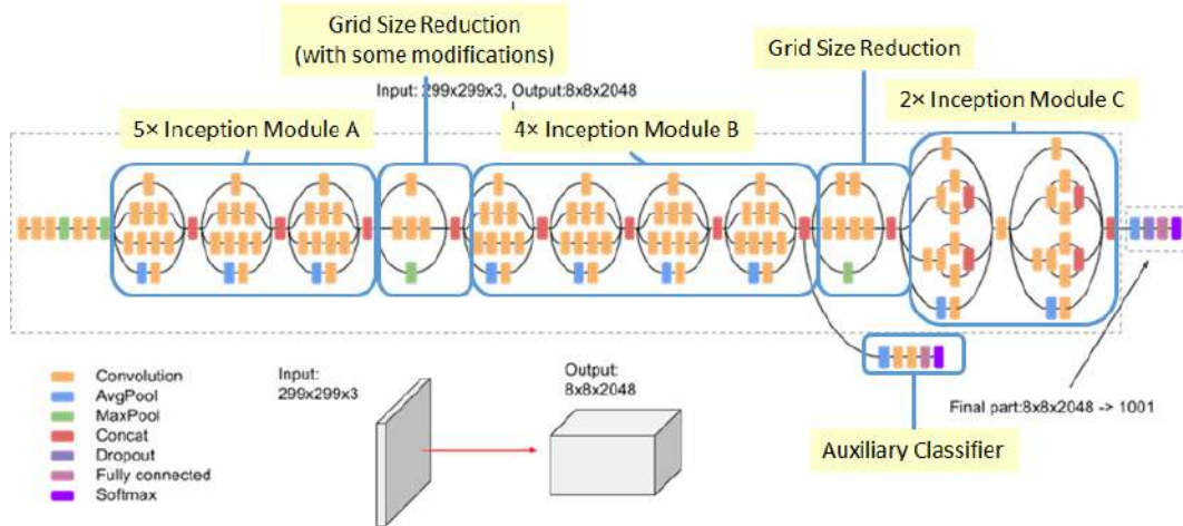
Figure 4.9: Inception-v3 Architecture [130].
