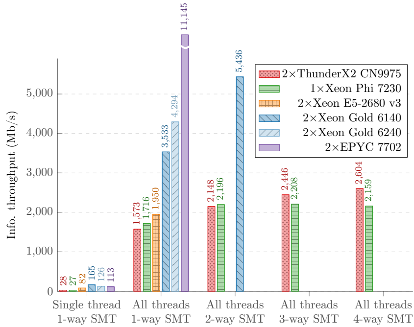
Figure 4.13 – AFF3CT simulation results of a (2048,1723) Polar code, FA-SSCL decoder L = 32 , BPSK modulation, AWGN channel, E_b/N_0 = 4.5 dB (BER = 4.34e-10 , FER = 5.17e-08 ).
