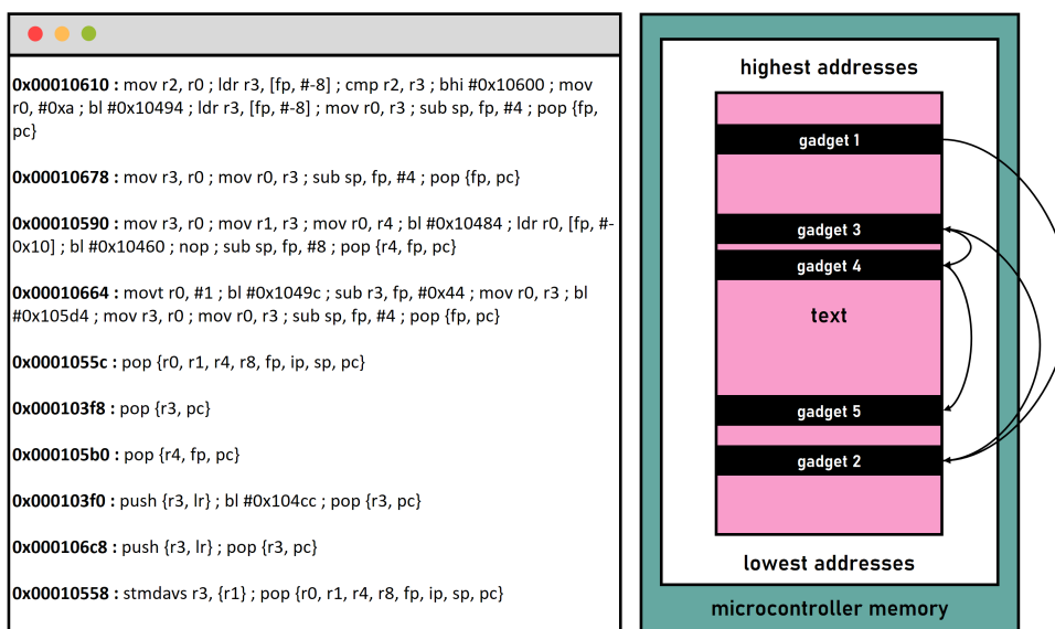
Figure 1.17: ROP signature
