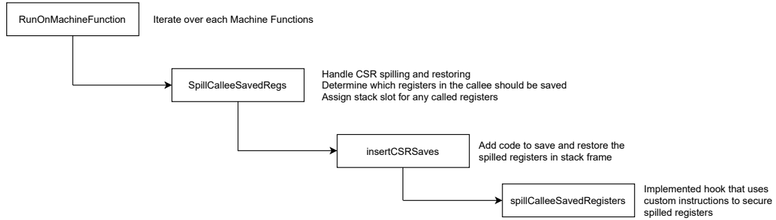
Figure B.2: LLVM PEI pass
