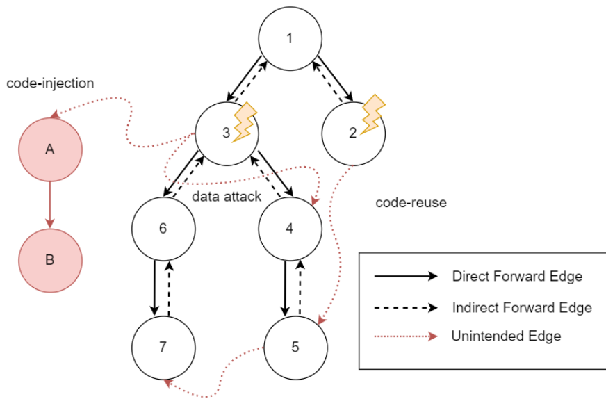
Figure 1.11: Memory safety attacks
