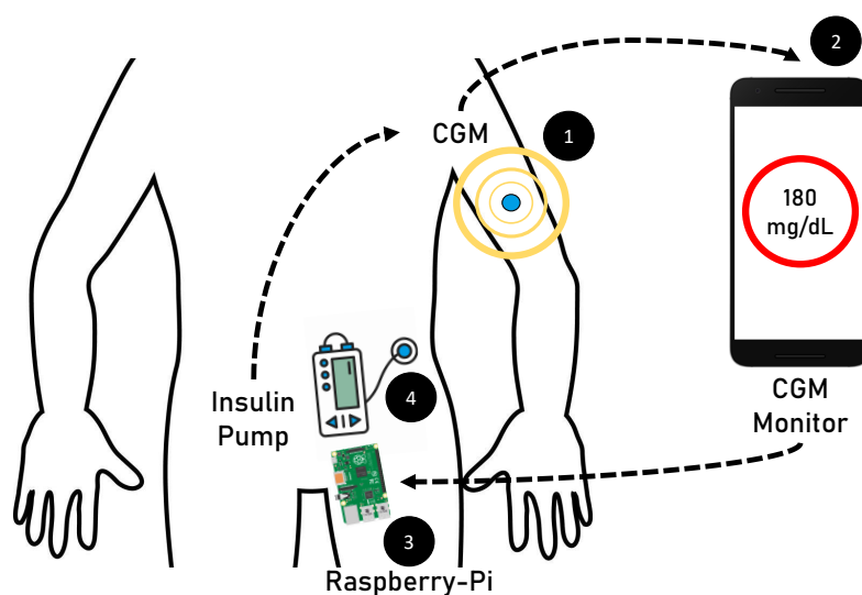
Figure 3.2: OpenAPS closed-loop
