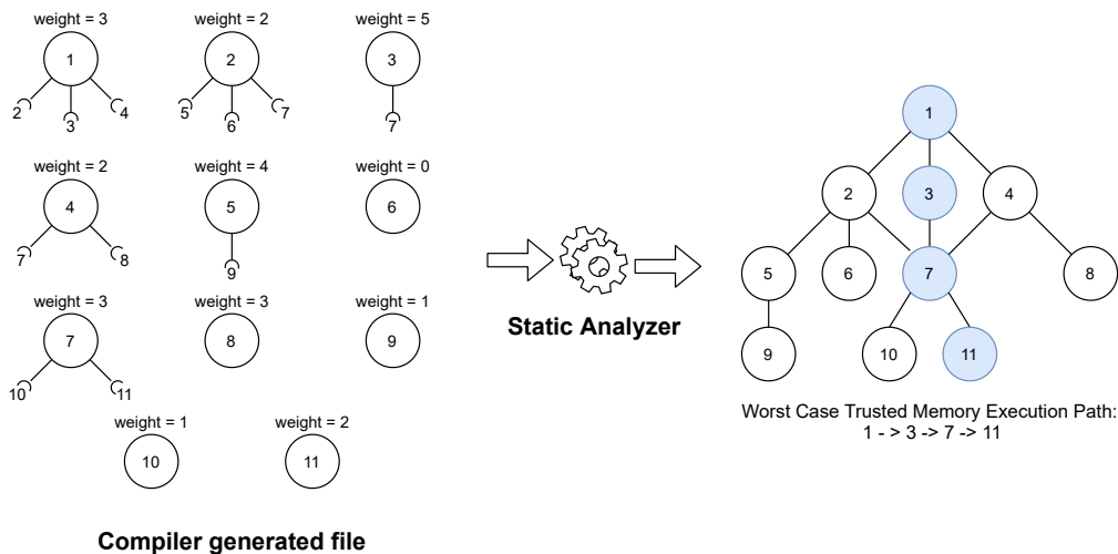
Figure 4.7: Static Analyzer.
