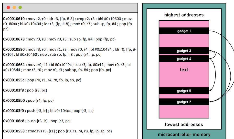
Figure 1.17: ROP signature
