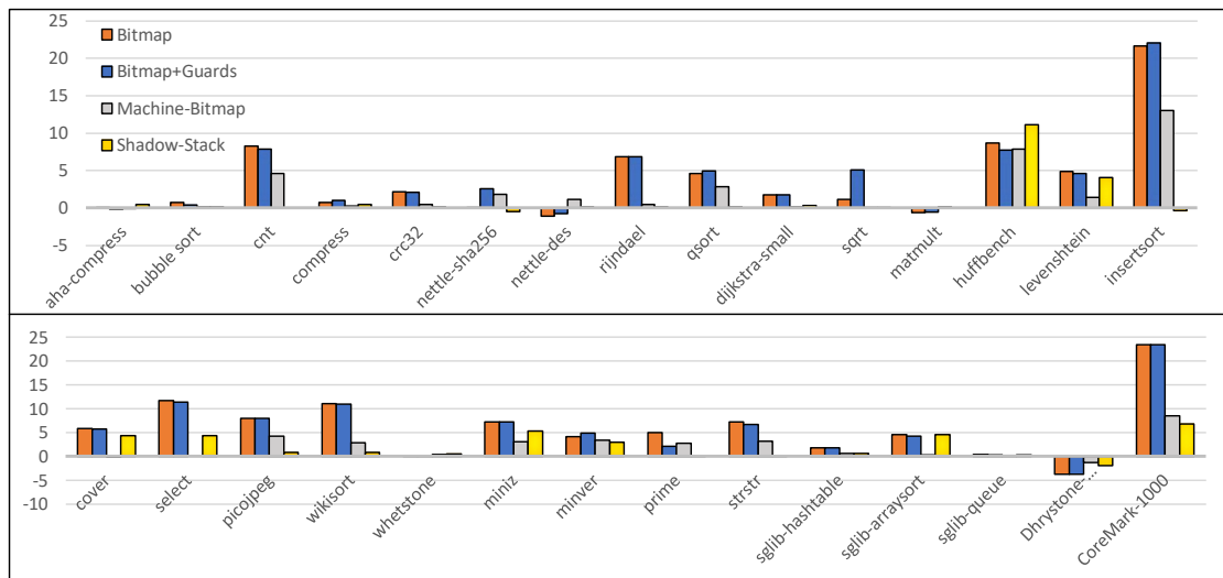
Figure 5.10: BackGuard benchmarks
