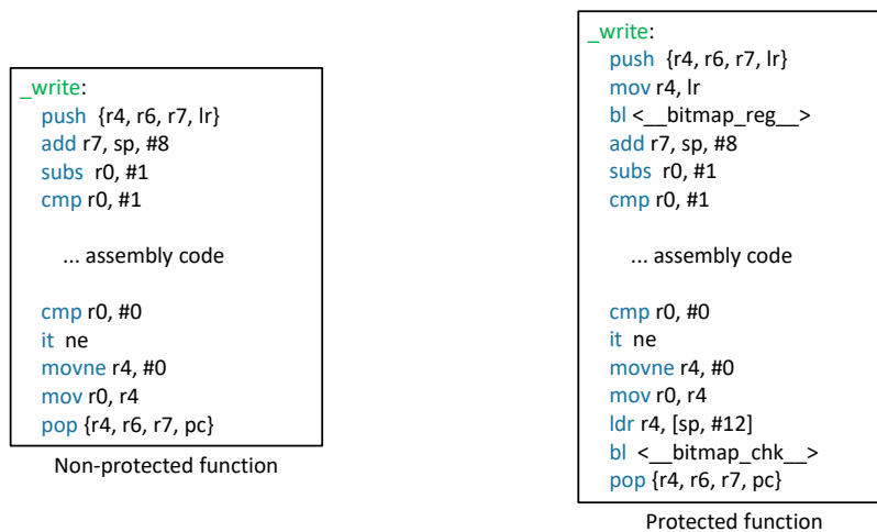
Figure C.1: BackGuard Machine pass generated Code
