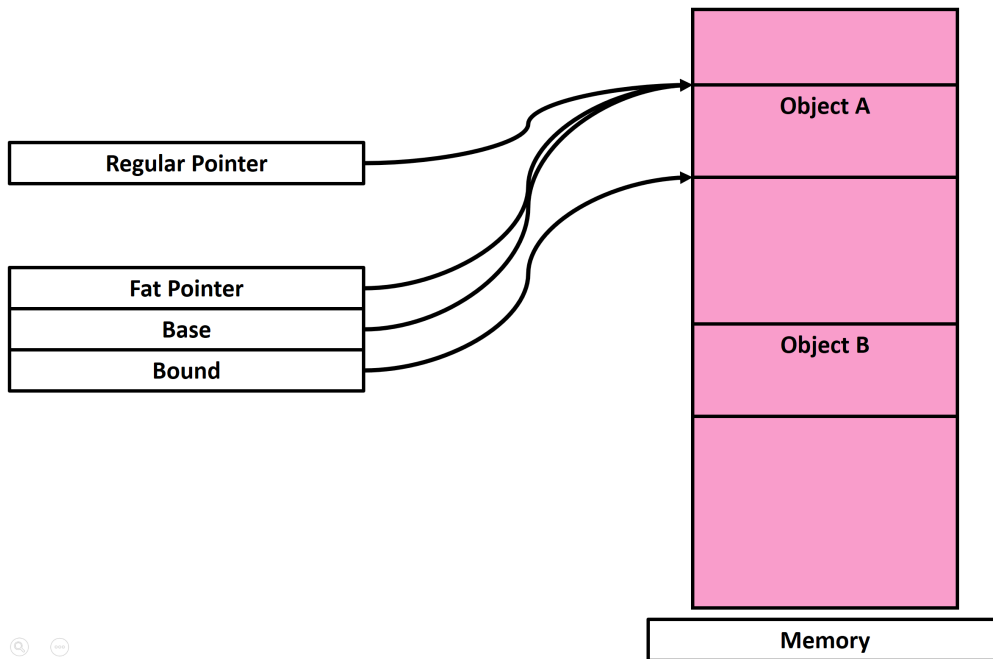
Figure 1.19: Fat Pointer
