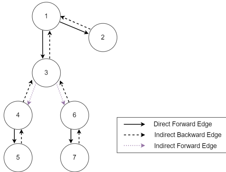
Figure 1.4: Control-flow graph
