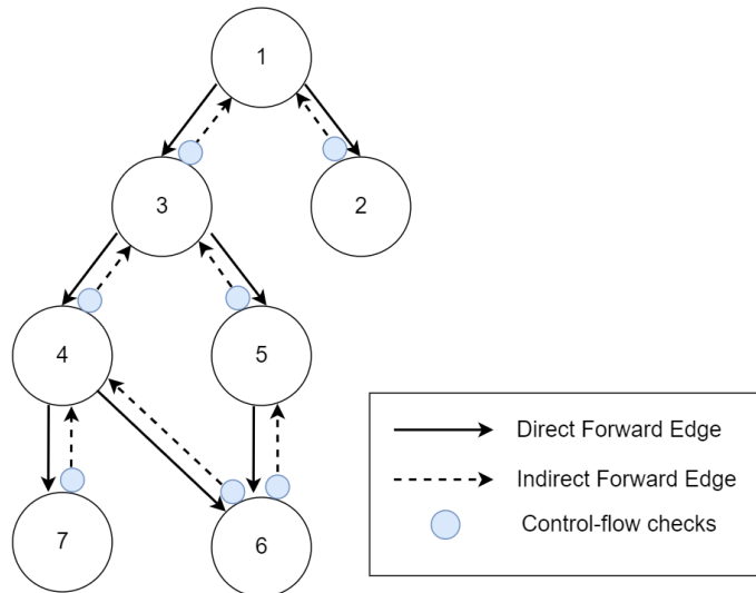
Figure 1.12: Control-flow integrity
