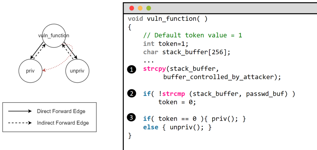
Figure 1.10: Data-oriented attack
