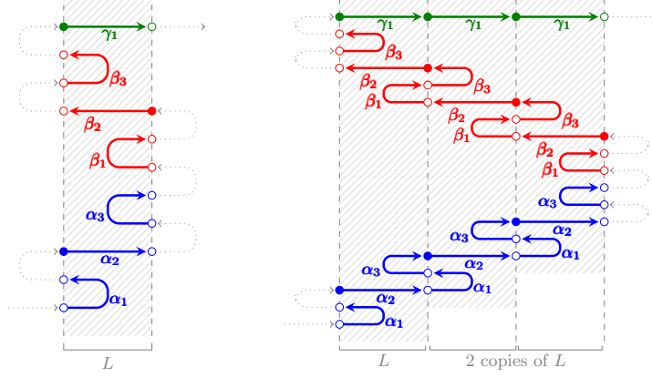
Figure 3.11: Pumping an idempotent loop with three components.
