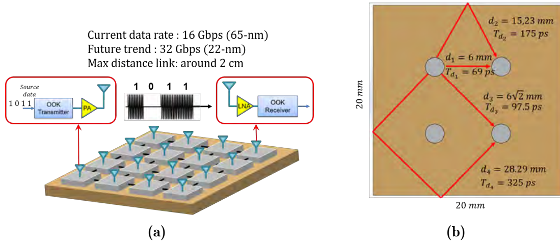
Figure 1: (a) General principle of WiNoC communications. (b) Two examples of multipath propagated through the silicon.
