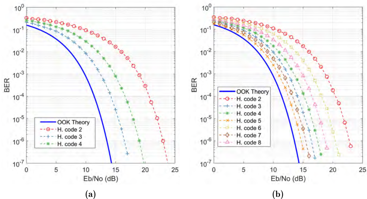
Figure 2.17: Performance evaluation for a set of (a) three Hadamard codes of length N = 4 and (b) seven Hadamard codes of length N = 8 , facing multi-path interference during single-access channel.
