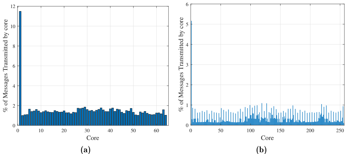
Figure 5.6: Message generated per core for the BlackScholes benchmark in a network of (a) 64 and (b) 256 cores.
