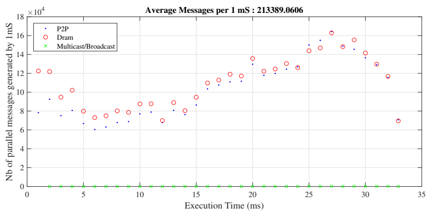
Figure 5.12: Temporal distribution of the different types of traffic (P2P, DRAM, Multicast/Broadcast) for the x264 application.
