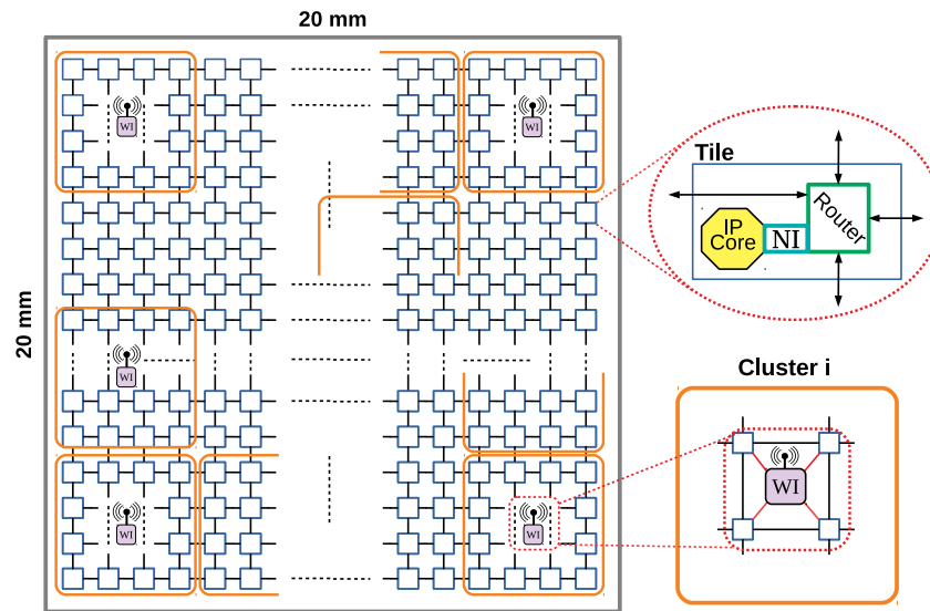
Figure 3.1: Wireless interface distribution among a clustered WiNoC hybrid topology with N clusters of M cores. The WI of a cluster is connected to four routers.
