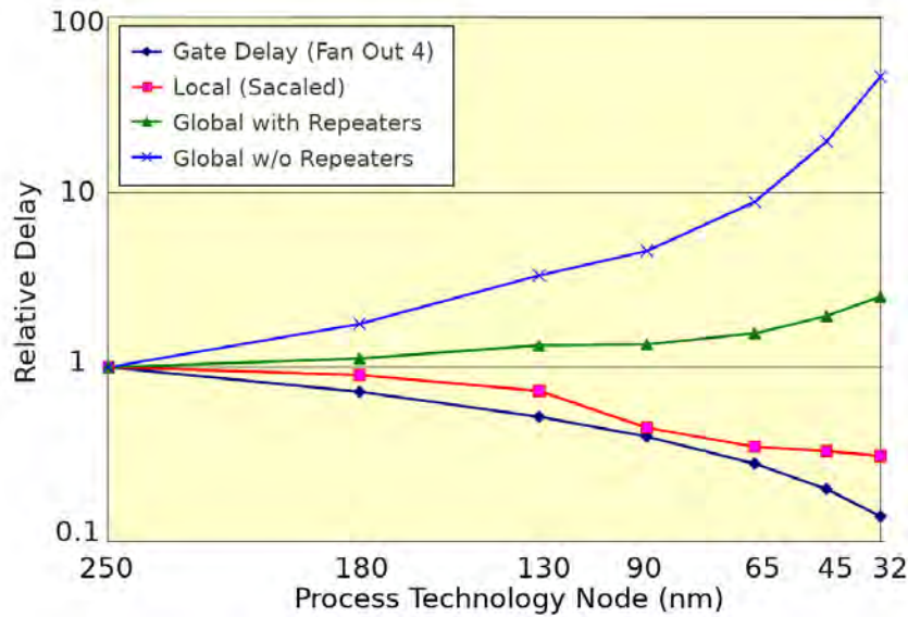
Figure 1.5: Relative delay comparison of wires vs. process technology [Sem05]
