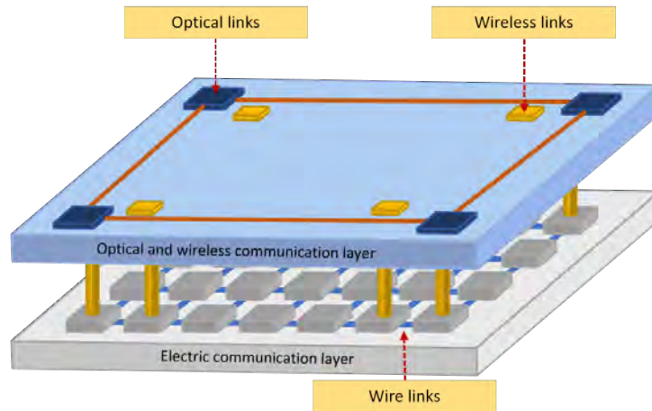
Figure 5.22: Optical/Wireless NoC Communication layer.
