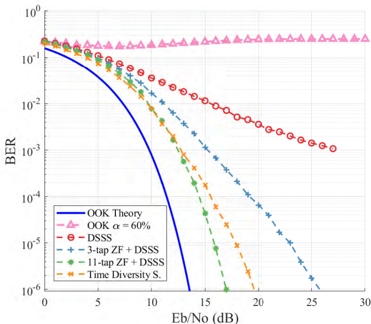
Figure 2.28: Demodulation performance BER scaling according to SNR for the considered techniques with \alpha = 60\% .
