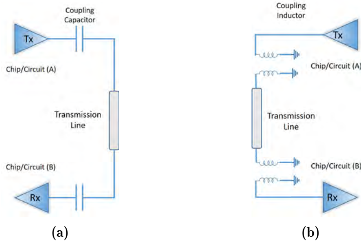
Figure 1.8: Transmission lines coupling types: (a) capacitive and (b) inductive
