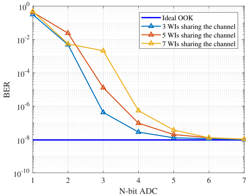
Figure 2.19: Average BER for multiple WIs sharing the channel using DSSS with OOK modulation for coherent detection in AWGN channel with QN for different values of N at SNR = 15 dB.
