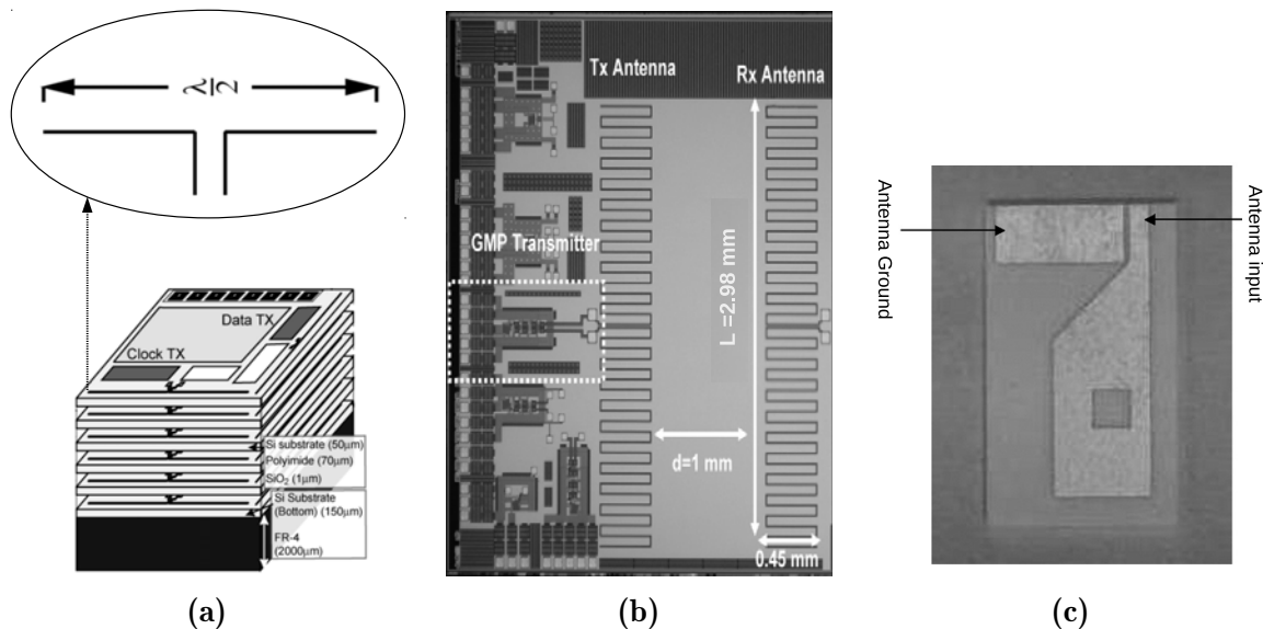
Figure 1.13: (a) Linear Dipole Antenna, (b) Meander dipole antenna, (c) Monopole antenna [YYY06]
