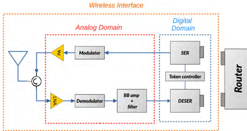
Figure 2.9: A conventional Wireless Interface of a WiNoC.
