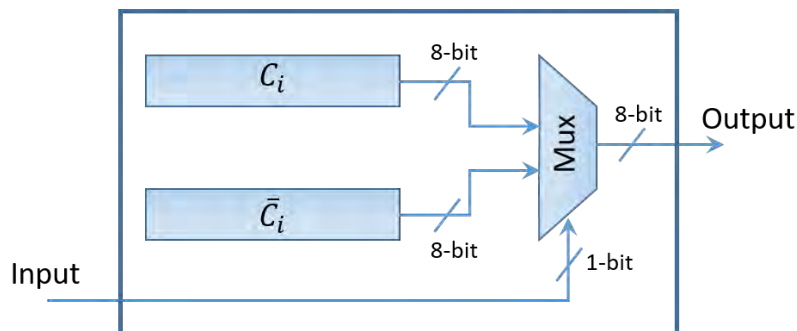
Figure 2.23: DSSS encoder architecture.
