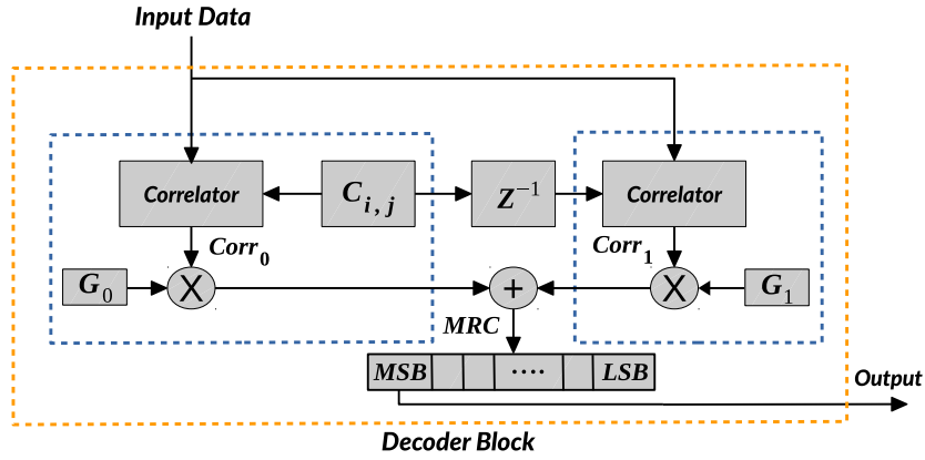
Figure 2.25: Decoder architecture of the time diversity scheme.
