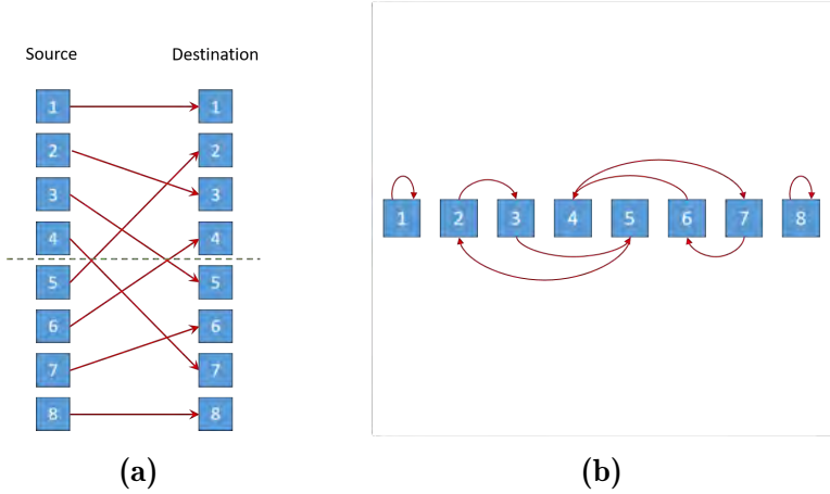
Figure 5.4: Example of (a) perfect shuffle for M = 8 cores with the obtained (b) circulating shuffle network.
