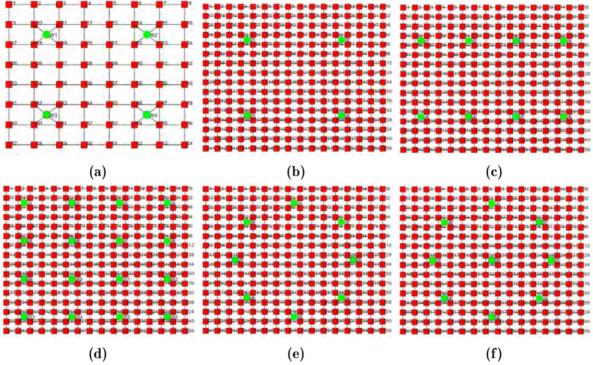
Figure 5.16: Antenna placement for evaluation of 64 and 256 cores.
