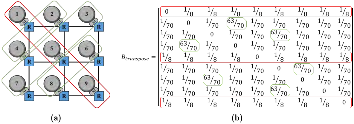
Figure 5.2: Example of M = 9 cores with transpose traffic based on (a) network mesh topology with its respective (b) frequency matrix of communication between cores.
