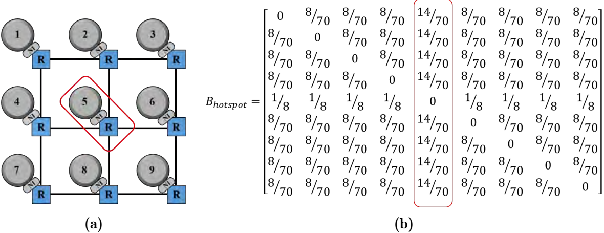
Figure 5.3: Example of M = 9 cores with hotspot traffic based on (a) network mesh topology with its respective (b) frequency matrix.
