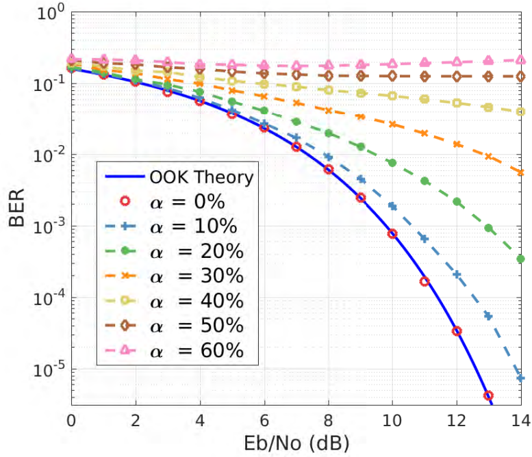
Figure 2.8: Scaling of BER performance according to the SNR per bit ( E_b/N_0 ) for different reflected-path gains in the OOK scheme.
