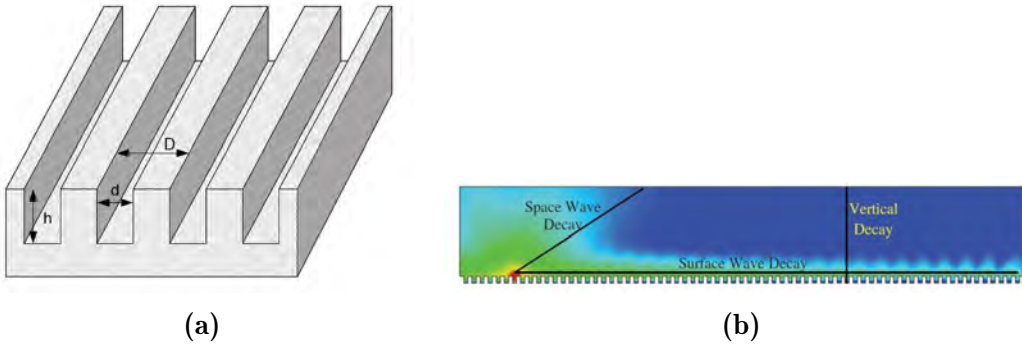
Figure 1.10: (a) Dielectric-coated metal surface, (b) E-field decay rate [Hen10]
