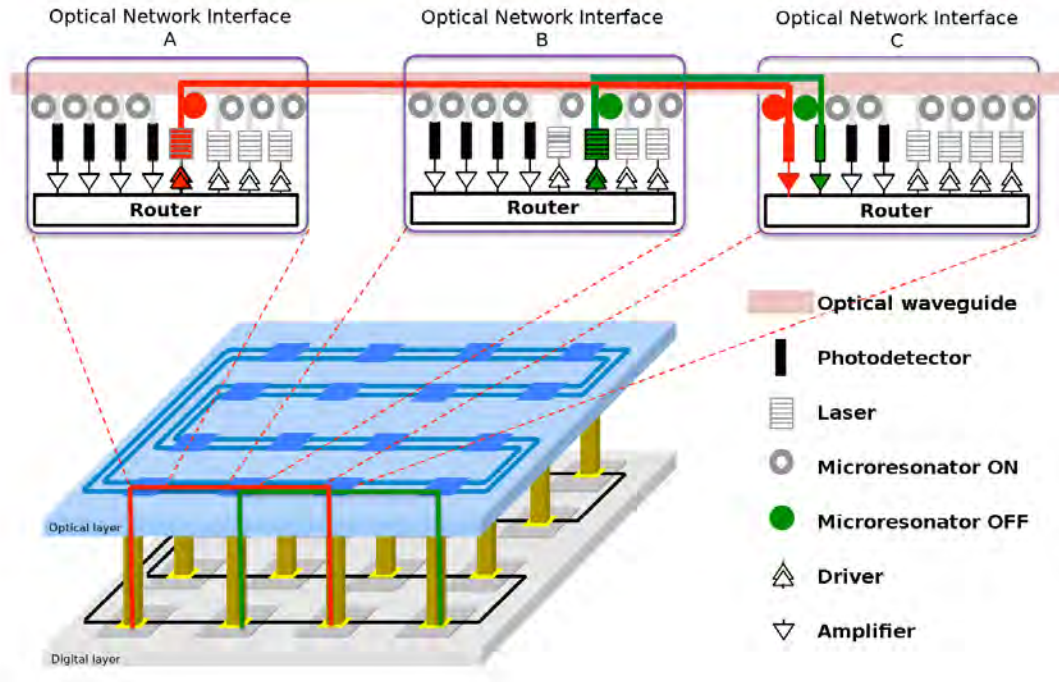
Figure 1.6: Conventional optical network interface architecture [Chi+17]
