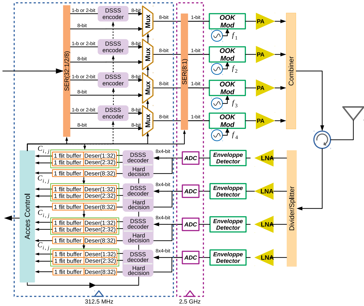
Figure 4.7: Enhanced digital-domain transceiver architecture.
