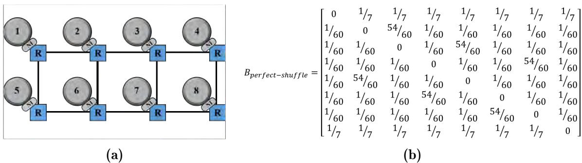
Figure 5.5: Example of M = 8 cores with perfect shuffle traffic based on (a) network mesh topology with its respective (b) frequency matrix of communication between cores.
