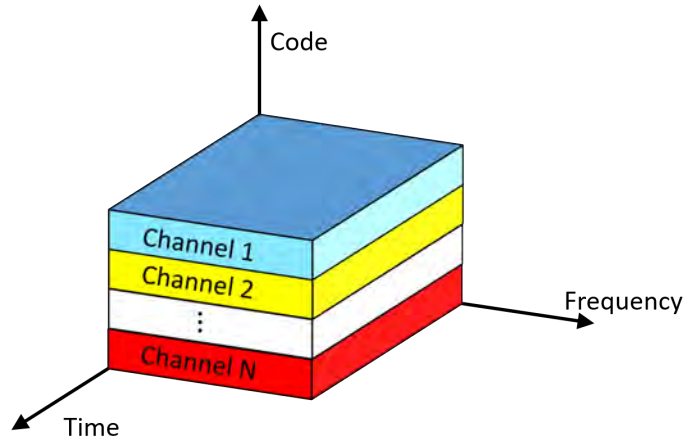
Figure 2.11: DSSS in which each channel is assigned a unique code sequence.
