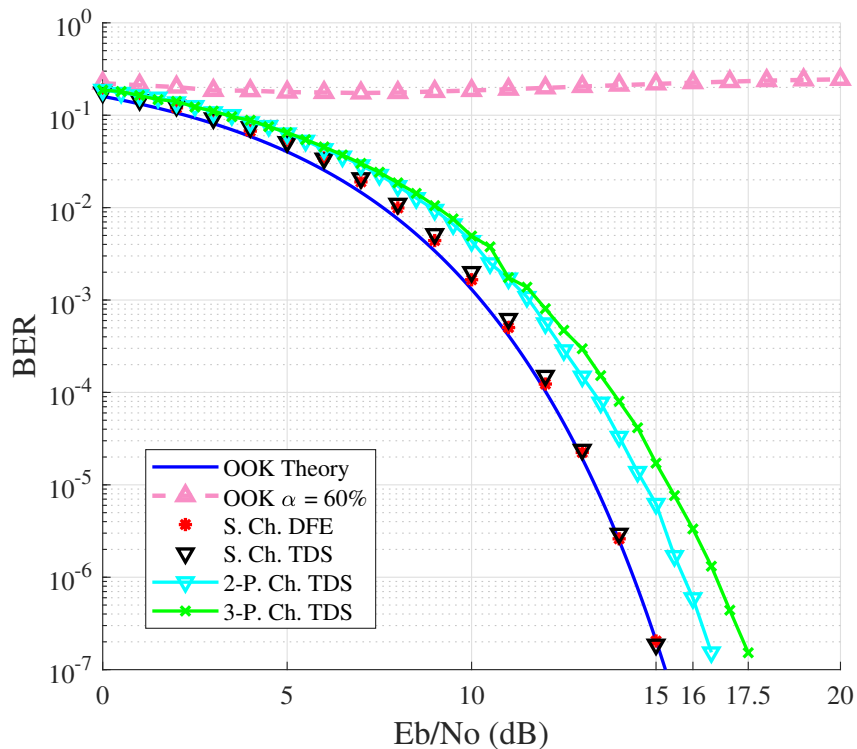
Figure 3.5: Demodulation performance BER scaling according to SNR for the considered techniques with \alpha = 60\% .
