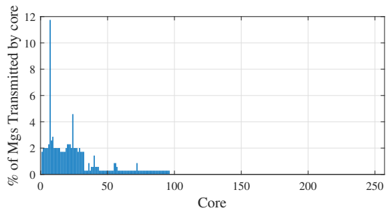
(e) RS-32_28_8_dec
