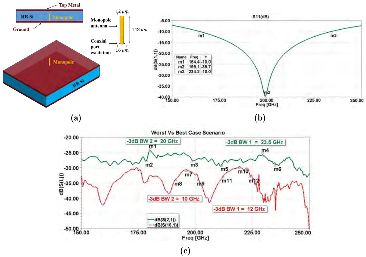
Figure 4.5: (a) Monopole antenna, (b) return loss of the antenna, (c) Frequency channel response for worst and best scenarios [Mas+19].
