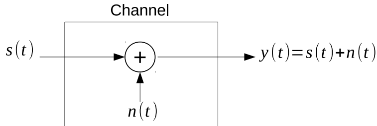
Figure 2.2: The additive noise channel
