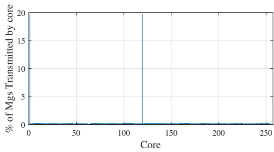
(c) H264-720p_dec
