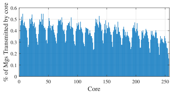
(a) FFT-1024_complex
