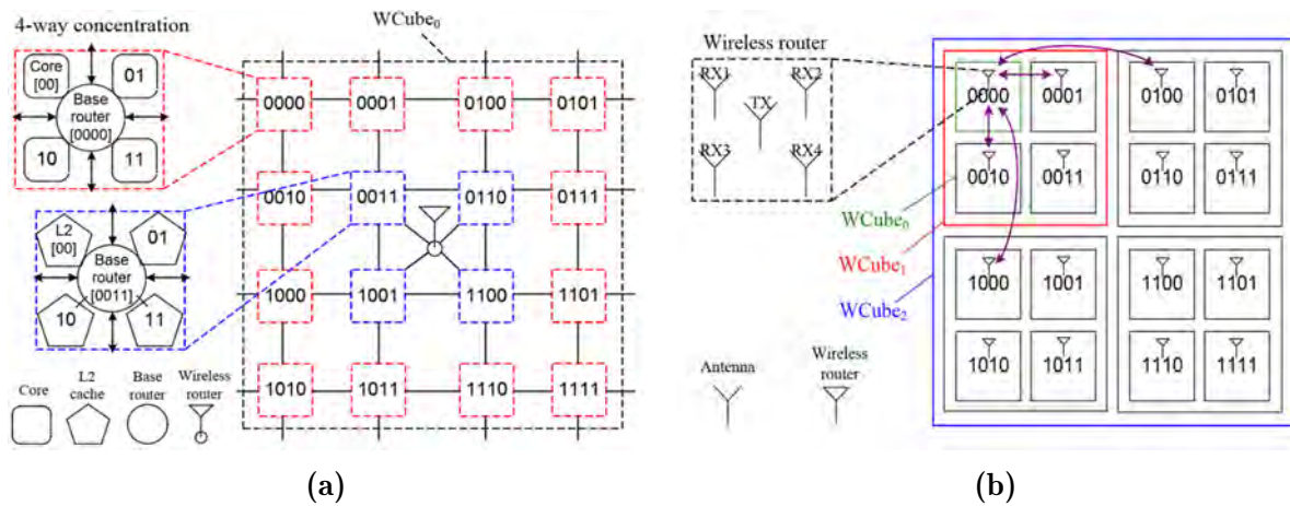
Figure 1.19: A WCube architecture [Lee+09]
