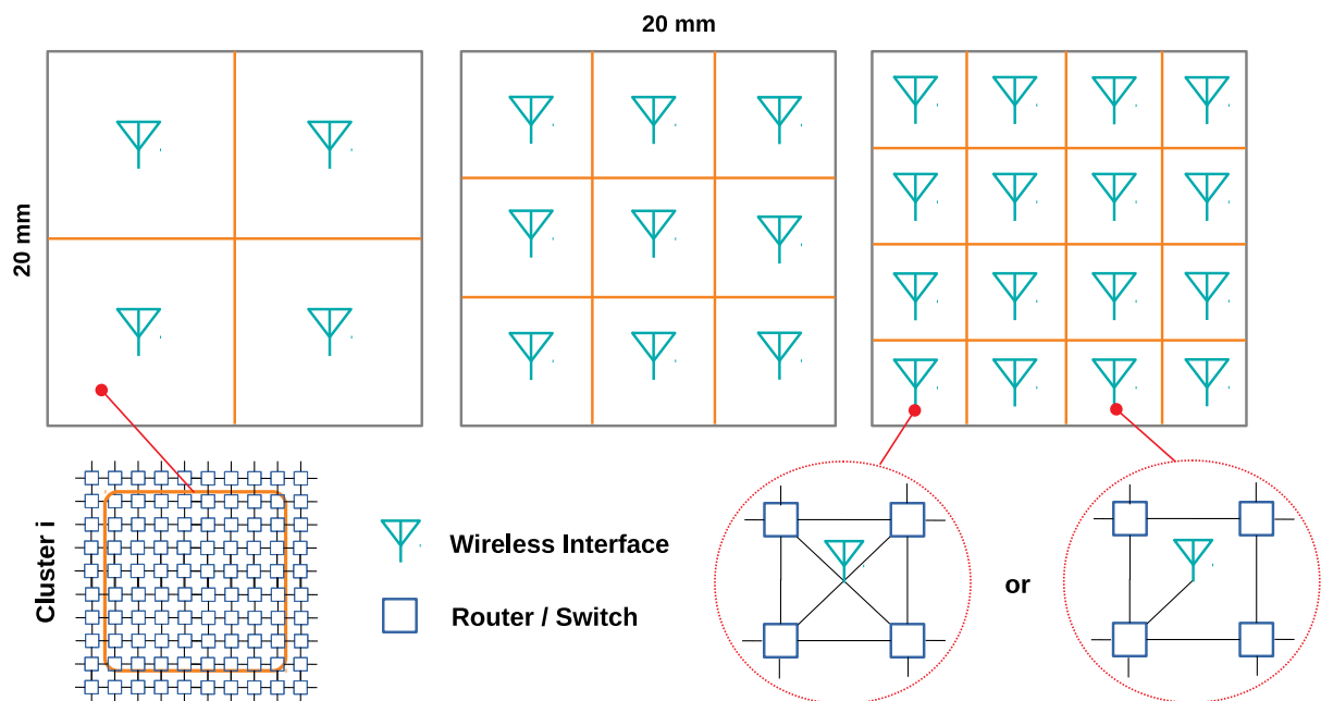
Figure 4.1: Wireless interface distribution among a clustered WiNoC hybrid topology with N clusters of M cores.
