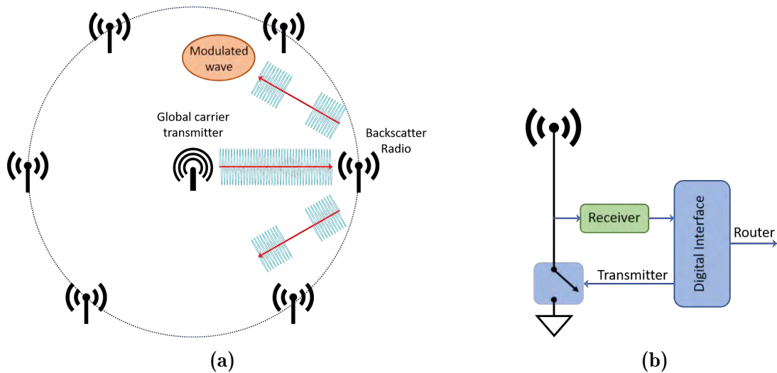
Figure 5.21: BackScattering WiNoC Communication.
