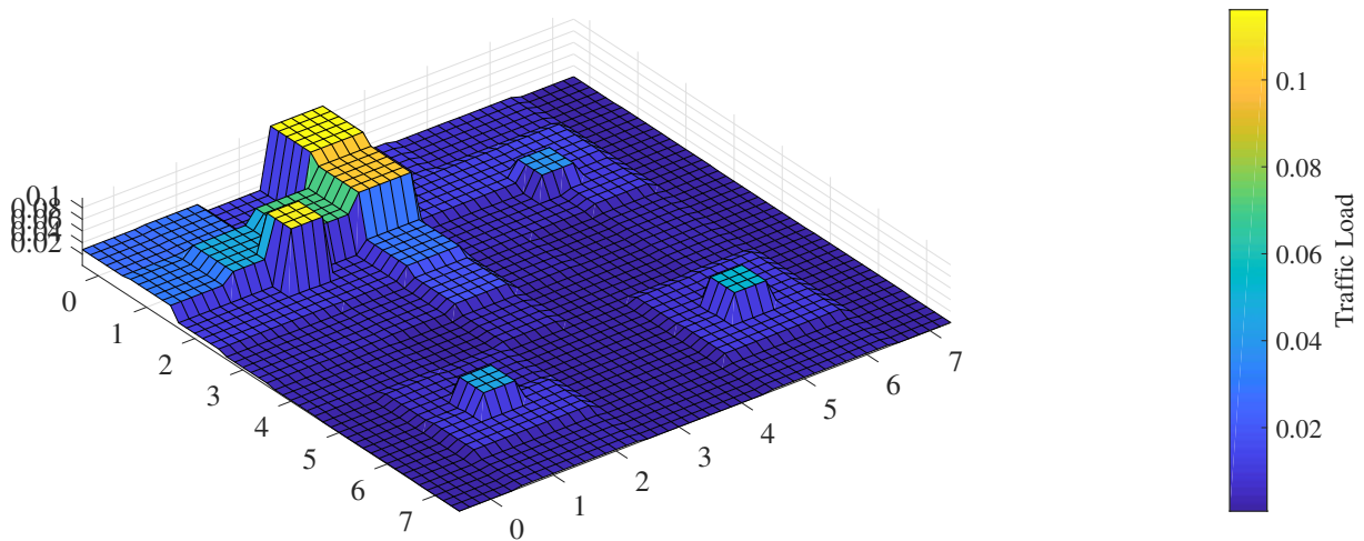
Figure 5.18: Network behaviour generated by application benchmark x264 into a 64-core WiNoC using 4 antennas rectangularly placed into the chip.
