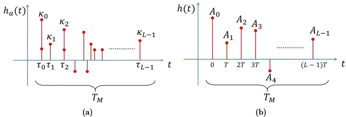
Figure 2.3: Representation of the multi-path channel impulse response
