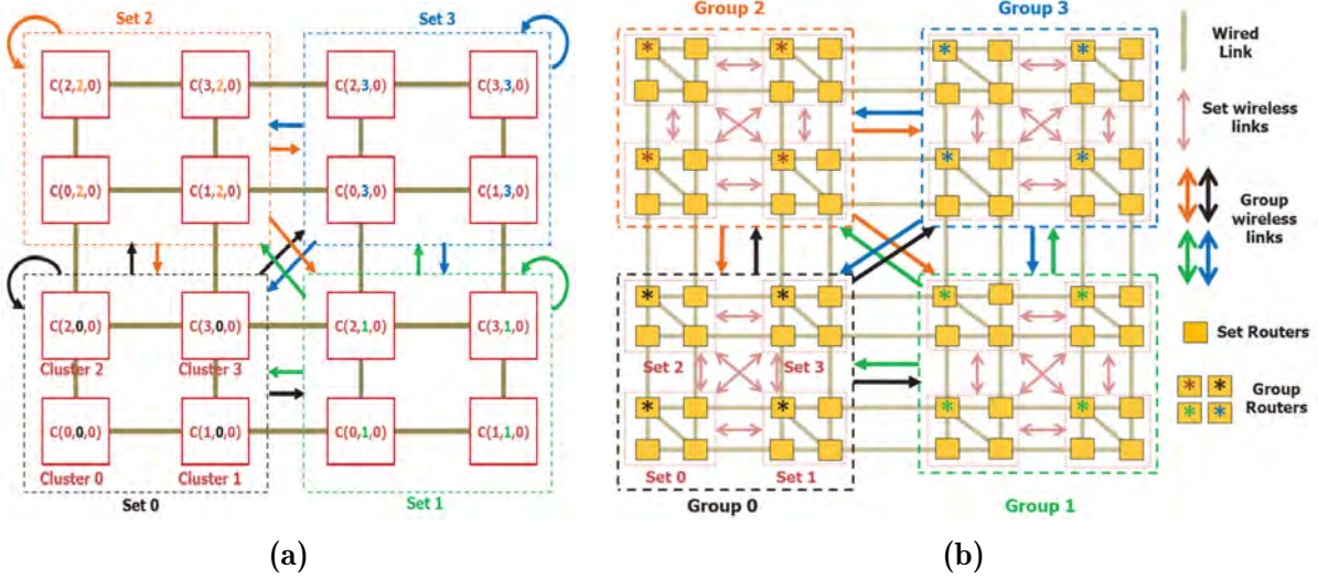
Figure 1.20: A iWISE architecture [Lee+09]
