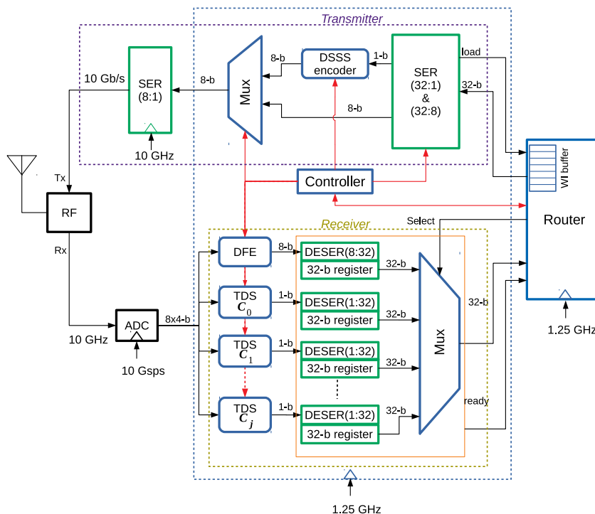
Figure 3.3: Enhanced digital-domain adaptive transceiver architecture.
