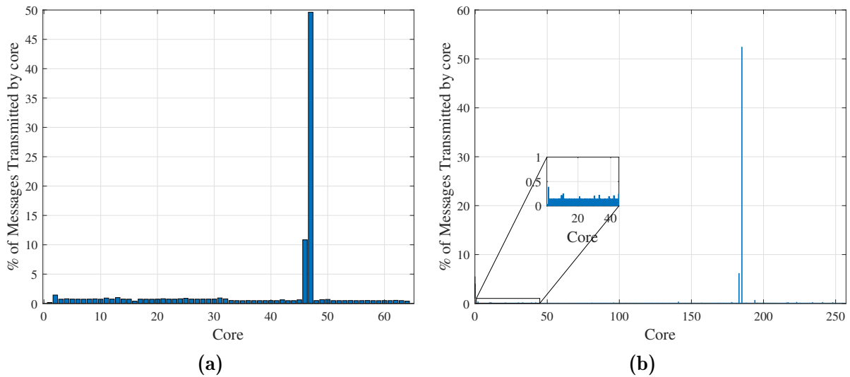
Figure 5.10: Message generated per core for the Streamcluster benchmark in a network of (a) 64 and (b) 256 cores.
