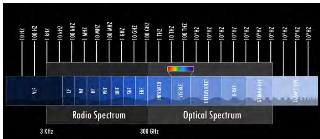
Figure 1.14: Range of frequencies in wireless communications.
