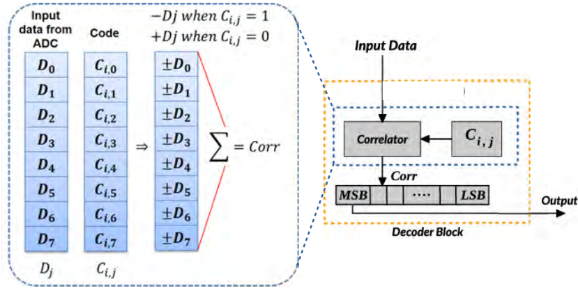
Figure 2.24: DSSS decoder architecture.
