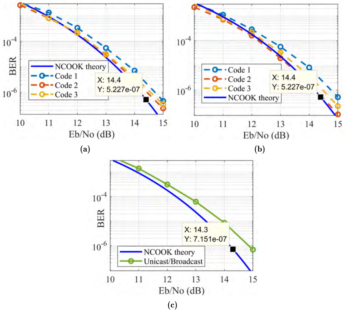
Figure 4.10: performance BER for multicast with (a) PG = 4 , (b) PG = 8 , and (c) unicast/broadcast.
