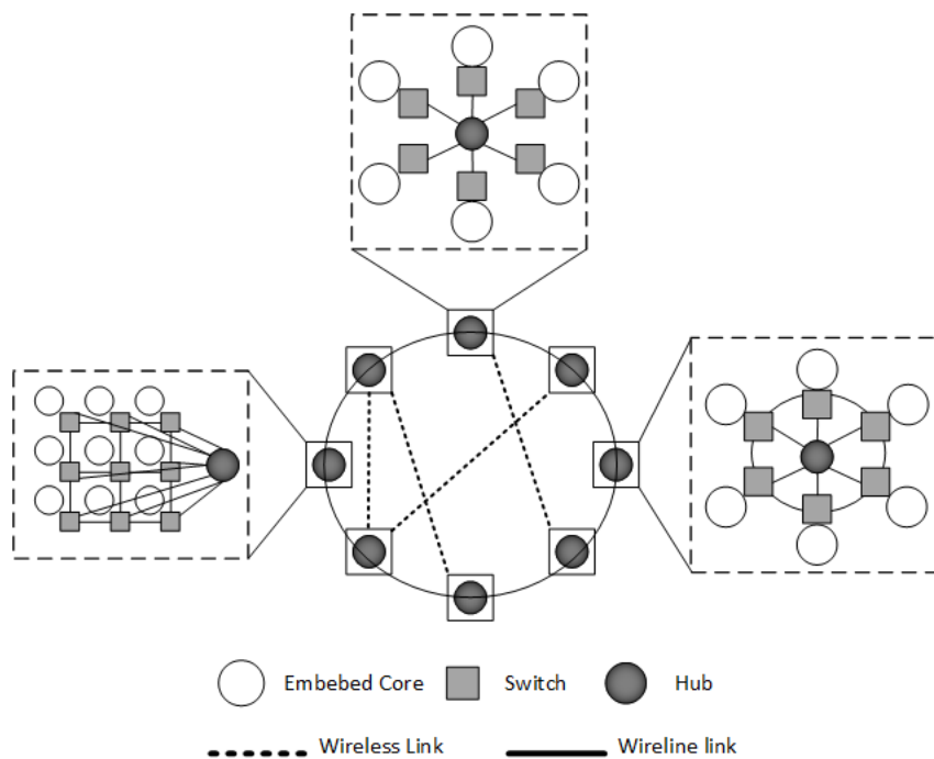
Figure 1.23: A hybrid (wireless/wired) hierarchical WiNoC architecture with heterogeneous subnets and small-world-based upper-level configuration [Cha+12].
