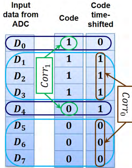
Figure 2.26: Time-diversity scheme optimization.
