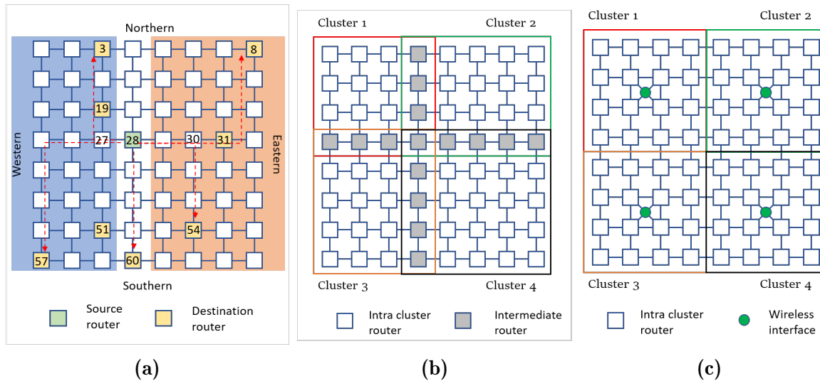
Figure 5.14: Multicasting techniques: (a) MDND, (b) VBON, and (c) WDN.
