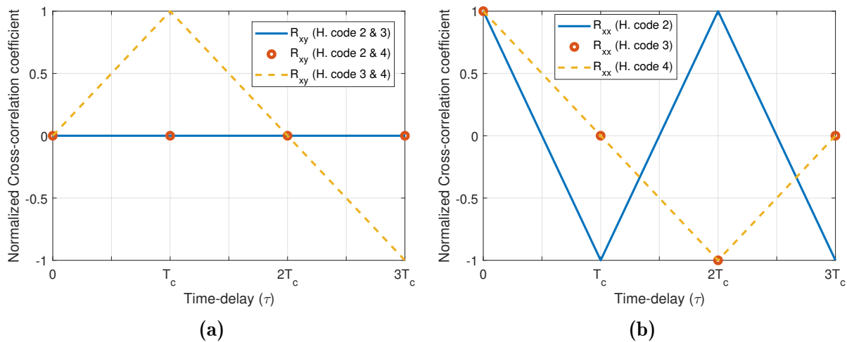
Figure 2.16: (a) Cross-correlation function between the codes contained into the Hadamard matrix H_4 , (b) autocorrelation function for each code contained in H_4 .
