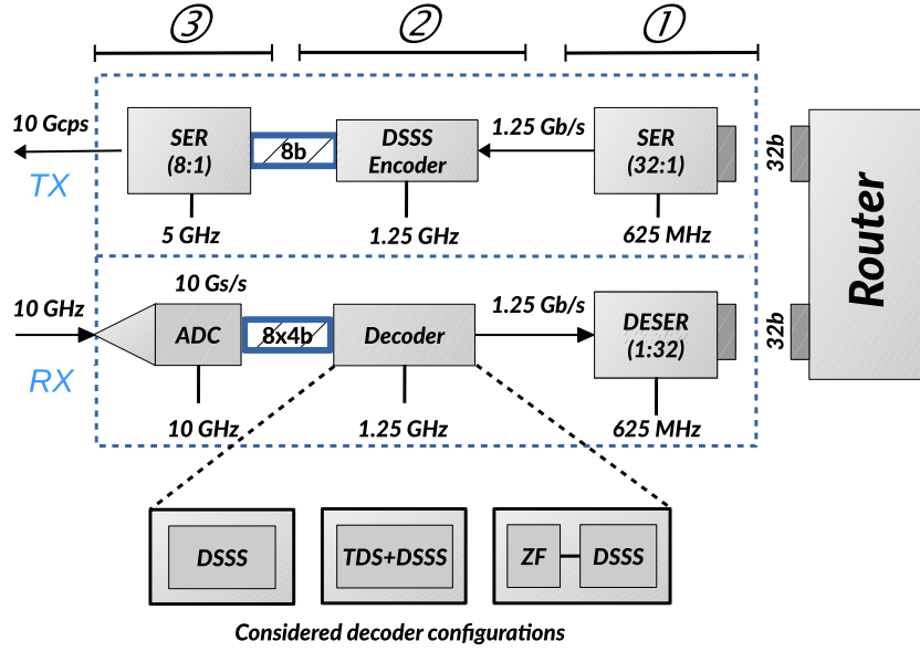
Figure 2.22: Enhanced digital-domain transceiver architecture with three decoder configurations.
