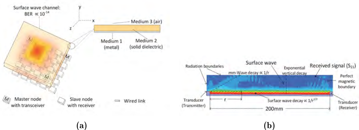
Figure 1.11: (a) Dielectric-coated metal surface, (b) SW propagation decay [Hen10]
