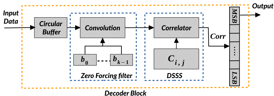
Figure 2.27: ZF equalizer with DSSS decoder architecture.
