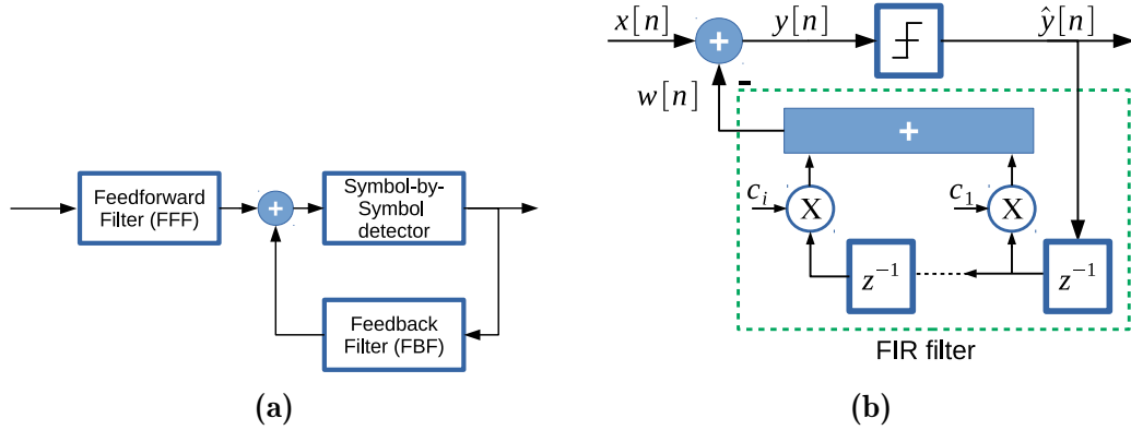
Figure 3.2: (a) General DFE structure, (b) Adopted DFE.
