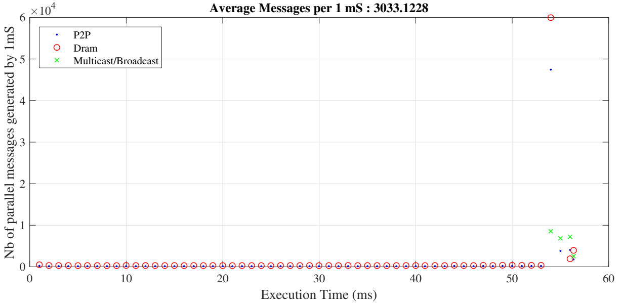
Figure 5.11: Temporal distribution of the different types of traffic (P2P, DRAM, Multicast/Broadcast) for the Blackscholes application.
