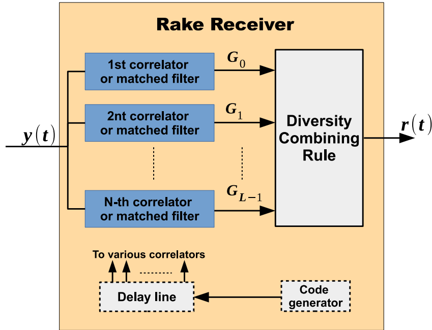
Figure 2.20: Diversity demodulator for spread-spectrum signals over multi-path channels.
