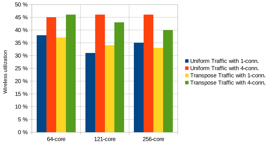
Figure 4.2: Wireless interface utilization using single and multiple router connections into a single WI.
