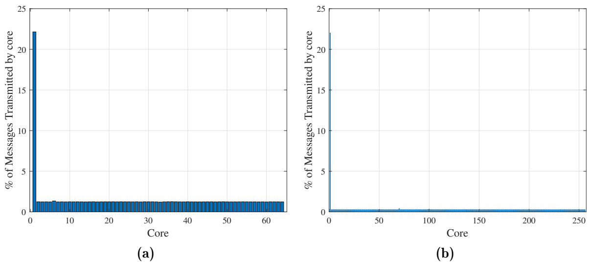
Figure 5.8: Message generated per core for the Raytrace benchmark in a network of (a) 64 and (b) 256 cores.
