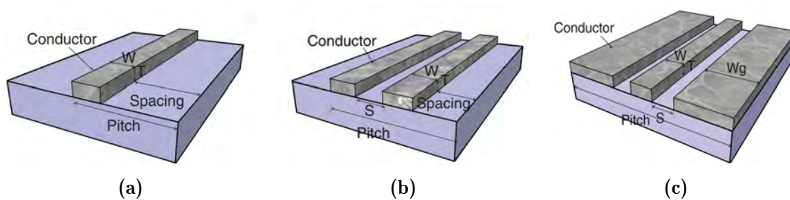
Figure 1.7: Three main types of on-chip TLs: (a) microstrip line (MSL), (b) differential line or coplanar strips (CPS), and (c) coplanar waveguide (CPW)
