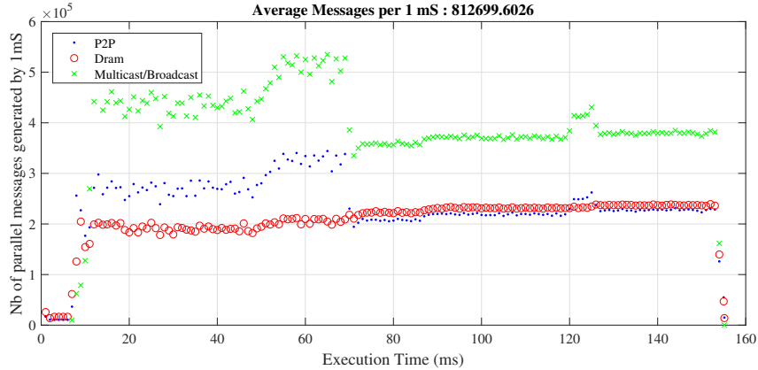
Figure 5.13: Temporal distribution of the different types of traffic (P2P, DRAM, Multicast/Broadcast) for the Streamcluster application.
