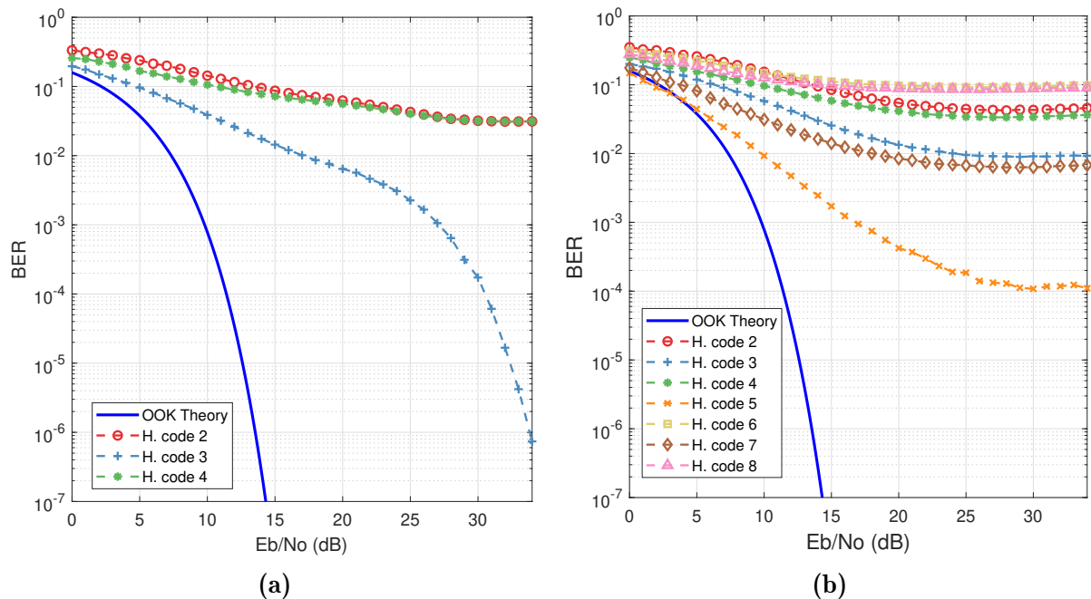
Figure 2.18: Performance evaluation for a set of (a) three Hadamard codes of length N = 4 and (b) seven Hadamard codes of length N = 8 , facing multi-path interference during full multiple-access channel.
