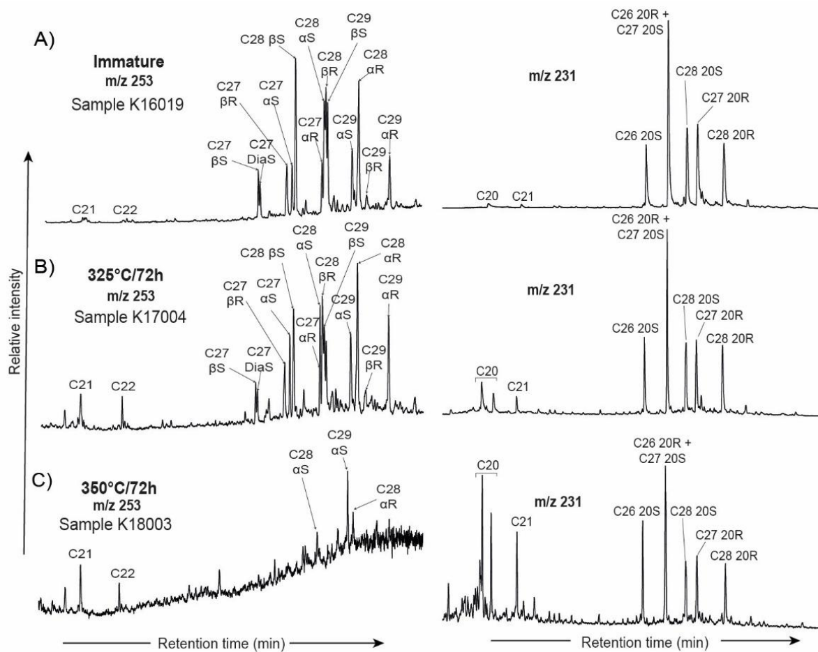
Fig. 5.13. Mass chromatograms showing the distribution of monoaromatic ( m/z 253) and triaromatic steroids ( m/z 231) in samples before (A) and after maturation at (B) 325^{\circ}\text{C} and (C) 350^{\circ}\text{C} for 72 hours.
