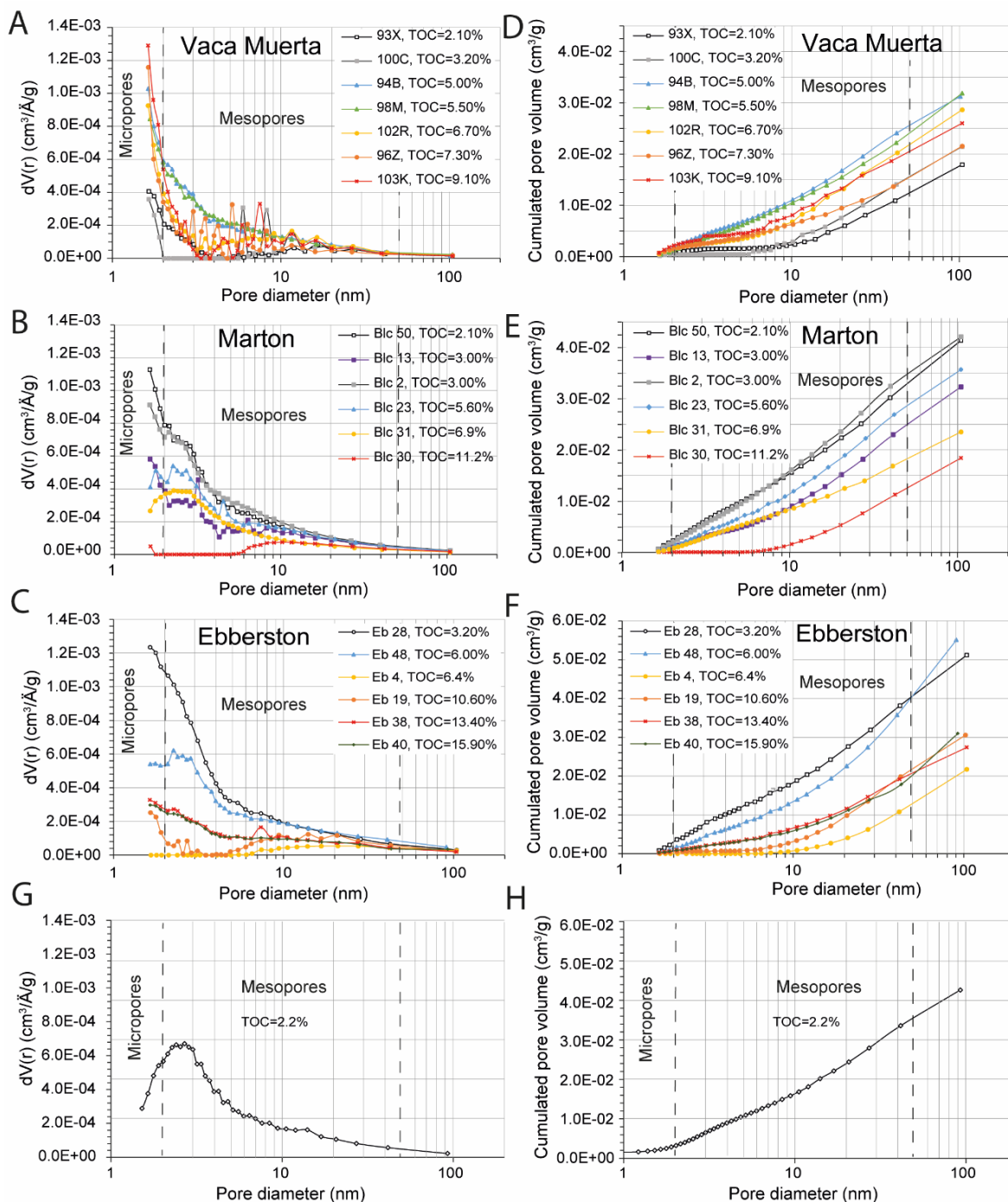
Fig. 4.15. Pore size distributions and cumulated pore volumes derived from the nitrogen adsorption branch for the isotherms of KCF (Marton, Ebberston, Viking graben) and VMF mudstones (BJH model) as a function of TOC (in weight %).
