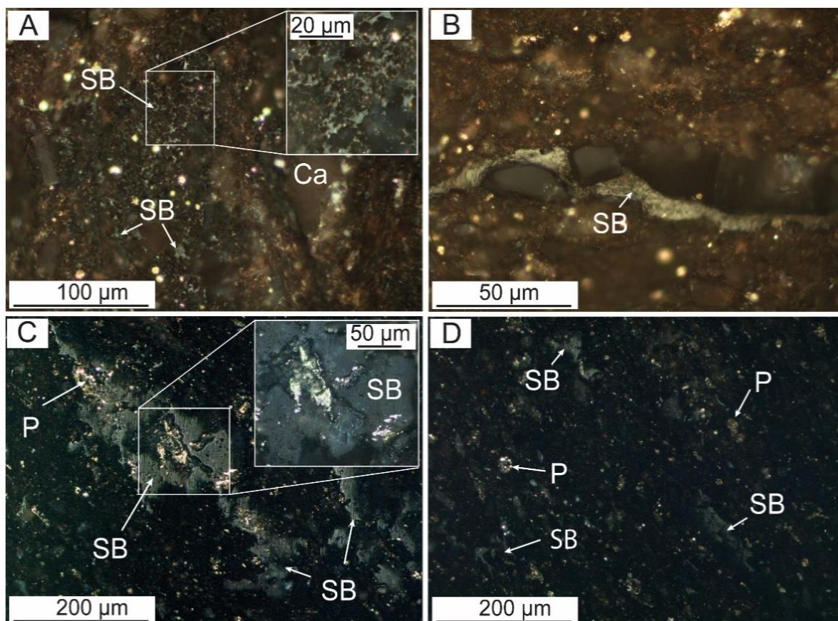
Fig. 4.5. Incident white light photomicrographs of VMF mudstones (~1.65%, TOC = 5.0 wt.%). A) Solid bitumen/pyrobitumen (SB) network. Insert in A shows solid bitumen embayed against small euhedral crystals of carbonates. B) Solid bitumen streak (grey-white). C-D) Pyrobitumen accumulations with a granular/pitted surface texture. P: pyrite. Ca: carbonate.
