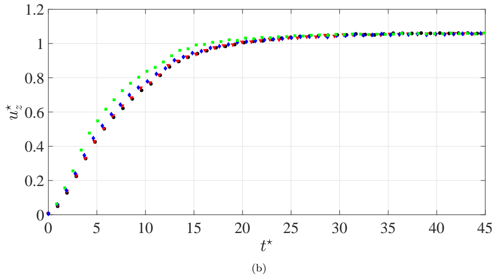
Figure 6.14 – Instantaneous vertical velocity u_z^* for all the analysed coatings, for the tests with Re_\infty in the range 100 – 110. (a), d = 10 mm spheres in the W020\_G080 mixture. (b), d = 5 mm spheres in the W030\_G070 mixture. \bullet , reference. \blacktriangledown , SH-NAR. \blacklozenge , SH-220. \blacksquare , SH-80.
