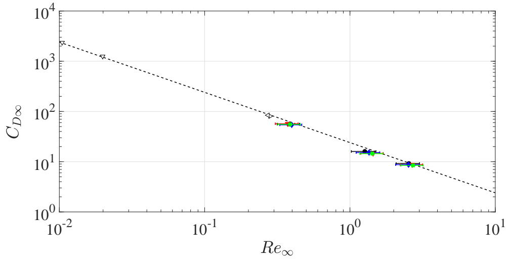
Figure 6.6 – Terminal drag coefficient C_{D\infty} as a function of the terminal Reynolds number Re_{\infty} for the glycerine tests. \bullet , reference. \blacktriangledown , SH-NAR. \blacklozenge , SH-220. \blacksquare , SH-80. \nabla , SH spheres by Byon et al. (2010). \triangleright , reference sphere by Ahmmed et al. (2016). \triangleleft , SH sphere by Ahmmed et al. (2016). The vertical error bars (95% confidence level) are of the same order of the size of the symbols. The horizontal error bars were estimated via the \mu_l uncertainty discussion related to Fig. 6.4. (---), Stokes' law C_{D\infty} = \frac{24}{Re_{\infty}} .
