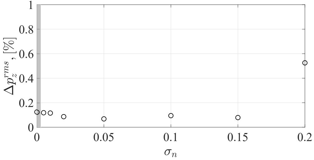
Figure 5.13 – Variation of the root-mean-square error \Delta p_z^{rms} (see Eq. 5.8) on the estimation of the instantaneous sphere position for increasing variance \sigma_n of the Gaussian noise applied to the artificially generated images ( d = 10 mm reference stainless steel sphere falling in pure water (W100_G000)). The accuracy of the method is almost unaffected by the noise for \sigma_n values typical of the experimentally recorded images ( \approx 2 \times 10^{-3} , as highlighted by the gray-shaded region).
