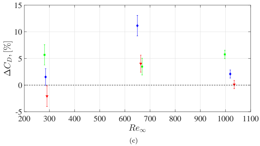
Figure F.6 – Terminal drag variation \Delta C_D for all the analysed coatings and mixtures. (a), W020_G080. (b), W030_G070. (c), W040_G060. The error bars represent the 95% confidence level. (---), reference value \Delta C_D = 0 indicating the limit between drag increase ( \Delta C_D > 0 ) and decrease ( \Delta C_D < 0 ) (see the \Delta C_D definition in Eq. 6.3).
