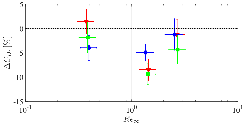
Figure 6.7 – Variation of the terminal drag coefficient as a function of the terminal Reynolds number Re_{\infty} for the glycerine tests. \blacktriangledown , SH-NAR. \blacklozenge , SH-220. \blacksquare , SH-80. The error bars represent the 95% confidence level. (---), reference value \Delta C_D = 0 indicating the limit between drag increase ( \Delta C_D > 0 ) and decrease ( \Delta C_D < 0 ) (see the \Delta C_D definition in Eq. 6.3).
