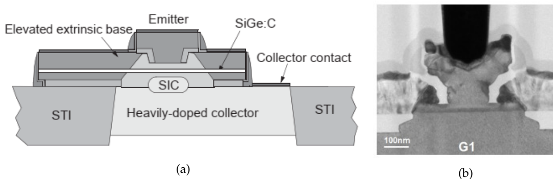
Figure 1.20: (a) Schematic [64] and (b) TEM cross-section [62] for a high-speed transistor from SG13S technology.
