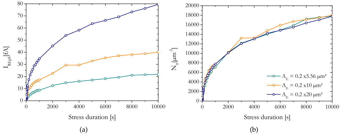
Figure 3.23: (a) Extracted I_{REpS} parameter and (b) Calculated N_T following equation (3.8) from Gummel measurements for a stress condition of V_{CB} = 2.4 V and J_E = 231 \mu A/\mu m^2 and for three B55 technology devices from ST Microelectronics.
