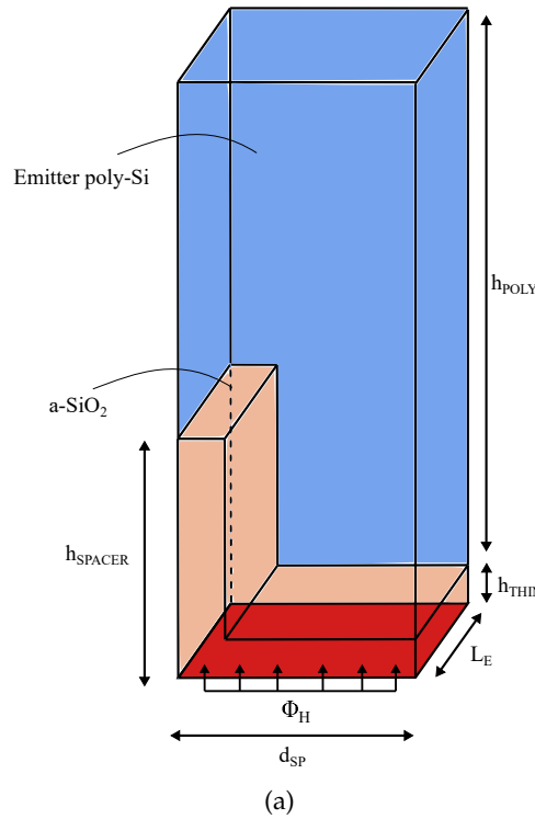
Figure 3.24: Schematic of the hydrogen diffusion volume taking into account the E-B spacer oxide and the emitter poly-Si thickness for B55 technology from ST Microelectronics.
