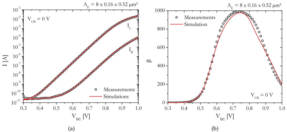
Figure 2.1: Comparison between measurements (symbols) and HiCuM/L2 simulation v2.34 (solid lines) for (a) the forward Gummel characteristic and (b) the current gain at V_{CB} = 0 \text{ V} on a 8 \times 0.16 \times 0.52 \mu\text{m}^2 device corresponding to SG13S technology from IHP Microelectronics.
