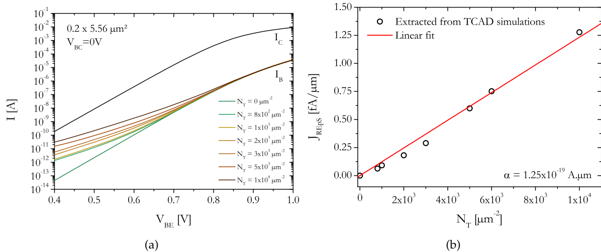
Figure 3.8: (a) TCAD simulation results for various trap densities and (b) corresponding J_{REPS} evolution allowing to extract the proportionality coefficient \alpha representative of the relationship between the density of defects at the interface and the base recombination current density value on a B55 technology from ST Microelectronics .
