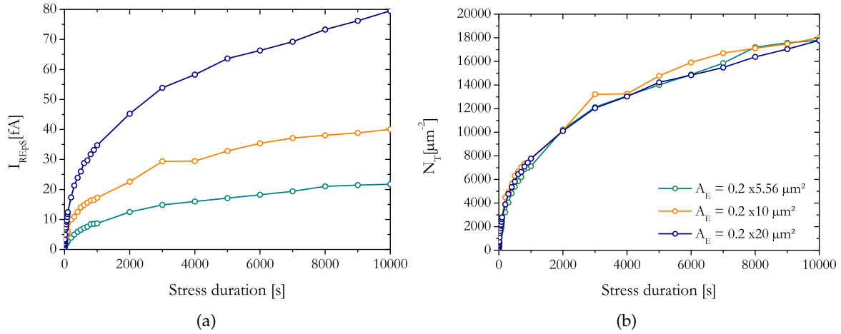
Figure 3.23: (a) Extracted I_{REPS} parameter and (b) Calculated N_T following equation (3.8) from Gummel measurements for a stress condition of V_{CB} = 2.4 V and J_E = 231 \mu A/\mu m^2 and for three B55 technology devices from ST Microelectronics.
