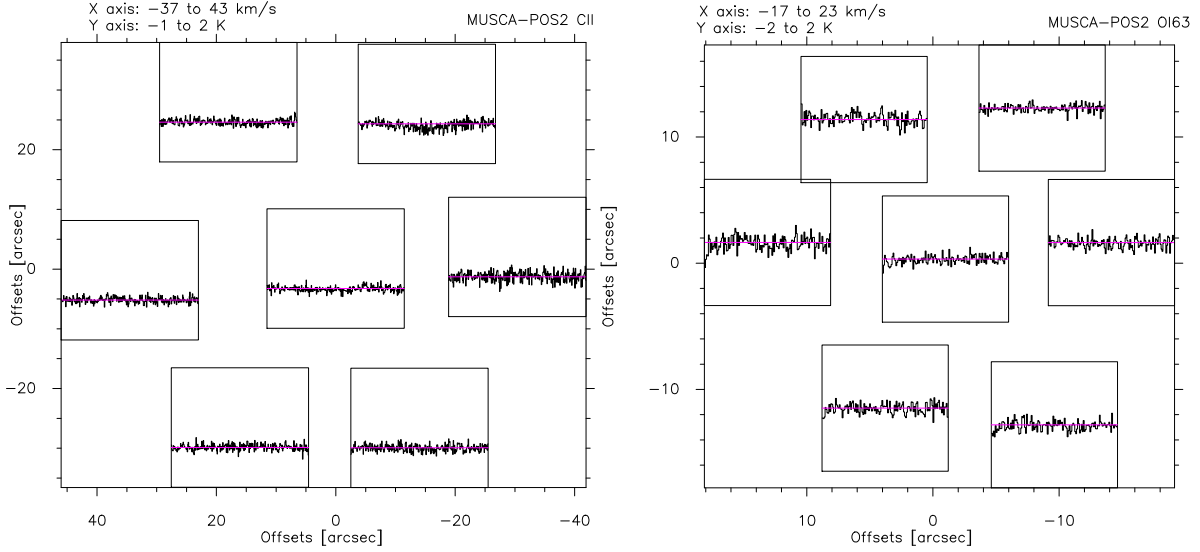
Fig. A.1. Left: observed pixels for the [C II] 158 \mu\text{m} line with the SOFIA telescope with a spectral resolution of 0.3 km s -1 . Right: observed pixels for the [O I] 63 \mu\text{m} line.
