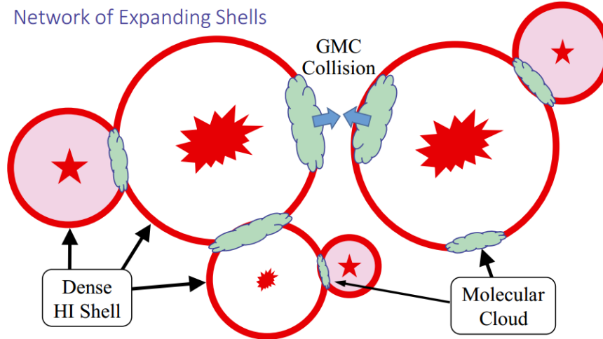
Figure 5.14: A schematic representation of the scenario described in Inutsuka et al. (2015). Molecular clouds generally form at the intersection of expanding bubbles, with a GMC collision leading to extremely active star formation as is observed for example in Cygnus-X north.
