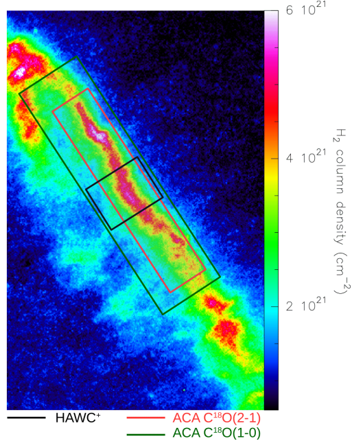
Figure 4.8: The Herschel column density map of the central part of the Musca filament (Cox et al., 2016). The red and green rectangles indicate the regions that will be mapped with the ALMA Compact Array (ACA) in C^{18}O(2-1) and C^{18}O(1-0) , respectively. The black rectangle shows the region that was observed with the polarimetric HAWC + receiver on SOFIA (PI: J. Soler).
