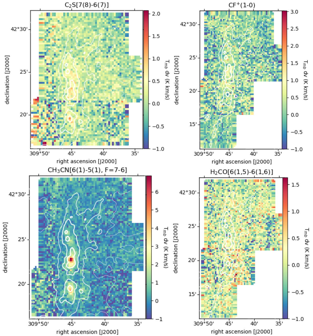
Figure A.1: Top left: The integrated intensity map of C_2S[7(8)-6(7)] , with Herschel column density contours at N_{H_2} = 10^{22} , 3 \cdot 10^{22} , 10^{23} and 5 \cdot 10^{23} \text{ cm}^{-2} . Top right: The same for CF^+(1-0) . Bottom left: The same for CH_3CN[6(1)-5(1), F=7-6] . Bottom right: The same for H_2CO[6(1,5)-6(1,6)] .
