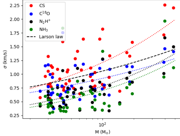
Figure 6.7: The fitted linewidth for CS(2-1), C 18 O(1-0), N 2 H + (1-0) and NH 3 as a function of the core mass. The black dashed line gives the evolution of the Larson law (Larson, 1981). The dotted lines show the fit \sigma \propto M^\alpha for each molecular line. It is observed that C 18 O(1-0) follows the Larson evolution, while the other lines do not.
