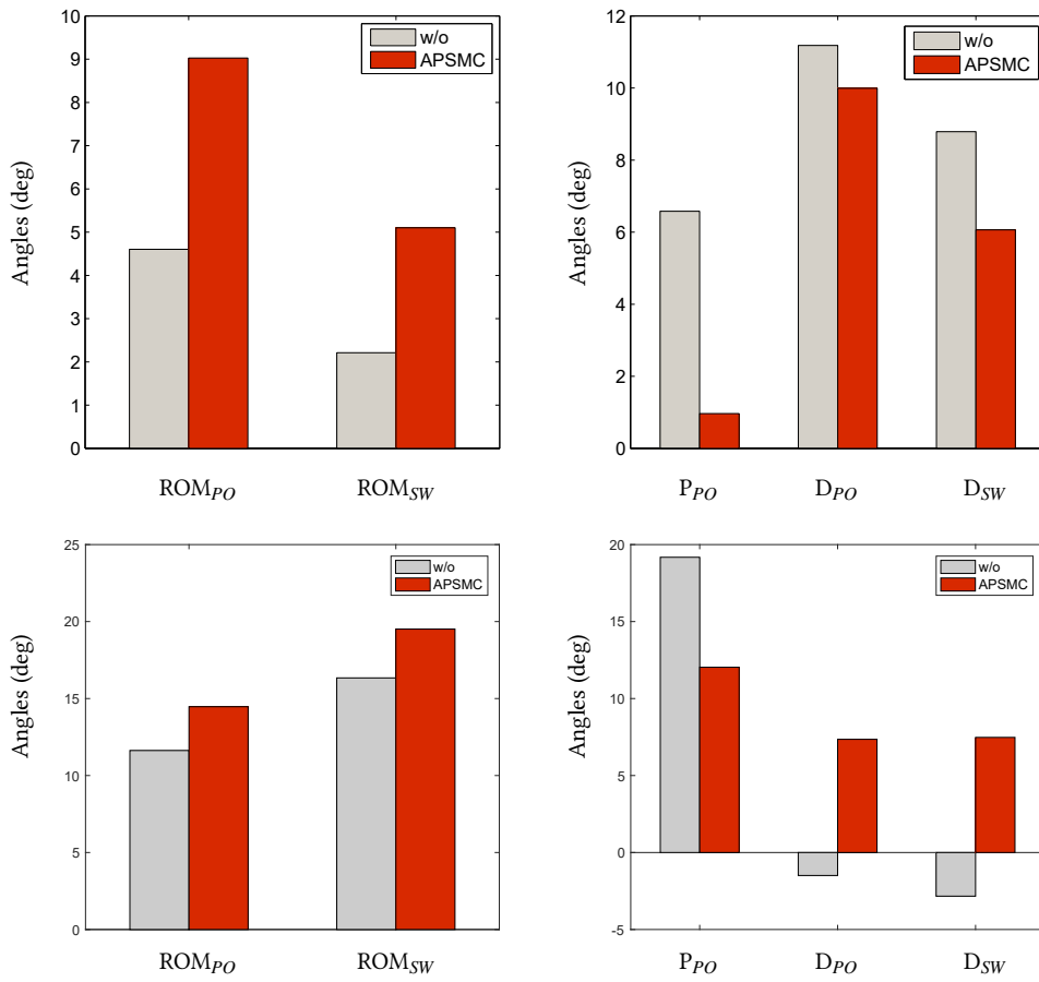
Figure 7.30 – The changes of the main walking kinematic features of the paretic patients from the condition “without assistance (w/o)” to the condition “with assistance (APSMC)”. ( P PO : Push off moment; S W : Swing phase, ROM: Range of Motion, P: Planter flexion, D: Dorsiflexion)
