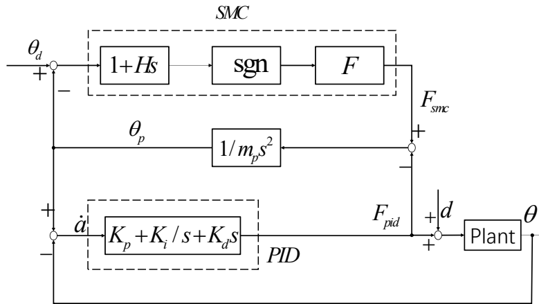
Figure 5.2 – Principal of PSMC.
