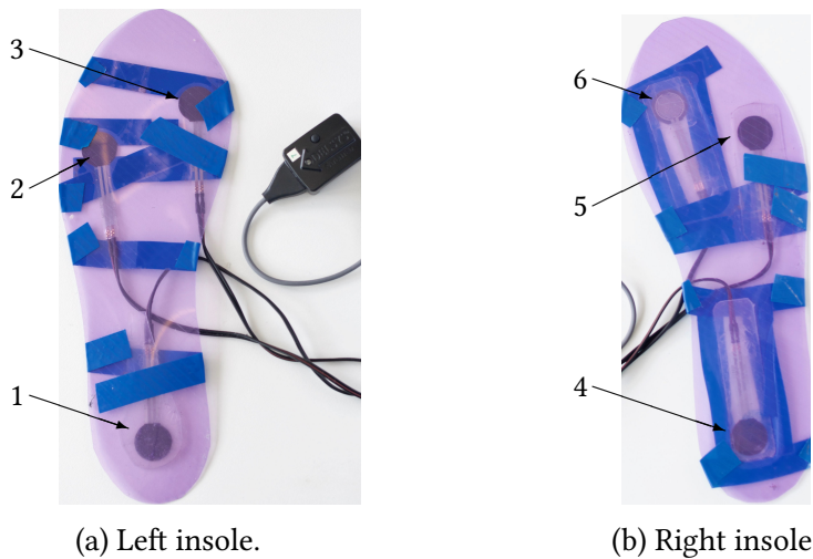
Figure 3.4 – The insoles with the force sensitive resistors.
