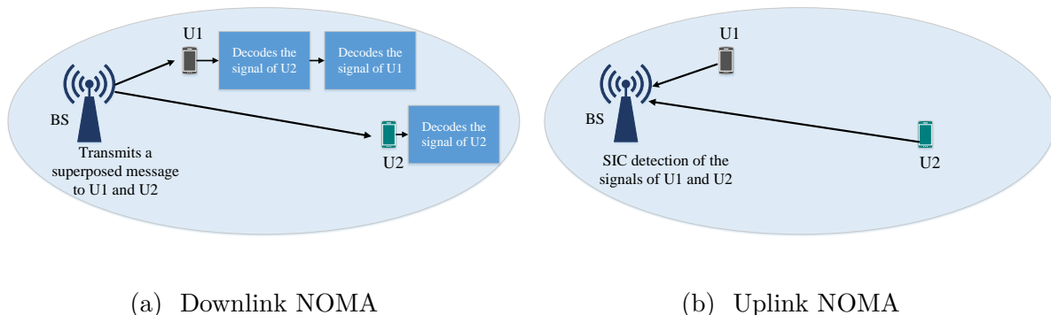
Figure 2.3 – SIC decoding
