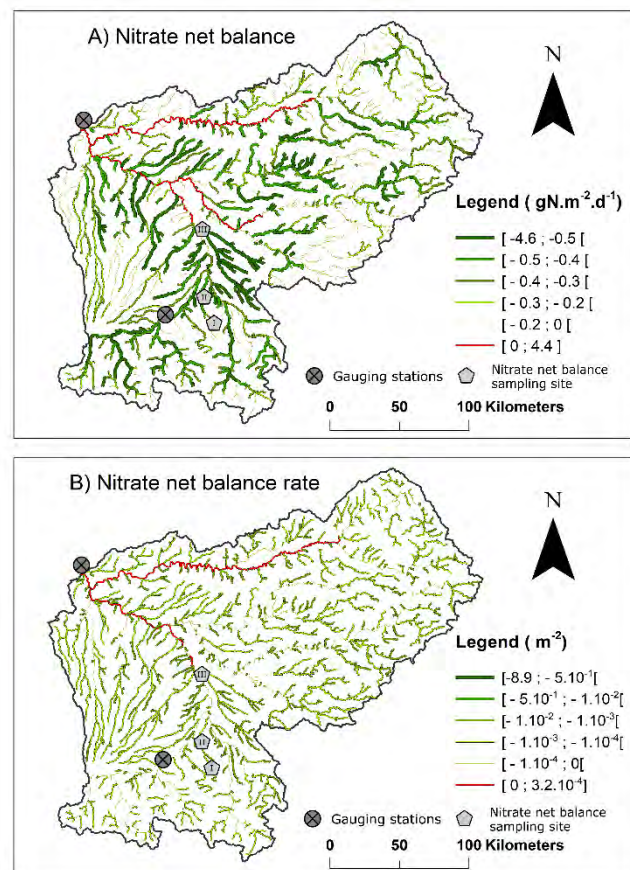
Figure 34: The inter-annual monthly average simulation of (A) Nitrate Net Balance, NNB, by reaches over Garonne watershed in \text{gN} \cdot \text{m}^{-2} \cdot \text{d}^{-1} ; (B) Nitrate Net Balance Rate, NNBR, by reaches over Garonne watershed in \text{m}^{-2} ; and localization of NNB sampling sites (I: Montegut, II: Lézat, III: Downstream of Toulouse) and two gauging stations (Tonneins at the outlet and Roquefort at Salat)
