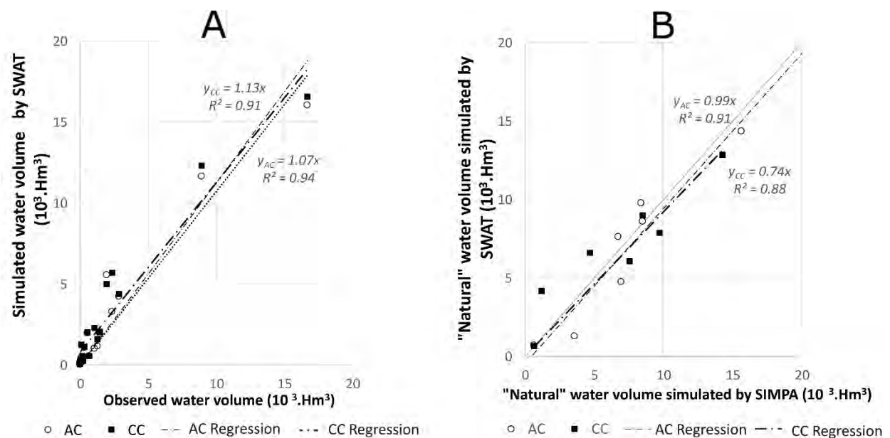
Figure 55: Simulated CC (Conventional Calibration) and AC (Additional Calibration) versus (A) observed annual water volume and versus (B) SIMPA simulation for the main watersheds of the SUDOE territory (inter-annual averages from 2000 to 2010).
