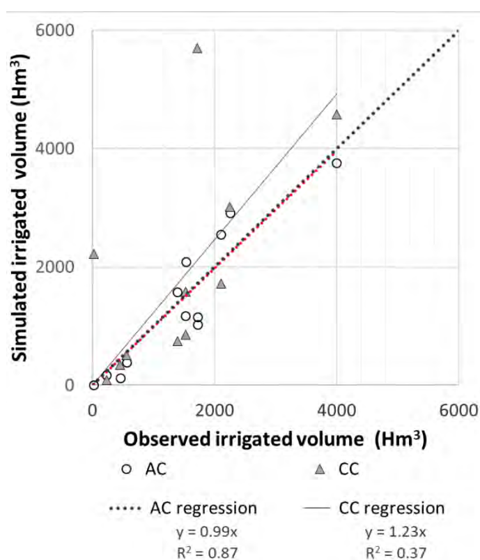
Figure 54: Simulated AC versus observed annual water volume ( \text{Hm}^3 ) used in irrigation for each Spanish region (inter-annual averages from 2000 to 2010).
