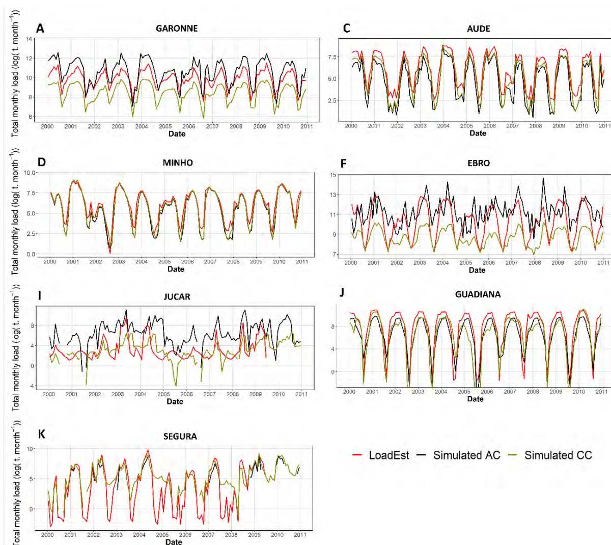
Figure 58: Monthly variation of sediment loads from 2000 to 2010 (calibration period: 2000 -2005, validation period: 2006 -2010) obtained with LOADEST and SWAT calibrations in the main SUDOUE watersheds (AC: Additional Calibration; CC: Conventional Calibration). The letters indicate the watershed localization over SUDOUE territory (Figure 51).
