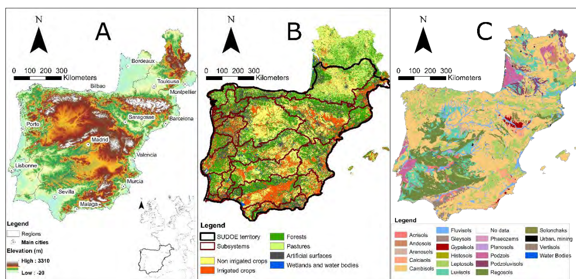
Figure 50: SUDOE study area characteristics (A) Topography, main cities and regions ; (B) Land use and subsystems ; (C) Pedology.
