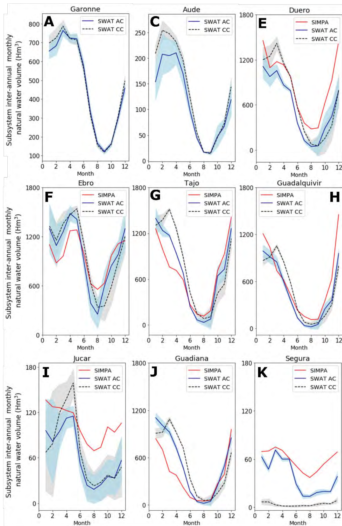
Figure 57: Inter-annual monthly dynamics of "natural" water volumes in the main SUDOUE watersheds simulated with SIMPA (red line), SWAT Additional Calibration (SWAT AC, blue line) and SWAT Conventional Calibration (SWAT CC, dotted dark line). The color ribbons (blue for AC and gray for CC) show the 95% prediction uncertainty intervals resulting from the best SWAT-CUP simulation. The letters indicate the watershed localization over SUDOUE territory (Figure 51) (inter-annual averages from 2000 to 2010). There is no SIMPA simulation for Garonne and Aude watersheds.
