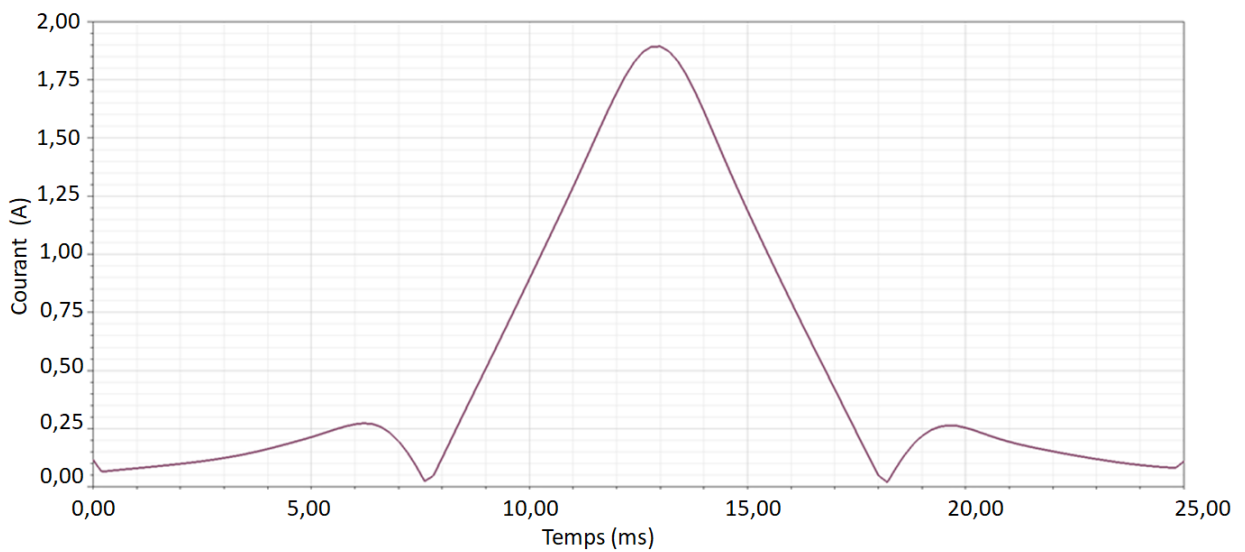
Figure II.66 – Courant secondaire MCPM.
