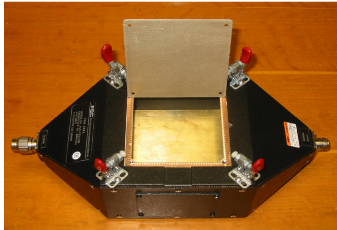
Figure I.38 – Cellule TEM Fcc-jm2 DC - 2 GHz [73].
