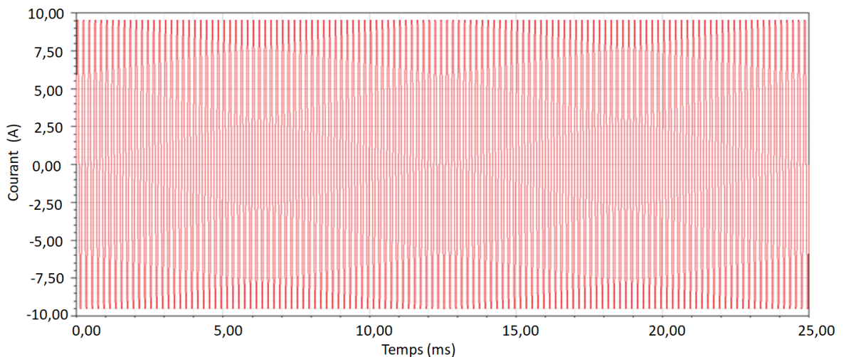
Figure II.63 – Courant primaire MCP.
