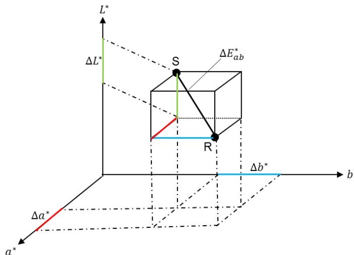
Figure 3-17: Representation of the cartesian coordinate differences between a reference (R) and a sample (S) adapted from (Chrisment et al., 1994)
