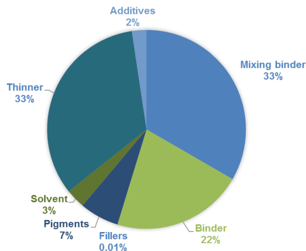
Figure 4-3: Proportions of the different components in the basecoat formula
