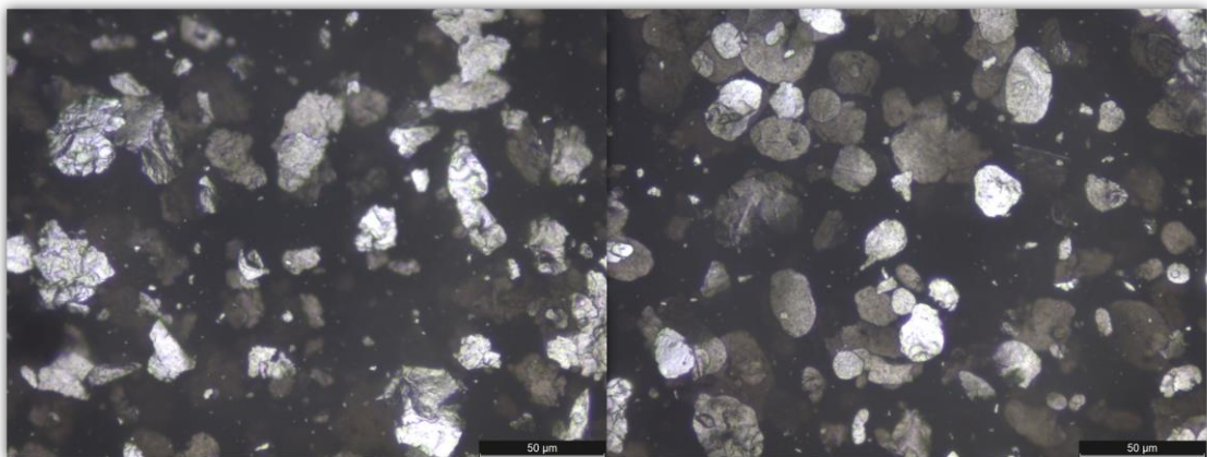
Figure 4-6: Light microscopy images of two letdowns, scale indicating 50 µm. Left: cornflake aluminum tinting base mixed with black tinting base. Right: silver dollar aluminum tinting base mixed with black tinting base
