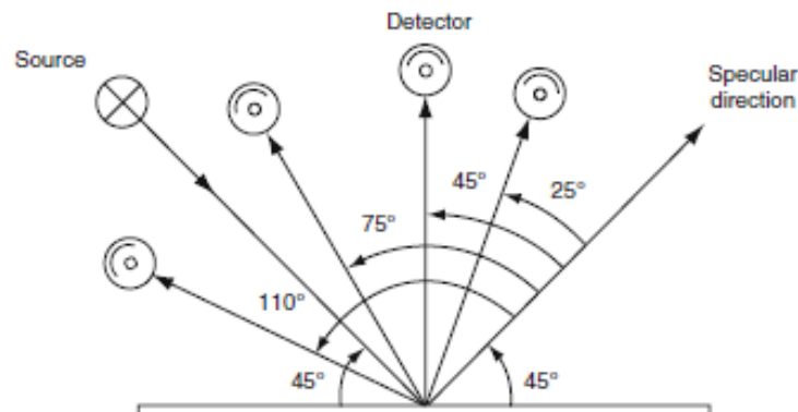
Figure 4-14: Principle of a multi-angle spectrophotometer from (Klein, 2010b)
