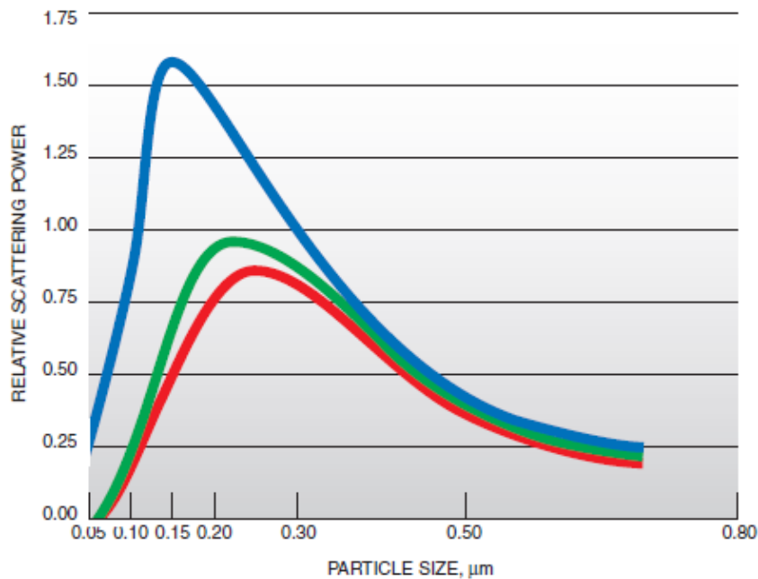
Figure 4-5: Relative light scattering power of rutile \text{TiO}_2 for blue, red and green light as function of \text{TiO}_2 particle size from (DuPont TM , 2007)
