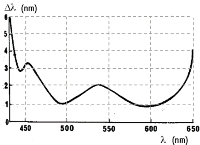
Figure 3-9: Wright and Pitt experiments on wavelength differences adapted from (Wyszecki and Stiles, 1982e)
