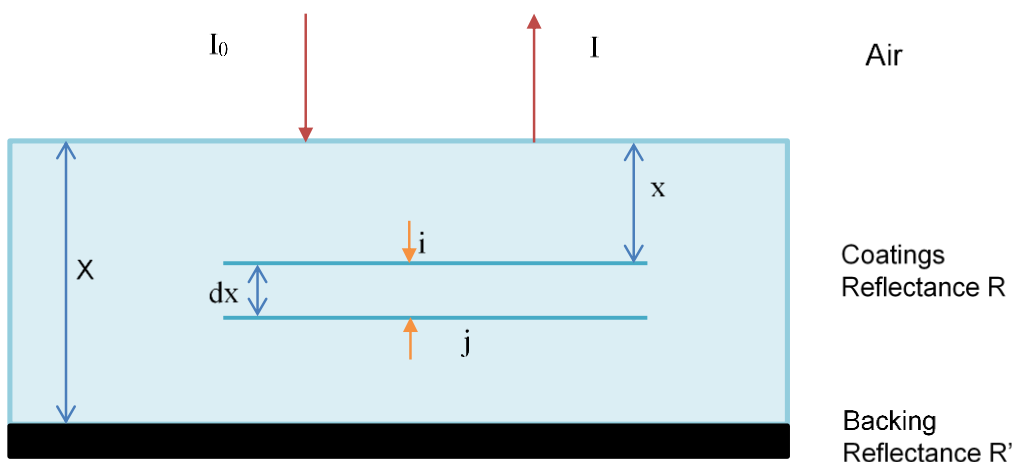
Figure 2-11 : Schematic diagram of light traveling in a colorant layer inspired from (Geniet, 2013)
