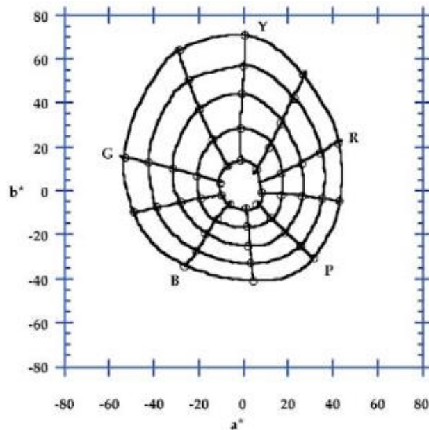
Figure 3-14: Munsell colors of chroma and hue at value 5 plotted in the CIELab a^*b^* plane from (Fairchild, 2013a)
