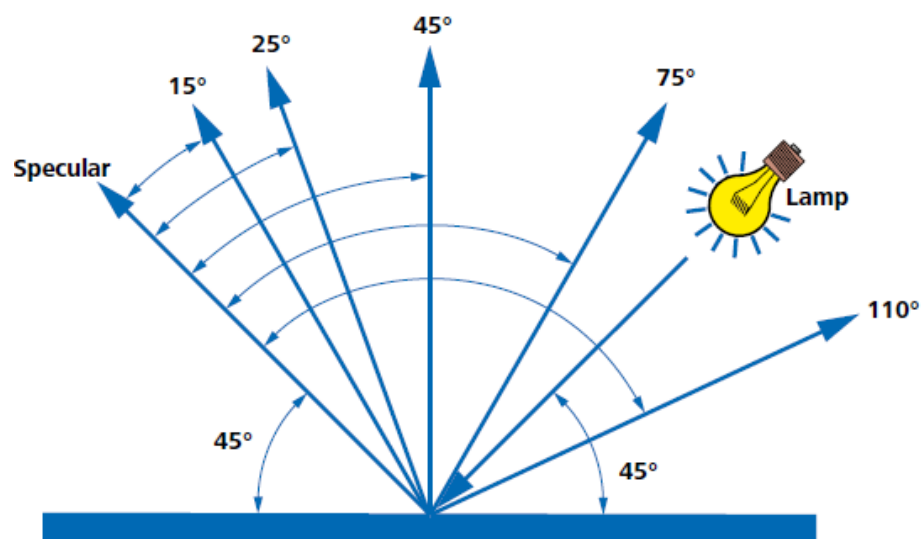
Figure 4-18: Color measurement geometries for the BYK Mac ( -15^\circ is not drawn) from (BYK.Gardner.GMBH, 2009)
