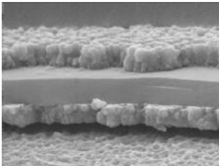
Figure 4-7: SEM 1 picture of a cross-section through a mica-based particle with a single layer of titanium dioxide from (Pfaff, 2009)
