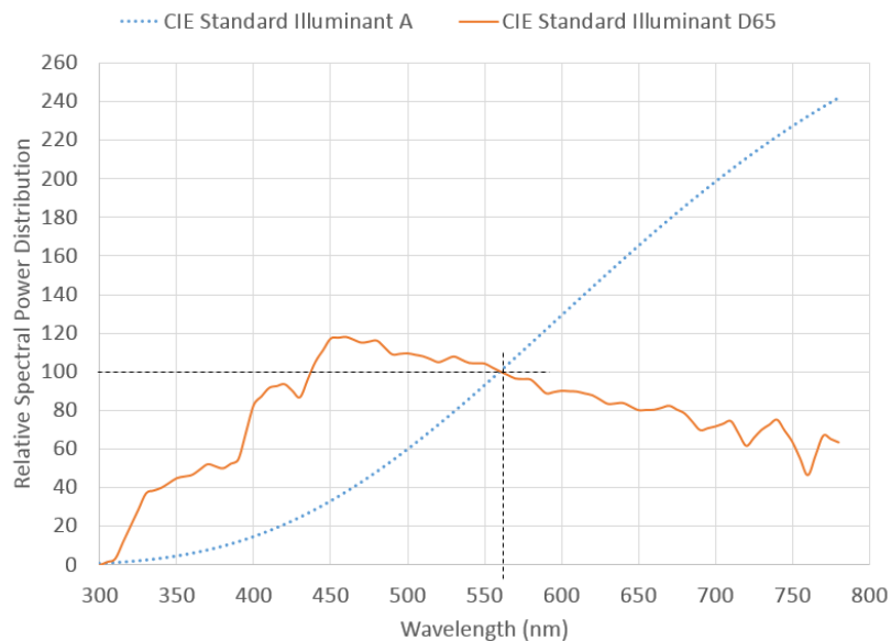
Figure 3-2: Relative spectral power distribution of the CIE standard illuminants A (in blue) and D_{65} (in orange) standardized to 100 at a wavelength of 560nm adapted from (Fairchild, 2013b)
