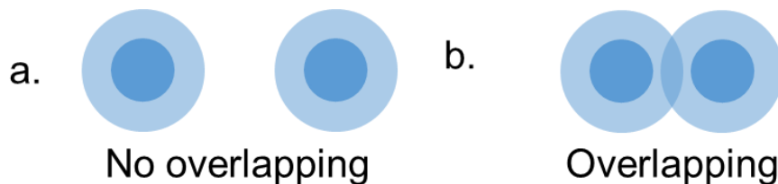
Figure 2-10: Loss of scattering due to particle scattering volumes overlapping
