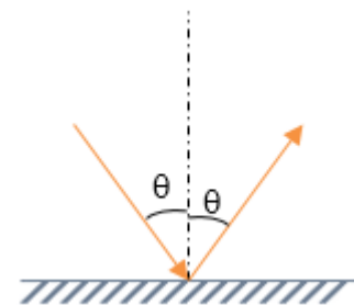
Figure 2-6: Light reflection adapted from (Klein, 2010)
