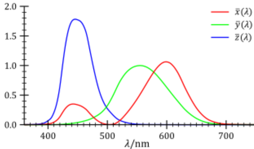
Figure 3-4: Standard color matching functions for the CIE 1931 XYZ system adapted from (Fairchild, 2013b)
