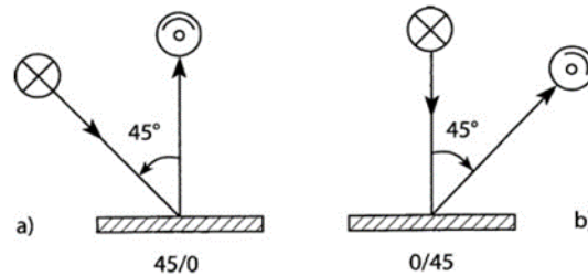
Figure 4-12: Directional measuring geometries: a) 45:0 and b) 0:45 from (Klein, 2010b)
