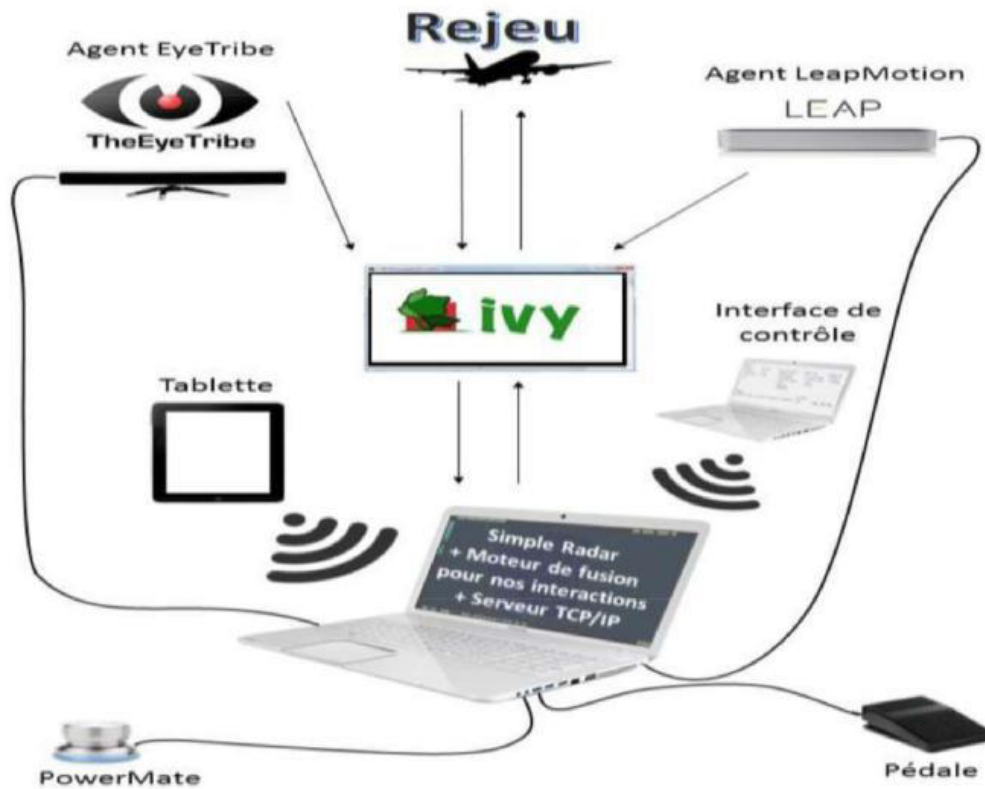
FIGURE 3.5: The architecture of the prototype
