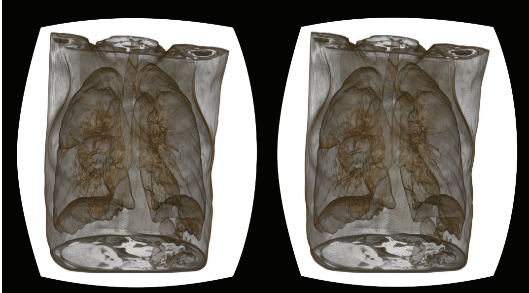
FIGURE 5.5: A lung CT scan rendered on the oculus rift using a CUDA accelerated raycasting algorithm
