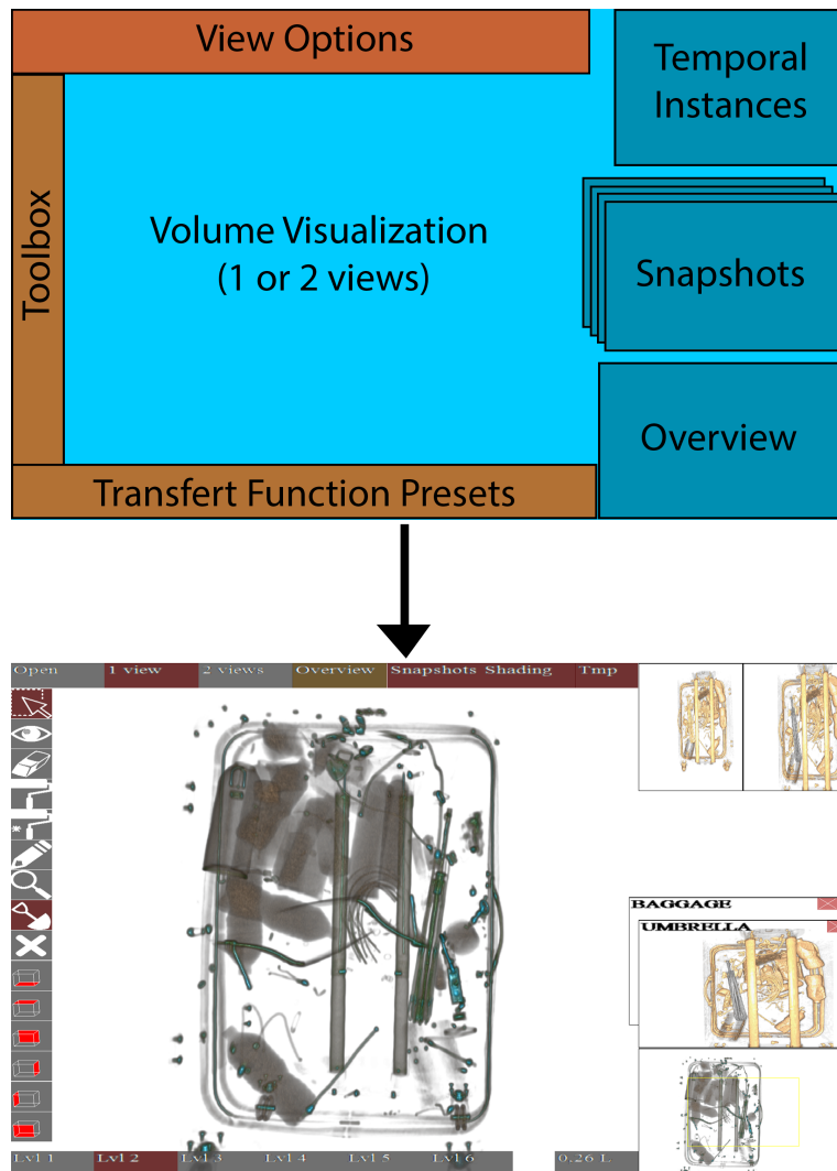
FIGURE 3.19: Top level layout and screenshot of our Graphical User Interface. All the features are available through this GUI
