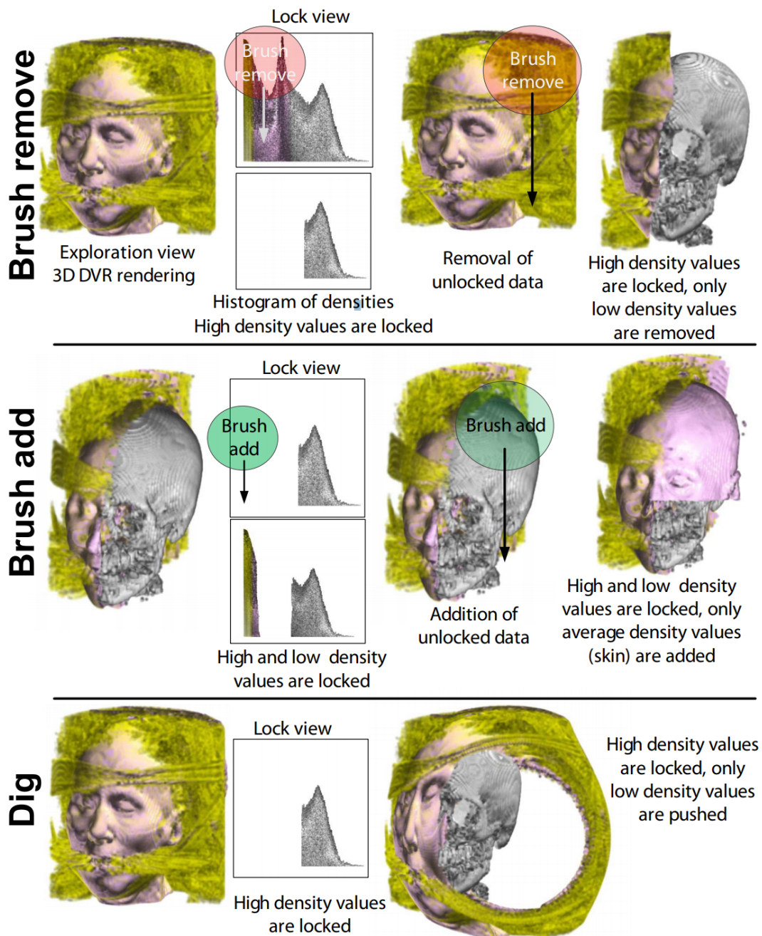
FIGURE 2.14: Brush, dig, and lock tools. Locked items are not affected by brush and dig. We used transfer functions to make air voxels transparent and standard gradient shading. We see that the head is surrounded by a large amount of uninteresting noise (yellow).
