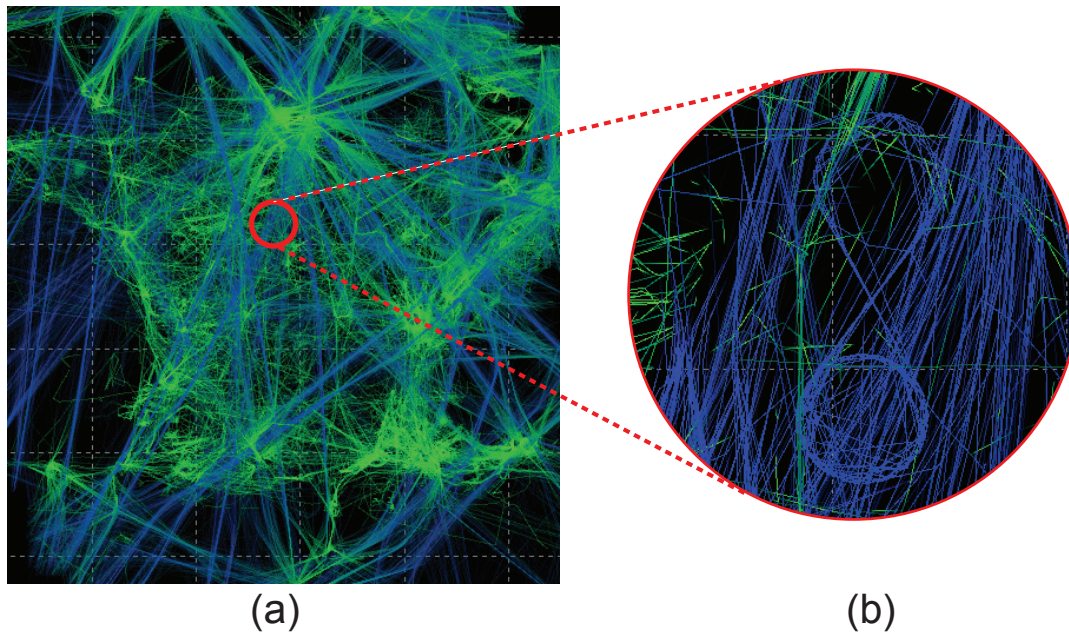
FIGURE 4.19: Visualizing one day of aircraft trajectories over France Hurter, Tissoires, and Conversy, 2009. (a) Overview of all trails. (b) Zoom, filtering, and color mapping techniques are used to highlight an outlier trajectory of an aircraft performing an eight-shaped loop. Revealing this outlier costs significant user effort.
