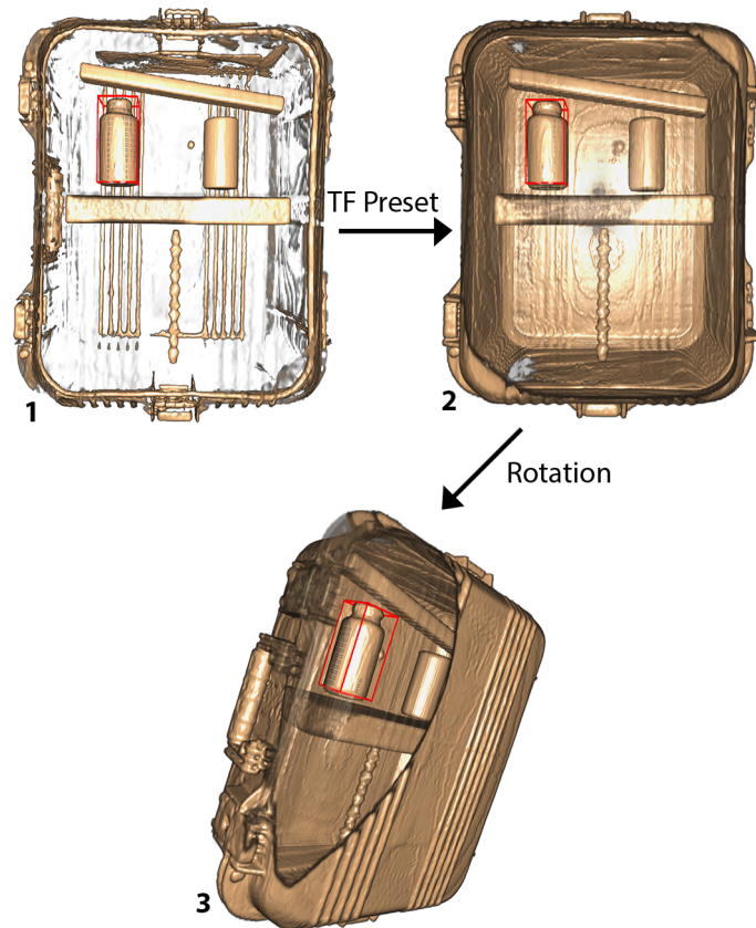
FIGURE 3.28: Inspection of an object from different perspectives. 1- The user defines an object of interest for further inspection. This object is then inside a box with red borders. 2- The user modifies the transfer function to see the target in another context. 3- The user rotates the baggage to look at the menace from a different perspective. It stays visible whatever the manipulation carried out.
