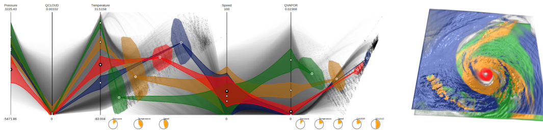
FIGURE 2.8: Parallel coordinates with embedded multidimensional scale plots for editing multidimensional TFs(Guo, Xiao, and Yuan, 2011)
