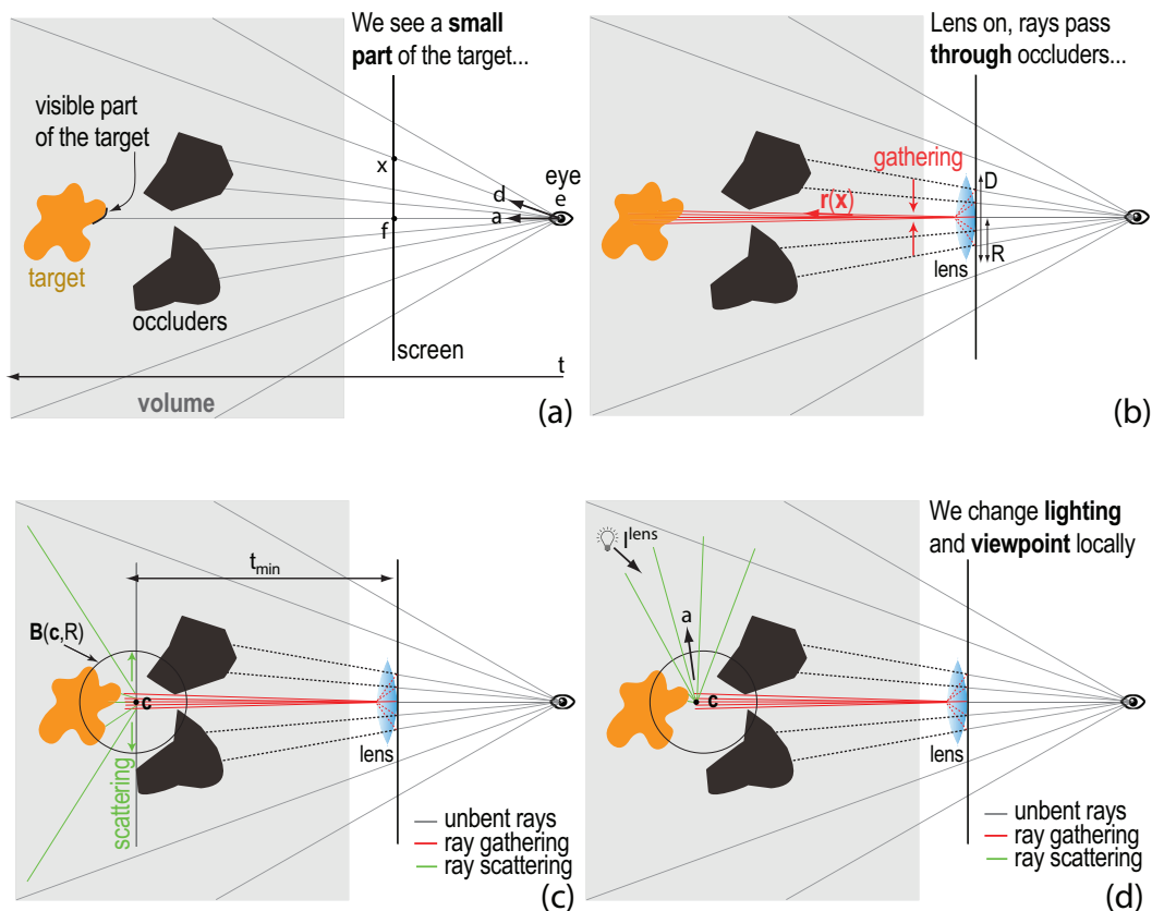
FIGURE 4.3: Obstruction-free lens working. A target is (mostly) hidden by occluders in front of it. (a) Classic DVR shows a small part of the target. (b) Our lens gathers rays to avoid occluders (subsection 4.4.1). Once close to the target, rays follow again their initial paths. Yet, only a small part of the target is visible. (c) Scattering rays makes the full target visible (subsection 4.4.2). Finally, we adjust the local viewing and lighting directions \mathbf{a} , \mathbf{l}^{lens} (subsection 4.4.3).
