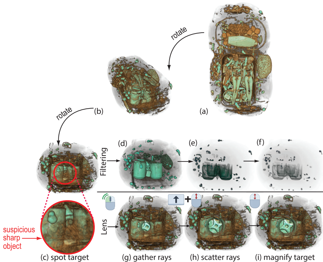
FIGURE 4.7: (a-c) A baggage scan is viewed from different angles. In view (c), a suspicious sharp object is spotted between a set of mugs. (d-f) Filtering densities using a classical 1D opacity transfer function removes progressively more of the occluders (mugs), but also the target. (g) The user applies the lens on the target object (double-click). An animation starts opening the lens, rays are gathered to pass through occluders. Halfway the animation, the object is magnified, but only the area close to the lens is visible. (h) The fish-eye field of view at the end of the animation scatters rays to fully show the target. (i) The lens is increased to magnify the target (mouse scroll).
