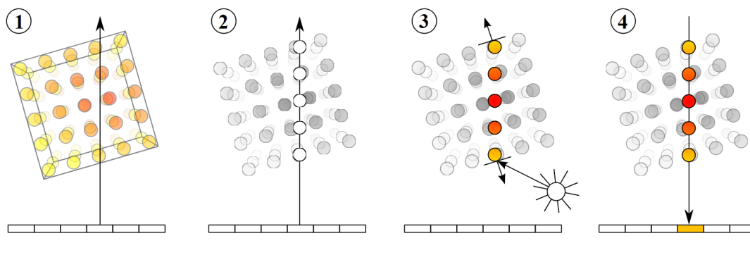
FIGURE 2.5: The four steps of the volume raycasting algorithm
