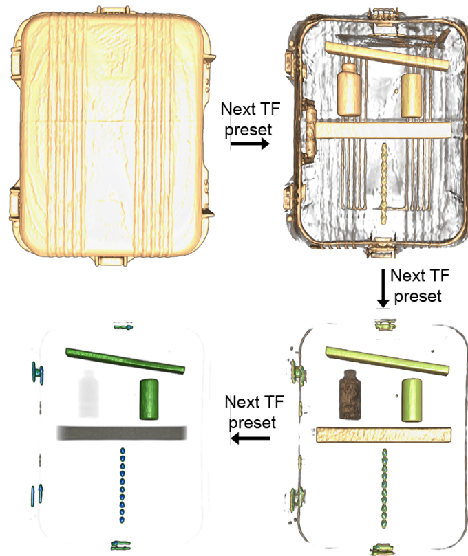
FIGURE 3.27: The transfer function presets help the user perceive the different types of material inside the baggage
