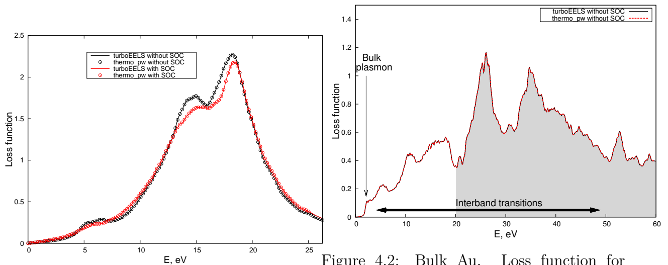
Figure 4.1: Bulk Bi. Loss function for a transferred momentum \mathbf{q} = 0.013 \text{ \AA}^{-1} in the z -direction obtained using: turboEELS code without and with spin-orbit coupling (SOC), and thermo_pw code without and with SOC.
