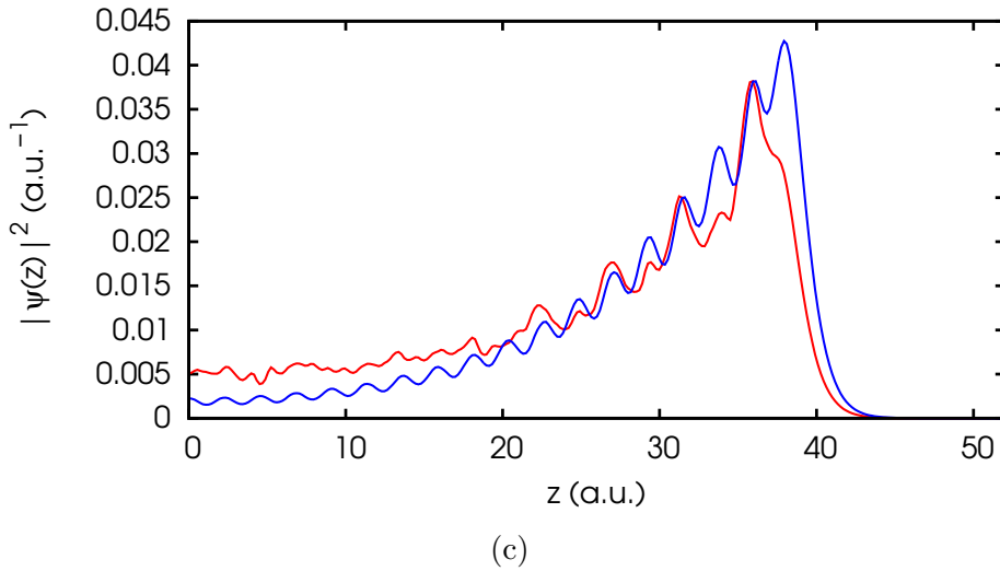
Figure 5.14: (continued) Planar averages of the surface states of Au(788) at (a) the bottom of the first subband at the \bar{Y} point, (b) the top of the first subband at the \bar{\Gamma} point and (c) the top of the second subband at the \bar{Y} point. Different colors correspond to wavefunctions with different eigenvalues identified as surface resonances at the same \mathbf{k} -point.
