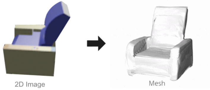
(a) Single-view shape reconstruction: Given an input image, our approach presented in Chapter 3 creates a parametric 3D polygonal mesh. Note how the unseen parts are correctly hallucinated.
