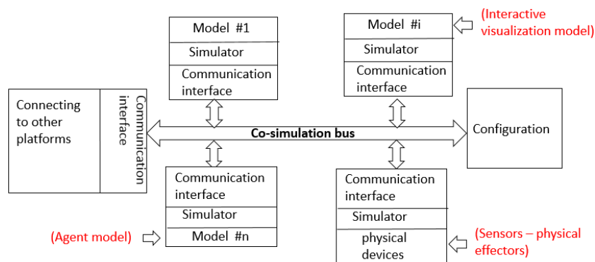
Figure 25: Example of a distributed co-simulation platform
