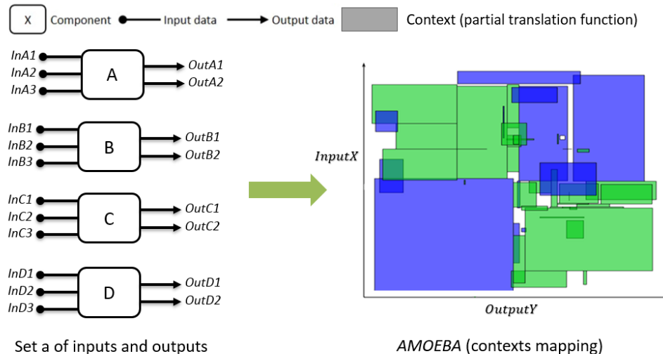
Figure 43: AMOEBA learns the data combinations
