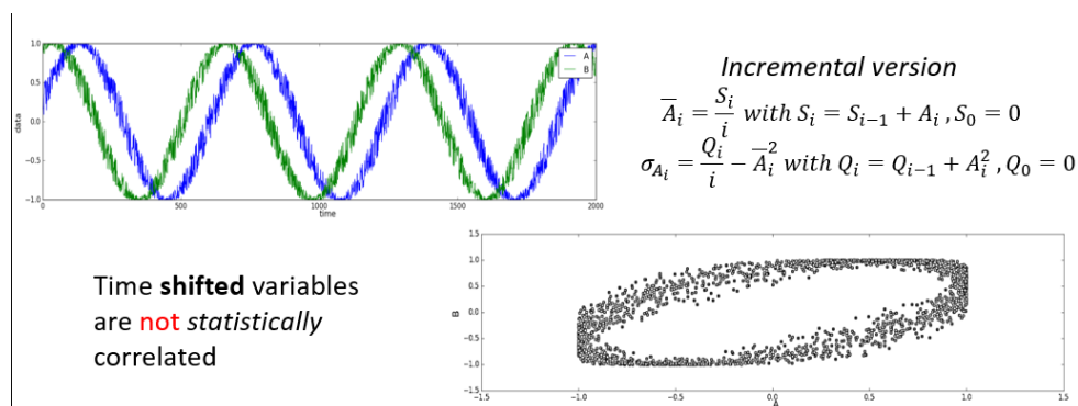
Figure 35: Pearson's correlation plot
