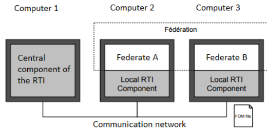
Figure 10: High level view, logic of a HLA Federation execution [Zacharewicz, 2006]
