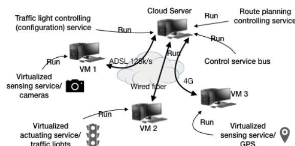
Figure 4.32 – Emergency car leading control prototype
