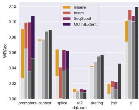
Figure 4.22: Added value of local optima search for 1,000 iterations
