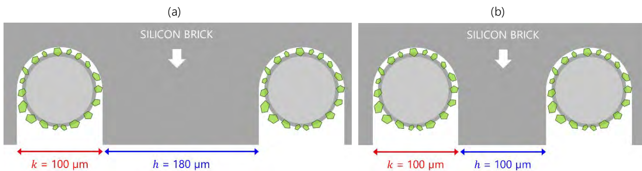
Figure 4.2. Schematic illustration of kerf versus wafer thickness when cutting a silicon brick with a wire of core diameter 80 \mu\text{m} (a) Nominal thickness 180 \mu\text{m} (b) Nominal thickness 100 \mu\text{m}
