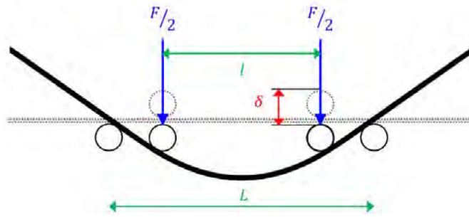
Figure 2.23. Important dimensions and measured data of the 4-line bending setup
