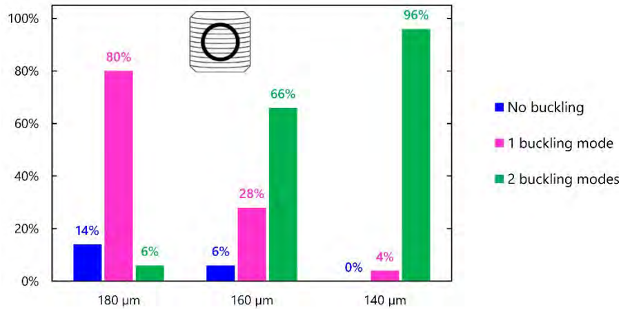
Figure 4.18. Percentage of monocristalline wafers of different thicknesses having experienced zero, one or two buckling modes before failure when tested with RoR setup
