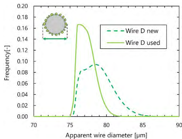
Figure 4.25. Histograms of apparent diameter of wire D before and after cutting
