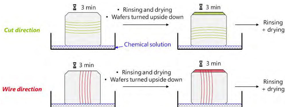
Figure 3.27. Chemical etching procedure implemented to etch only the edges of the wafers
