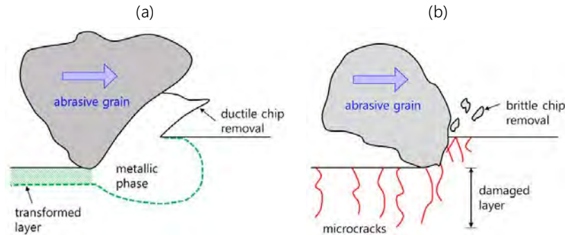
Figure 1.13. Schemes of cutting brittle materials in (a) ductile mode and (b) brittle fracture, from [158]
