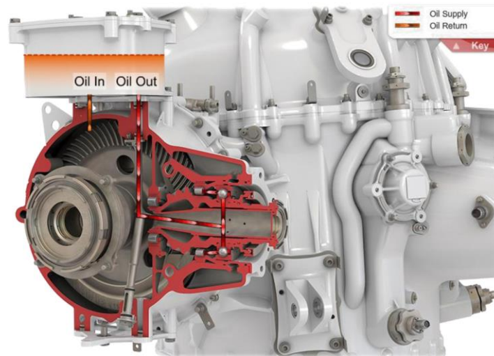
Figure I.2: Cross-sectioned view of a Helicopter gear box cooling system [22]
