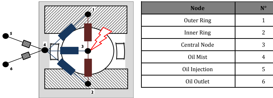
Figure 3.3 : 4 Nodes REB Thermal Network Scheme
