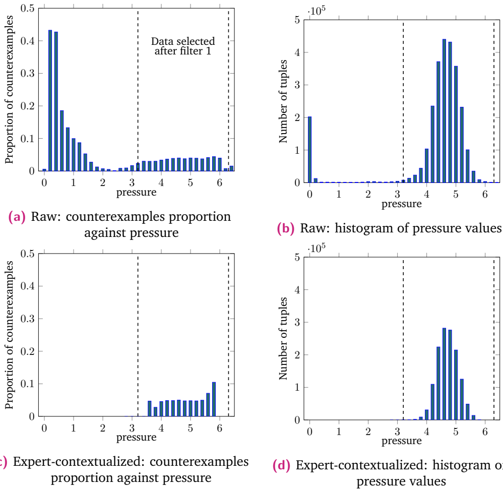
Fig. 5.13: Counterexamples and distribution for pressure values
