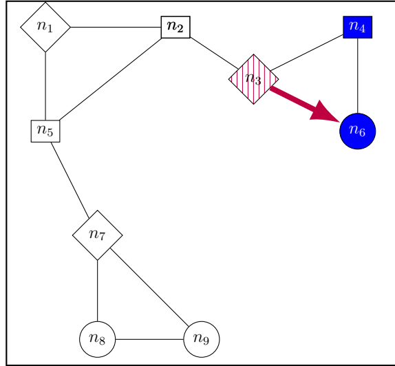
(b) t_6 : handleAlloc() , n_3 receives Req_3 after it has sent an ALLOC message for Req_2 . It enters the PREEMPTING state and sends a PREEMPT message to n_6 .
