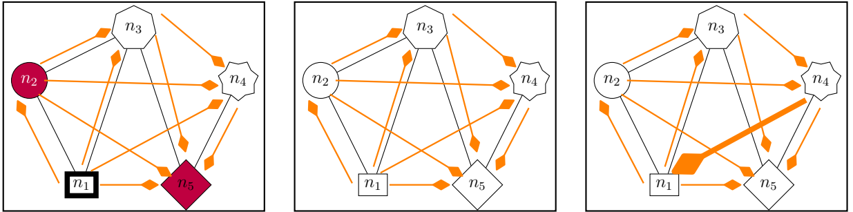
(a) t_1 : initial stage, n_1 can enter CS for Req_A (b) t_2 : n_1 releases its CS, n_4 requests fork from n_1 (c) t_3 : n_4 gets fork from n_1
