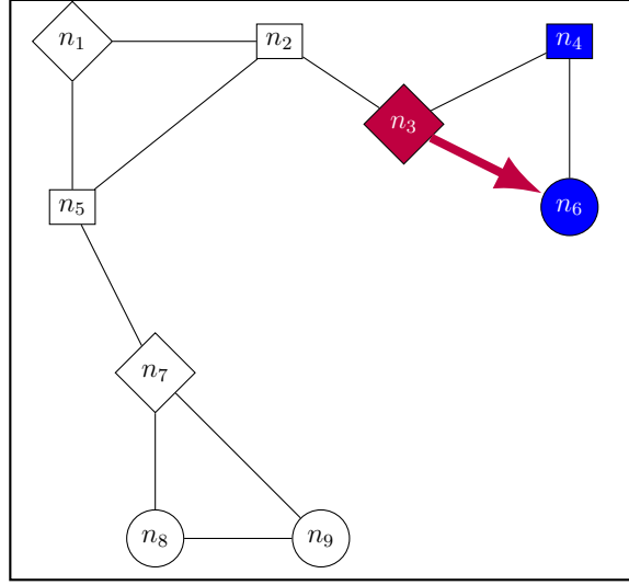
(b) t_4 : allocation of Req_2 continues. n_3 sends an ALLOC message to n_6 .
