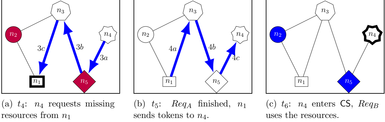
Figure 6.26: Sample execution of Bouabdallah-Laforest algorithm 2/2
