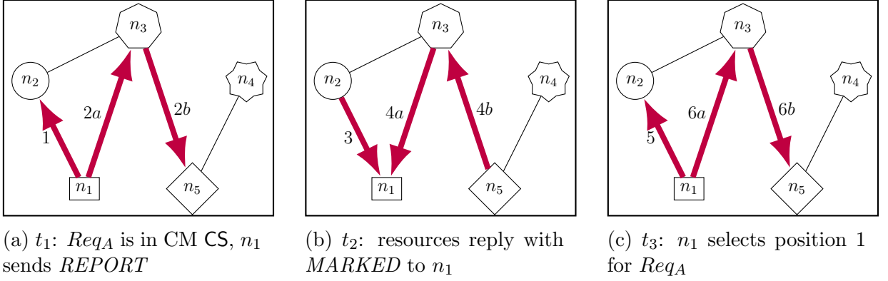
Figure 6.13: Sample execution of Rhee's algorithm 1/4
