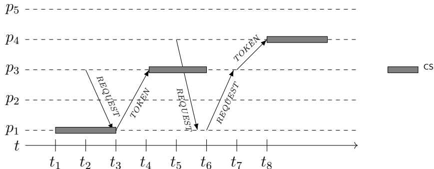
Figure 6.18: Timeline of sample execution of Naimi-Tréhel algorithm
