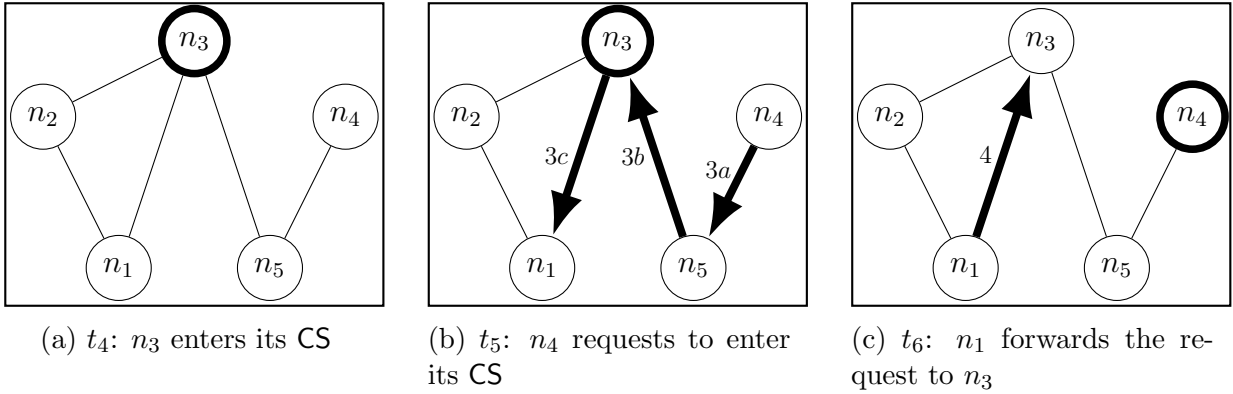
Figure 6.20: Sample execution of Naimi-Tréhel algorithm 2/3
