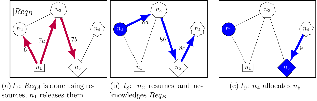
Figure 6.5: Sample execution of Dijkstra's Incremental algorithm 3/4
