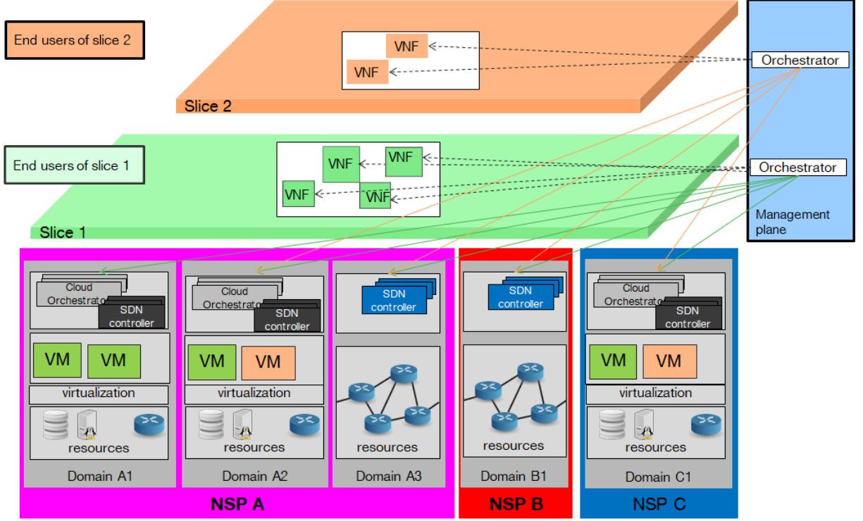
Figure 2.5: Architecture of multi-domain network slices
