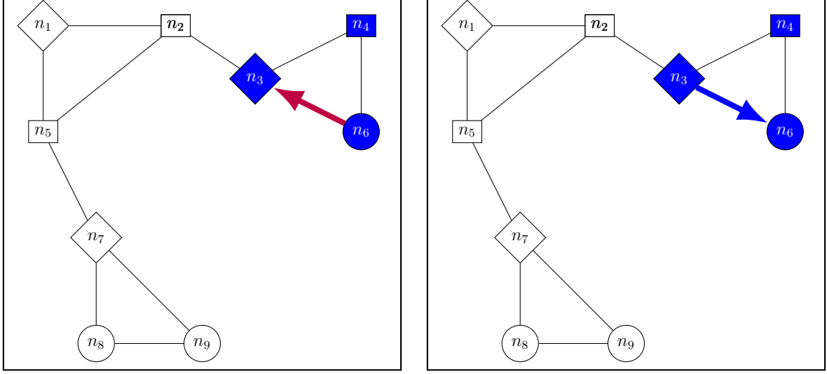
(a) t_7 : handleAlloc() , n_6 sends a PRE-EMPT message. Upon reception n_6 comes ALLOCATED for Req_3 . (b) t_8 : handleAlloc() , Req_3 ends. n_3 sends an ALLOC_ACK message to the requesting node n_6 .
