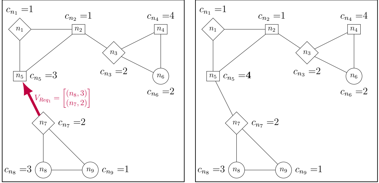
(a) t_5 : handleRouting() , a ROUTING message is sent to n_5
