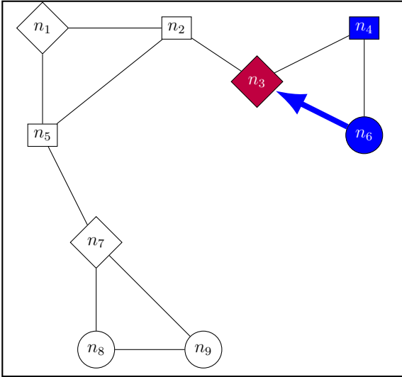
(a) t_5 : handleAlloc() , allocation of Req_3 continues. n_6 sends an ALLOC message to n_3 .
