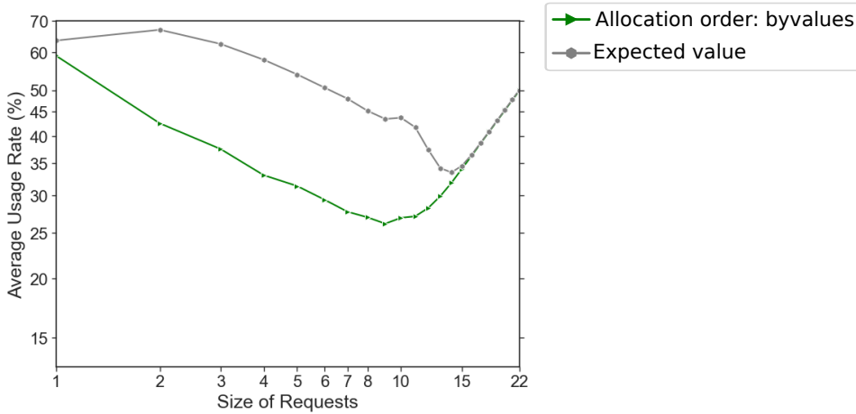
Figure 5.9: Comparison with expected value of the Average Usage Rate in a system with one instance of 44 types of resources
