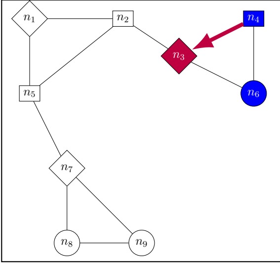
(a) t_3 : allocate() , allocation of Req_2 starts. n_4 sends an ALLOC message to n_3 .
