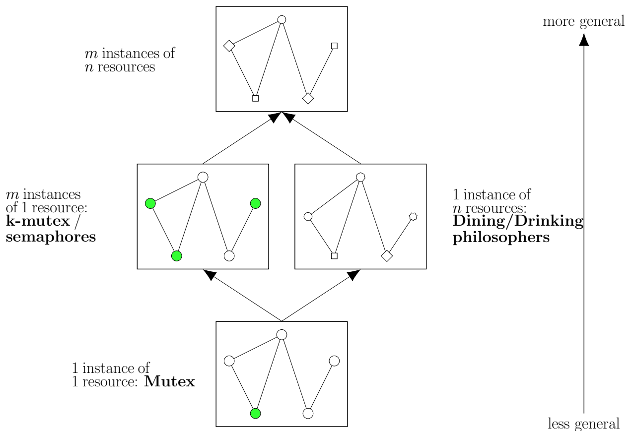
Figure 3.7: Classification of problems for the distributed allocation of resources
