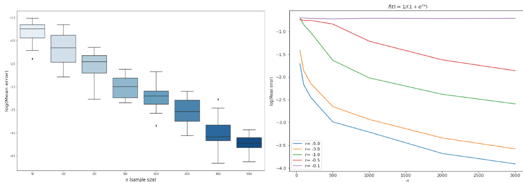
Figure 4.10: In the left a boxplot for \log(ME_n) , for different values of the sample size in threhsold graphon with d = 3 , \tau = 0.1 and F_{1/2} . In the right we plot the mean error for the logistic graphon with different values of the parameter r .
