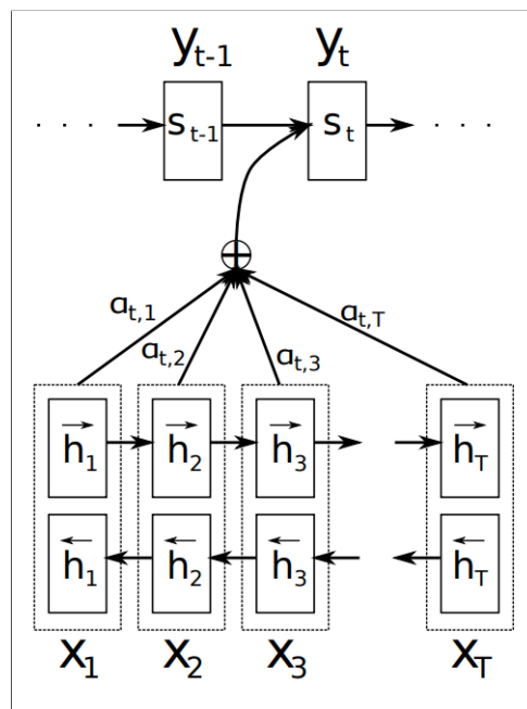
Figure 2.18 – Example of the Attention mechanism taken from [5].
