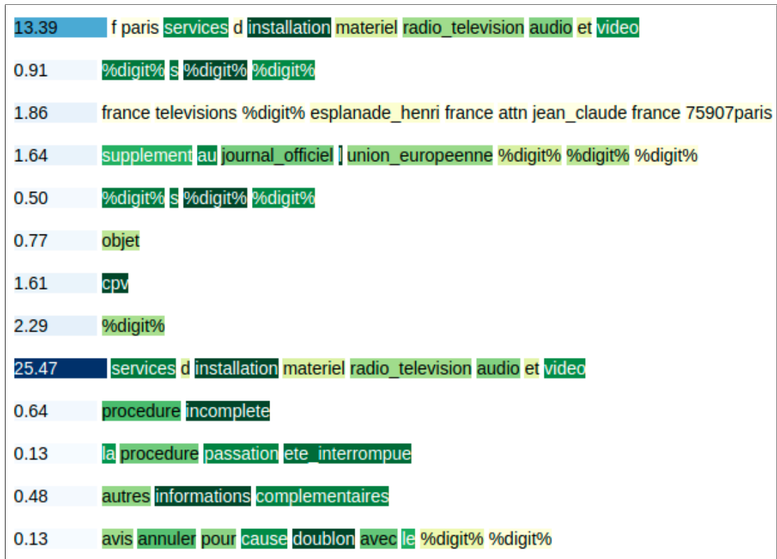
Figure 2.29 – Figure illustrating attention weights in a sentence and a word level on a FULL-TED document in the class "Installation services of communications equipment"
