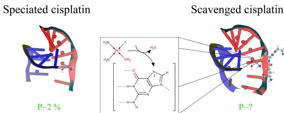
Figure V-2. cDDP-nDNA main crosslinks, their relative proportions P and a representation of the chemical structure of guanine exhibiting the atom N7 of the imidazole ring of a guanine being attacked by a monoaquacisplatin [65, 130, 132]. In the case of monoadducts, the distinction is present in between speciated cisplatin in the medium and cisplatin bound to any nucleophile present in the environment (on the scheme, a glutathione molecule is represented). The two strands of DNA are represented in blue and red ribbons, the N7 atoms of the guanines are represented as large blue or red spheres.
