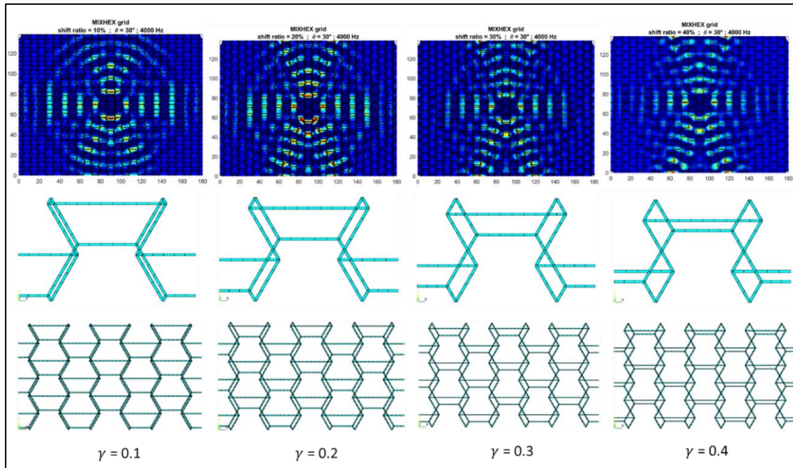
Figure 91 - Propagation of a monochromatic wave set at 4000 Hz for the MixHex cellular grid as the shift ratio is varied from \gamma = 0.1 to \gamma = 0.4 . The shift ratio is limited to 0.4 to avoid structures compenetrating.
