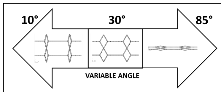
Figure 72 - HEXHEX unit cells according to internal angle variation
