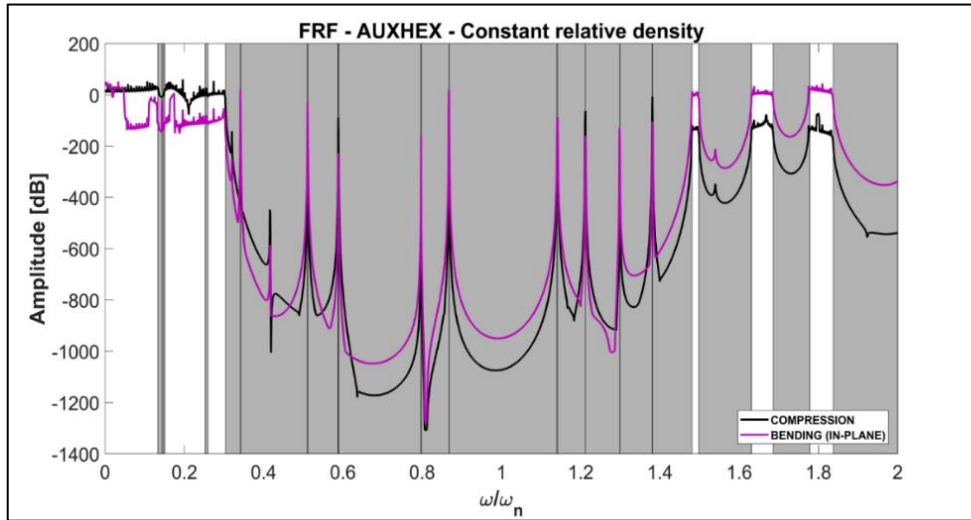
Figure 50 - In plane FRF for pressure wave (black) and in-plane bending (magenta) for the AuxHex pattern
