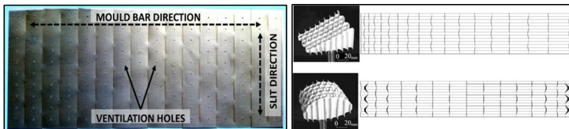
Figure 6 - Detail of honeycomb ventilation holes performed as a pre-process thanks to kirigami (left) Variable thickness honeycombs and their cutting patterns proposed by Nojima, Saito and Pellegrino[18] (right)
