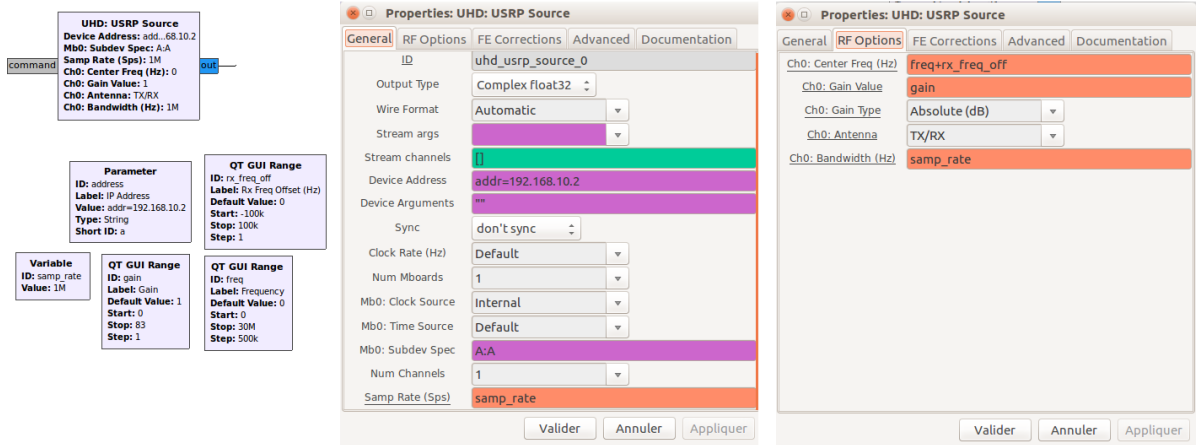
Figure V-10 : UHD Source
