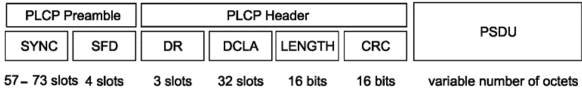
Figure IV-9 : Structure PPDU [136]
