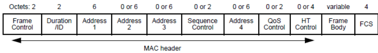
Figure IV-8 : Structure MPDU [46] [136]
