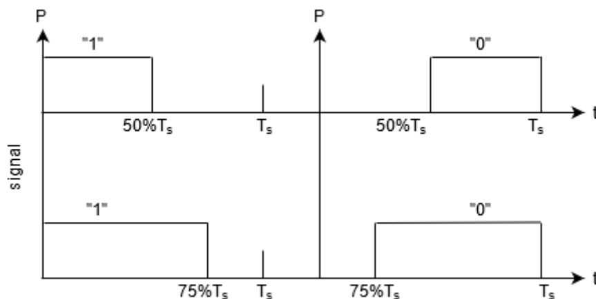
Figure II-8: Illustration de la modulation V-PPM
