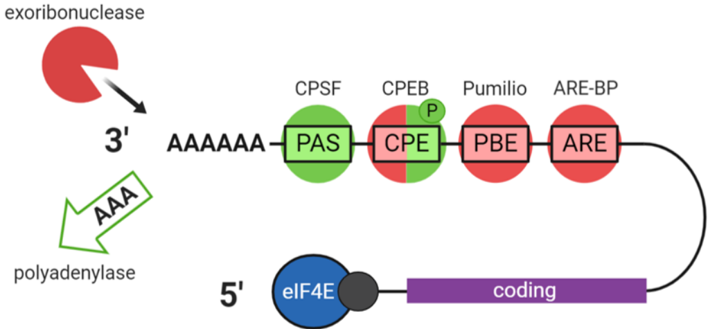
Figure 21. Key 3'UTR elements, their associated RBPs and control of poly(A) tail length. 3'UTR elements and RBPs mediating polyadenylation and translation activation are shown in green and those mediating deadenylation and translational repression in red. PAS: polyadenylation signal, CPSF: cleavage and polyadenylation specificity factor, CPE: cytoplasmic polyadenylation element, CPEB (CPEB1): CPE-binding protein, PBE: Pumilio-binding element, ARE: AU-rich element, ARE-BP: ARE-binding protein. Source: Own work (created with BioRender)
