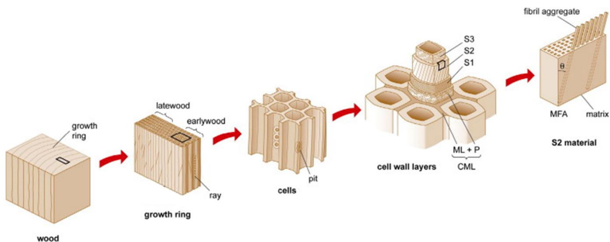
Figure 6. Hierarchical structure of wood. Adapted from [38]. ML: middle lamella; P: primary wall; S: secondary wall (with its sub-layers: S1, S2 and S3); CML: compound middle lamella; MFA: microfibril angle.
