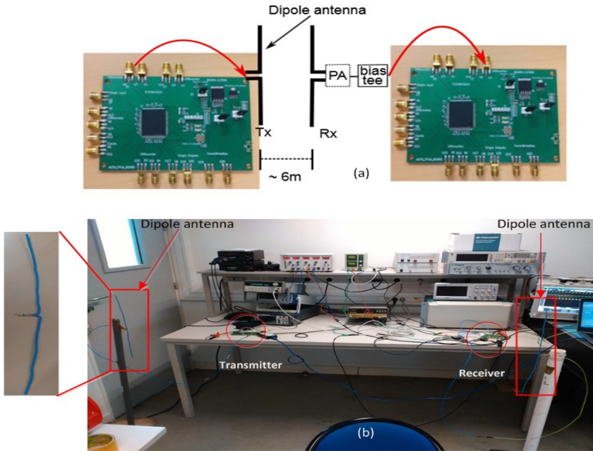
Fig. 6.18: Measurement setups. (a) Measurement setup used in transmission of wireless data between two FPGAs using customized dipole antenna. After the antenna on the Rx side, we have the option to use PA. (b) Actual measurement setup used in experimentation in real environment. (Inset) the half wave dipole antenna developed in-house for bandwidth of around 240 MHz.
