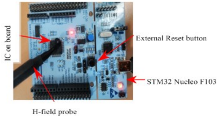
Fig. 3.13: Measurement steps for STM32 \mu C: Localized EM probe horizontally placed over the IC of \mu C board.
