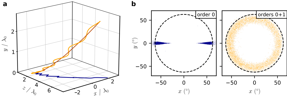
Figure 4.3: Electron dynamics in Gaussian beam with and without first-order corrections - On panel (a), three electron trajectories are plotted in the 3D-space (x, y, z) : (i) in blue, with only considering zeroth-order fields, (ii): in orange, with fields corrected up to the first order and (iii) in brown, with ponderomotive force only (Eq. (4.8)). On panel (b) are plotted the final angular distributions without (blue) and with (orange) first-order field corrections. The black dashed circle just helps the reader for direct comparison between the two plots.
