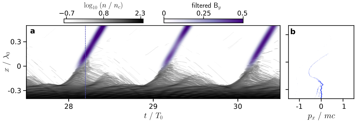
Figure 3.8: Temporal dynamics of the plasma mirror using a plane detector in the plasma surface - In panel (a), spatio-temporal plasma evolutions (in gray log color scale) are recorded on \mathcal{P}_1 (see Fig. 3.7-a) as well as the attosecond light pulses emitted during the interaction (harmonics 10-20). Panel (b) shows the electron distribution during the ejection in the (x, p_x) phase space at a time t = 28.2 T_0 (blue dashed line). All physical and numerical parameters are kept the same as in Fig. 3.7.
