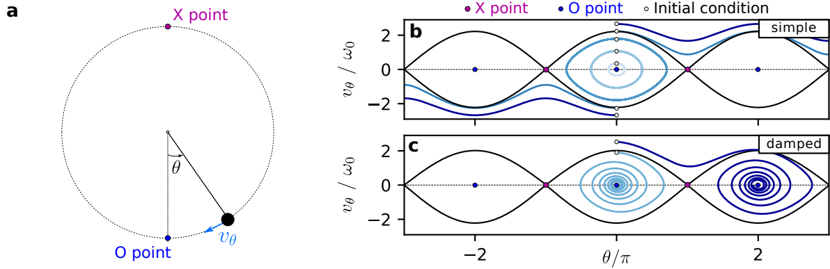
Figure 2.5: Trajectories in phase space for a simple pendulum - Panel (a) sketches a simple pendulum and highlights two positions of interest: the unstable X point and the stable O point. On panels (b) and (c) are plotted different trajectories in phase space, solutions of Eq. (2.4): (b) \nu = 0 and (c) \nu = 0.1 . Each trajectory starts from a different initial state (displayed as white circles), which corresponds to \theta(t) = 0 and v_\theta(0) = v_0 from 0.3 to 2.5 \omega_0 . The O and X points are also pictured in this space.
