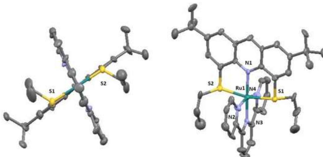
Figure 4.6. Different views of the crystal structure of the heteroleptic complex 19 (40% ellipsoids). Solvent molecules, H-atoms, and \text{PF}_6^- counter anions are omitted for clarity.
