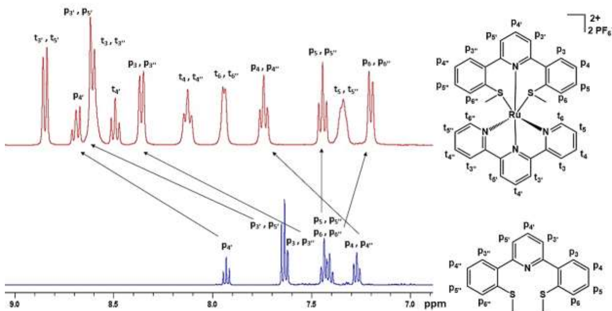
Figure 5.14. 1 H-NMR spectra of ligand 20 (bottom) and its heteroleptic Ru(II) complex 22 (top), recorded in D 6 -acetone on a 500 MHz NMR spectrometry.
