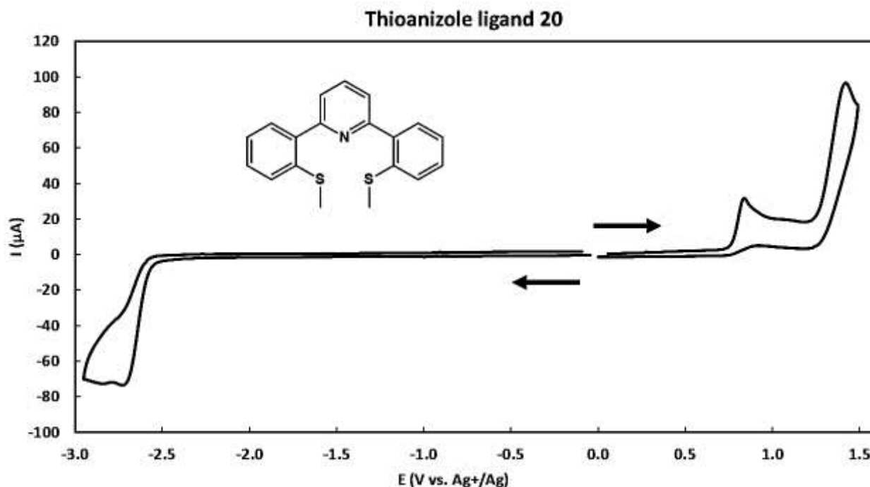
Figure 5.16. Cyclic voltammogram of the thioanisole ligand 20 ( 10^{-3} M) in deaerated acetonitrile solution containing 0.1 M of \text{TBAPF}_6 , at a scan rate of 100 \text{ mV.s}^{-1} using vitreous carbon working electrode (5 mm diameter), E_p(\text{V}) vs \text{AgNO}_3 (0.01 M)/Ag.
