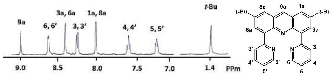
Figure 2.2. The dttdpa ligand proton assignment on its 1 H-NMR spectrum, recorded in D 2 O at 500 MHz NMR spectrometer.
