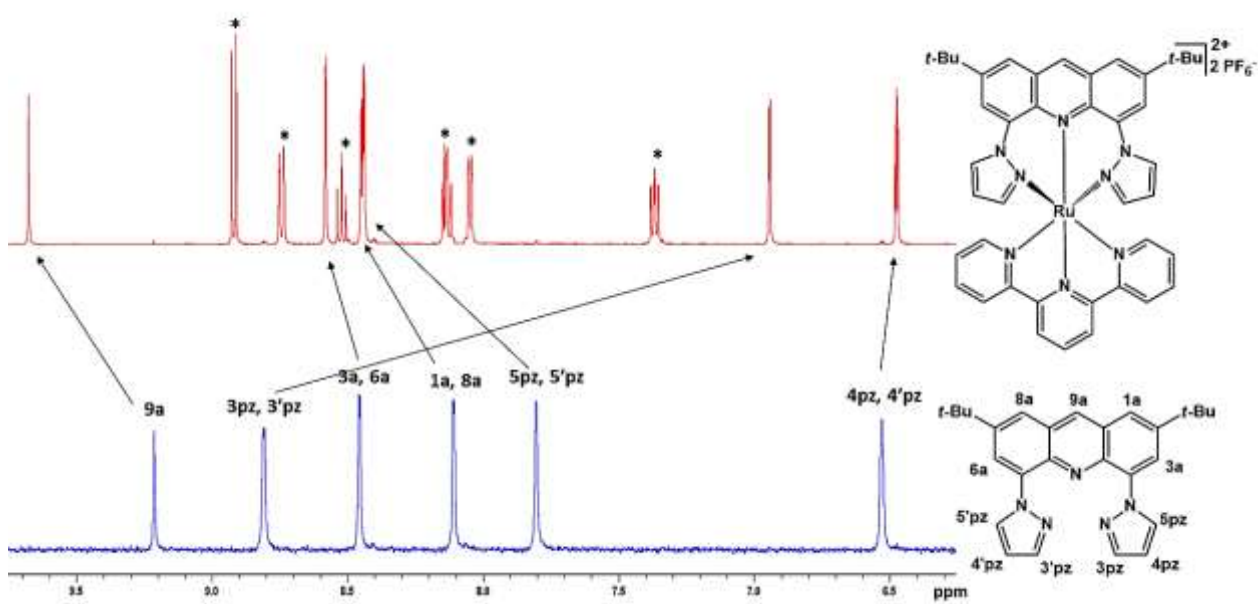
Figure 3.8. ^1\text{H} -NMR spectrum of both dtdpza ( 14 ) ligand (bottom) and its corresponding heteroleptic Ru(II) complex ( 16 ) (top), recorded in D-acetone at 500 MHz NMR spectrometer.
