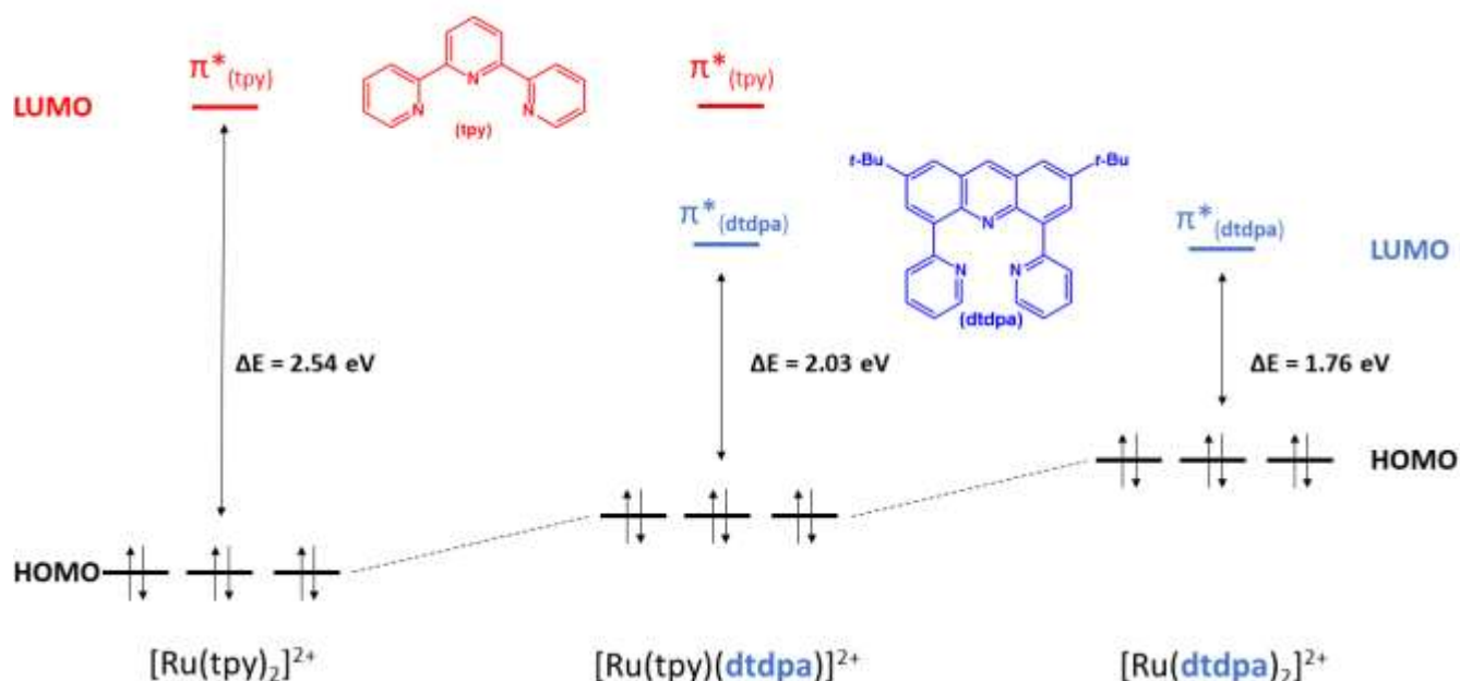
Figure 2.16. Relative molecular orbitals energy level for complexes 12 , 13 , and [Ru(tpy) 2 ] 2+ .
