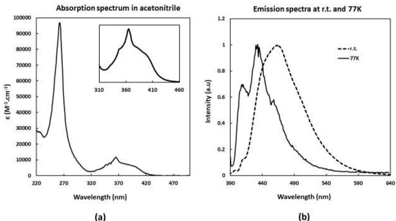
Figure 2.14. Absorption and emission spectra of dtbpa ligand.
