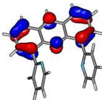
Figure 2.11. HOMO localization on dtdpa ligand, optimized by DFT calculations.
