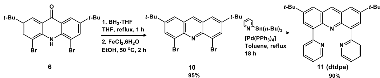
Scheme 2.5. dttdpa target ligand synthetic pathway.
