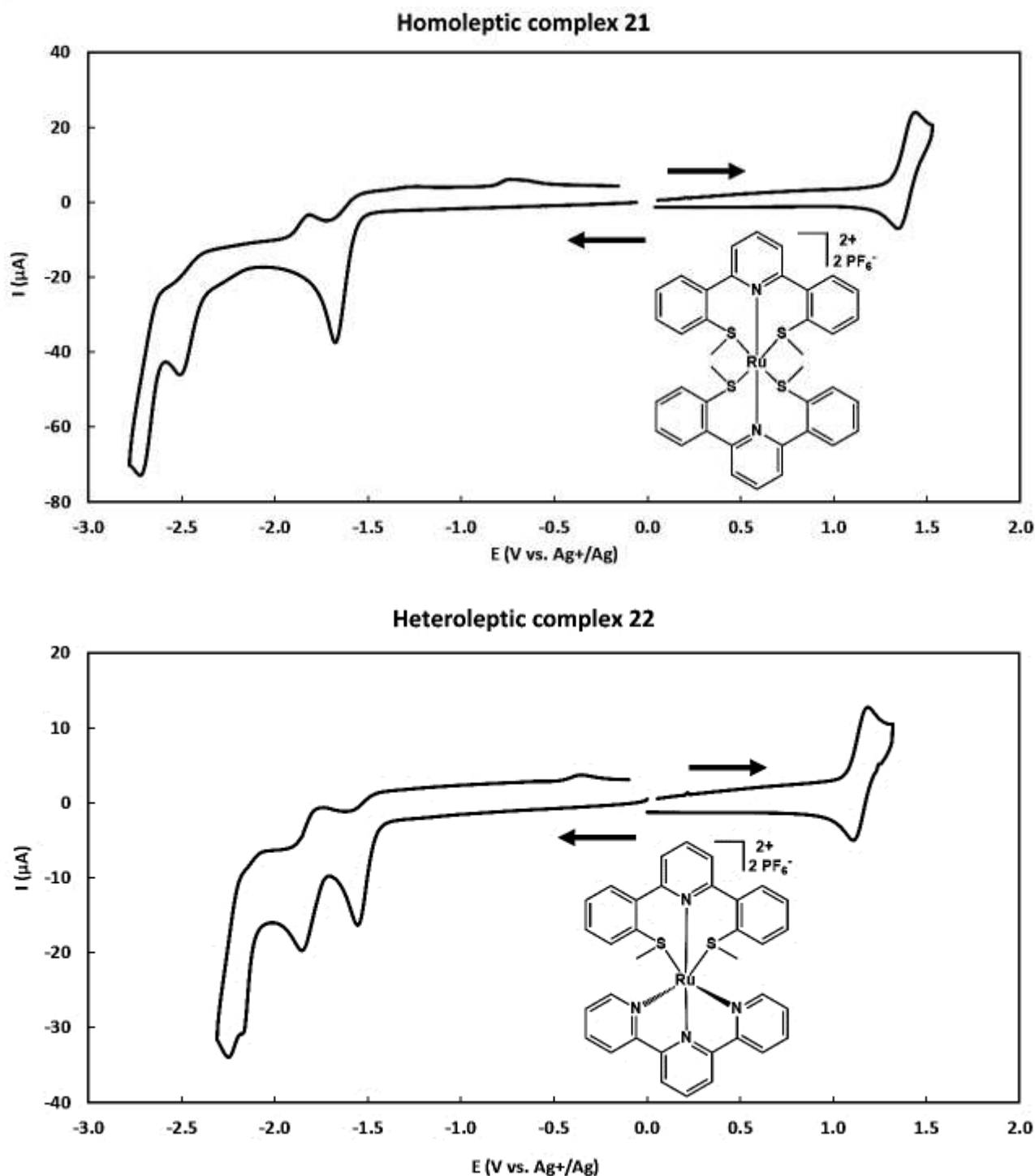
Figure 5.17. Cyclic voltammograms of the homoleptic complex 21 (top), and the heteroleptic complex 22 (bottom) at 10^{-3} M concentrations in deaerated acetonitrile solution with 0.1 M of \text{TBAPF}_6 , at a scan rate of 100 \text{ mV.s}^{-1} using vitreous carbon working electrode (5 mm diameter), E_p(\text{V}) vs \text{AgNO}_3 (0.01 M)/Ag.
