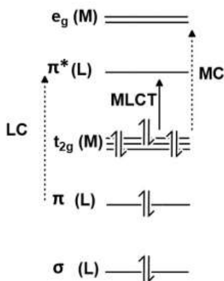
Figure 1.11. Schematic molecular orbital energy diagram for d^6 ruthenium(II) complex in an octahedral environment, showing by arrows the different types of transition.
