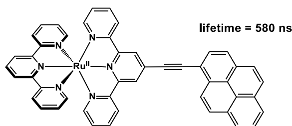
Figure 1.30. Pyrene-acetylene substituted on a [\text{Ru}(\text{tpy})_2]^{2+} complex.
