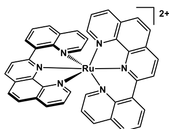
Figure 1.34. Second example for optimizing the octahedral geometry of bis-tridentate Ru(II) complexes.
