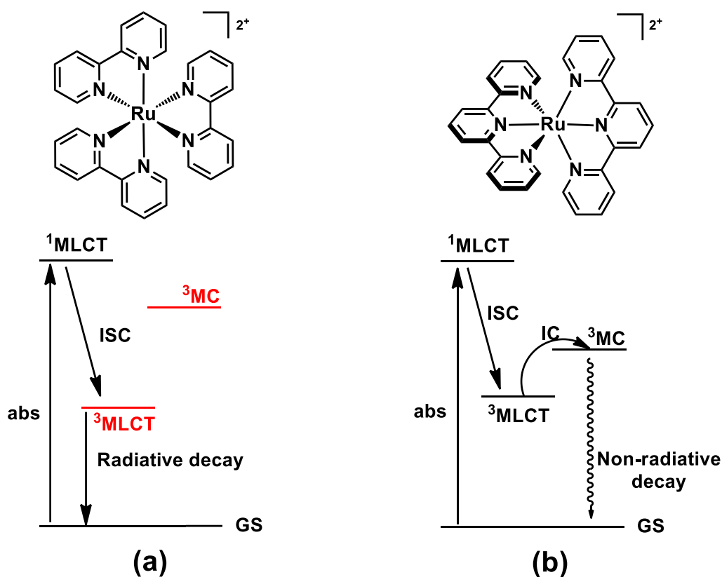
Figure 1.26. Perrin-Jablonski diagram for [\text{Ru}(\text{bpy})_3]^{2+} (a) vs [\text{Ru}(\text{tpy})_2]^{2+} (b).
