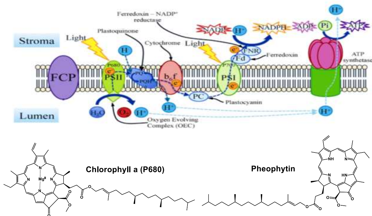
Figure 1.1. A representation of main steps in photosynthesis, showing the electron and proton flow through the thylakoids protein membrane of complexes PS II, Cyt b 6 f , and PS I, and production of ATP fuel by an electron and proton gradient across the protein membrane. 8
